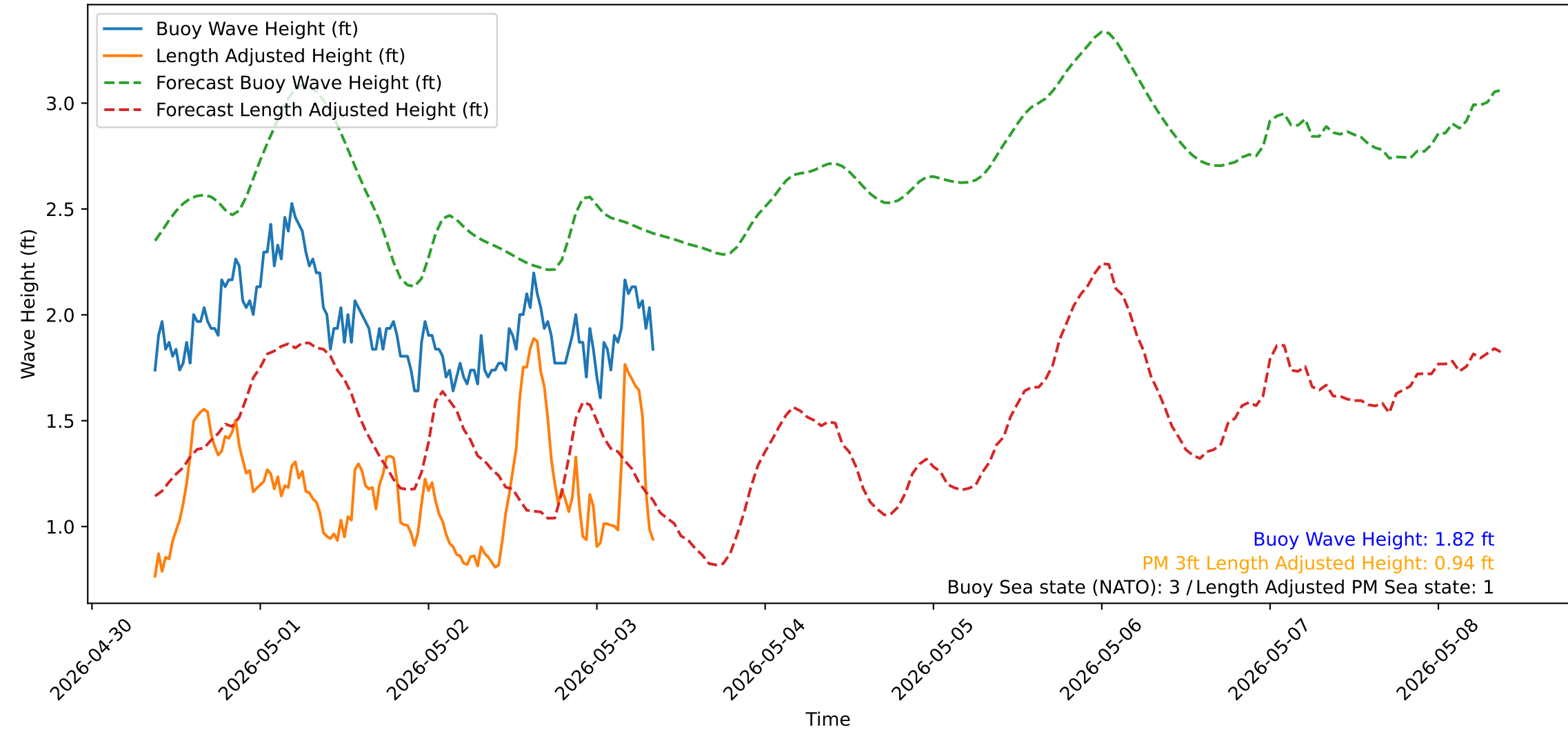
Wave Heights over Time for Red Beach at 2026-05-03 08:50:51
