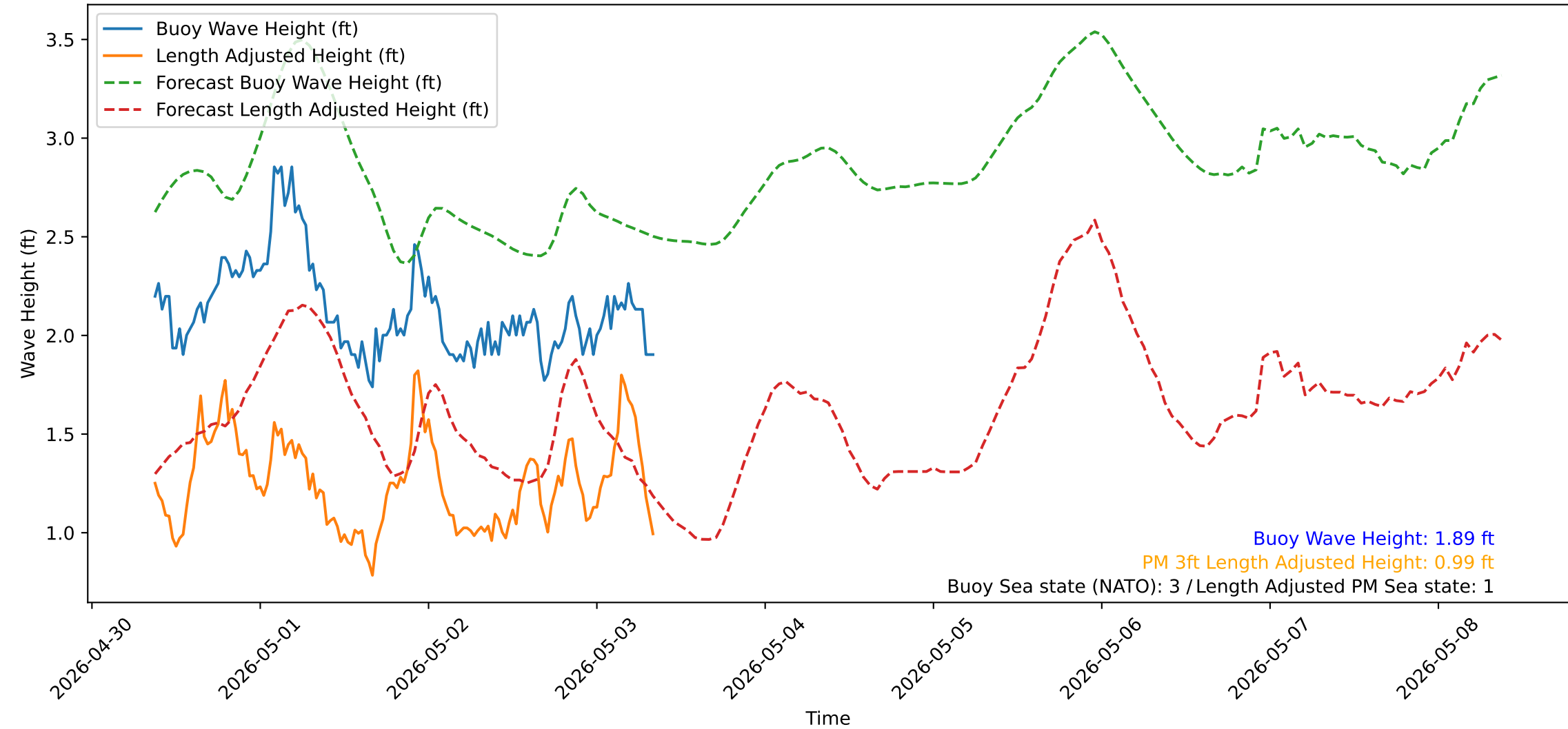
Wave Heights over Time for Green Beach at 2026-05-03 08:51:13
