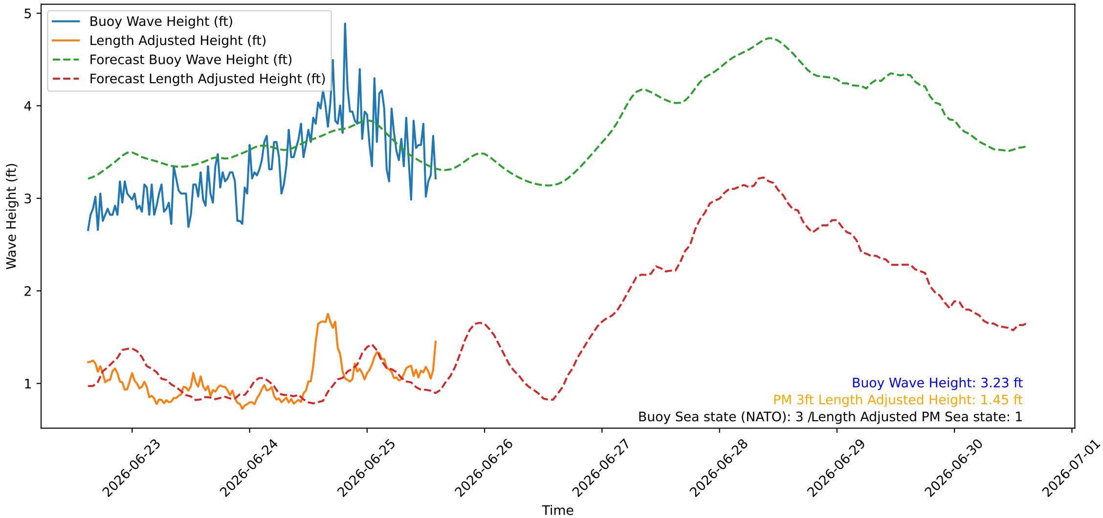
Wave Heights over Time for Oceanside Harbor at 2026-06-25 14:50:26
