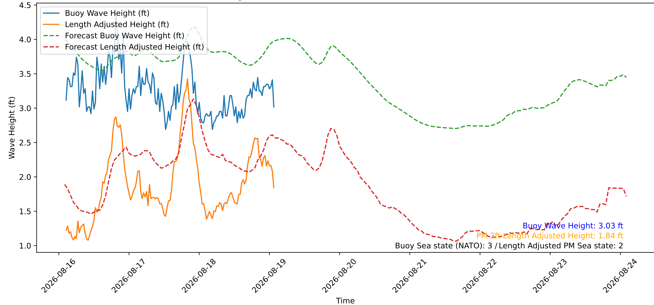
Wave Heights over Time for Green Beach at 2026-08-19 02:21:11
