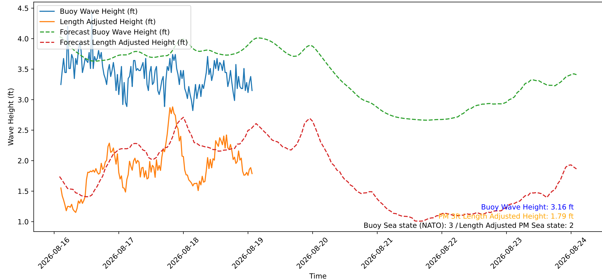
Wave Heights over Time for Oceanside Harbor at 2026-08-19 02:20:26
