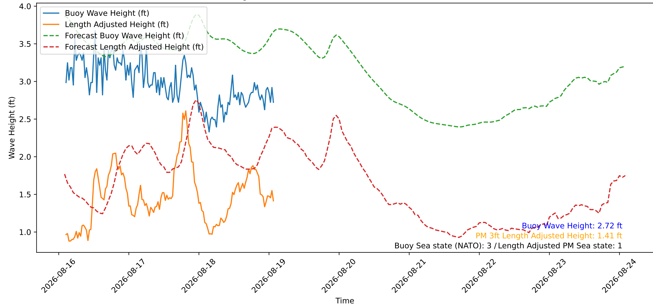
Wave Heights over Time for Red Beach at 2026-08-19 02:20:46
