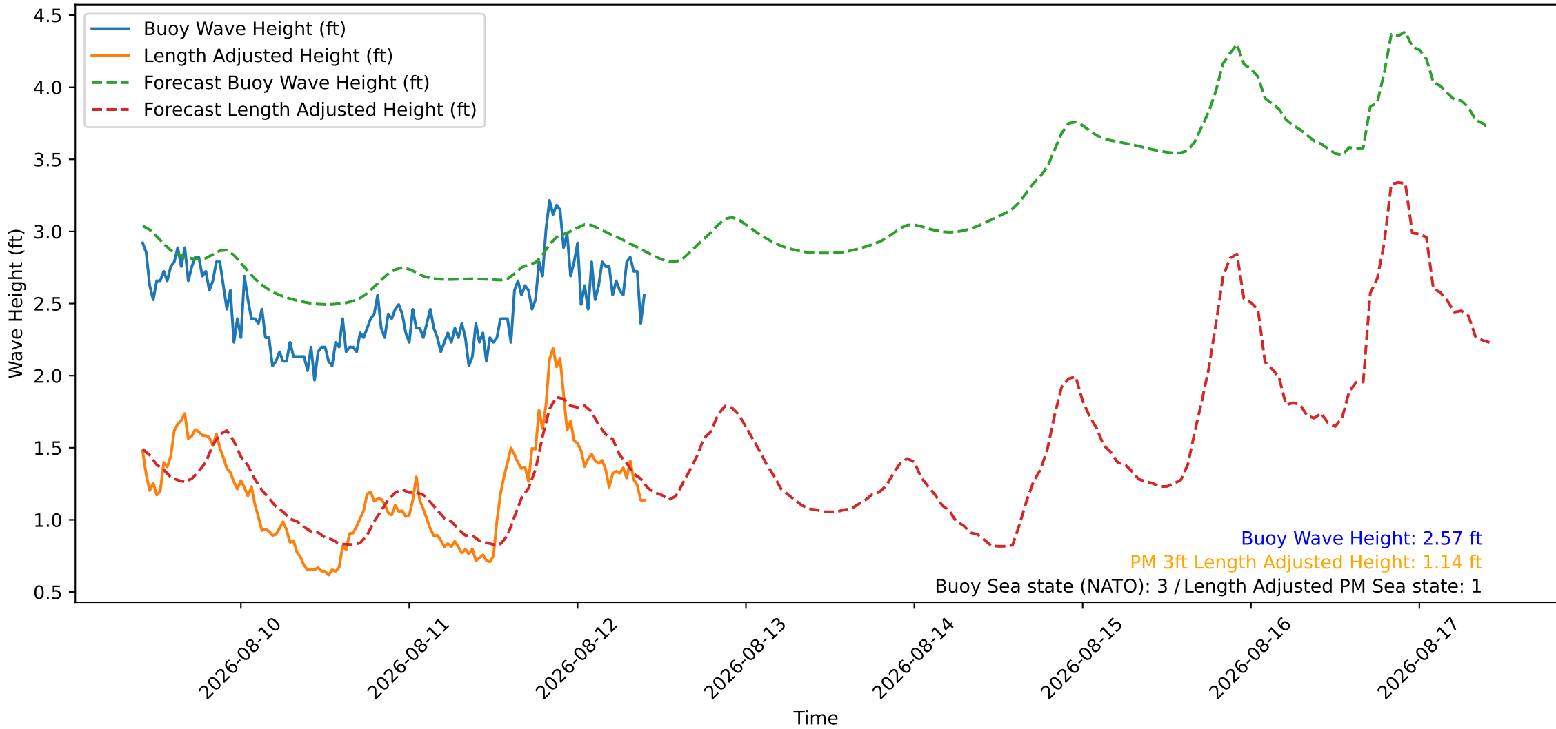
Wave Heights over Time for Green Beach at 2026-08-12 10:11:09
