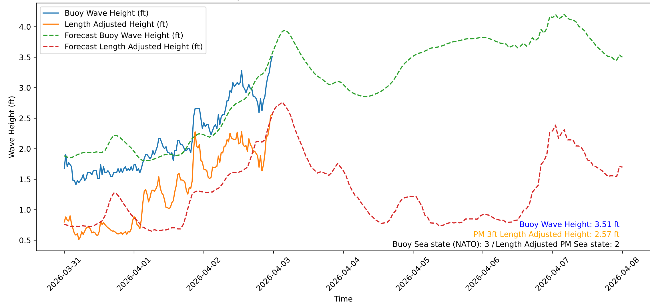
Wave Heights over Time for Green Beach at 2026-04-03 00:11:09
