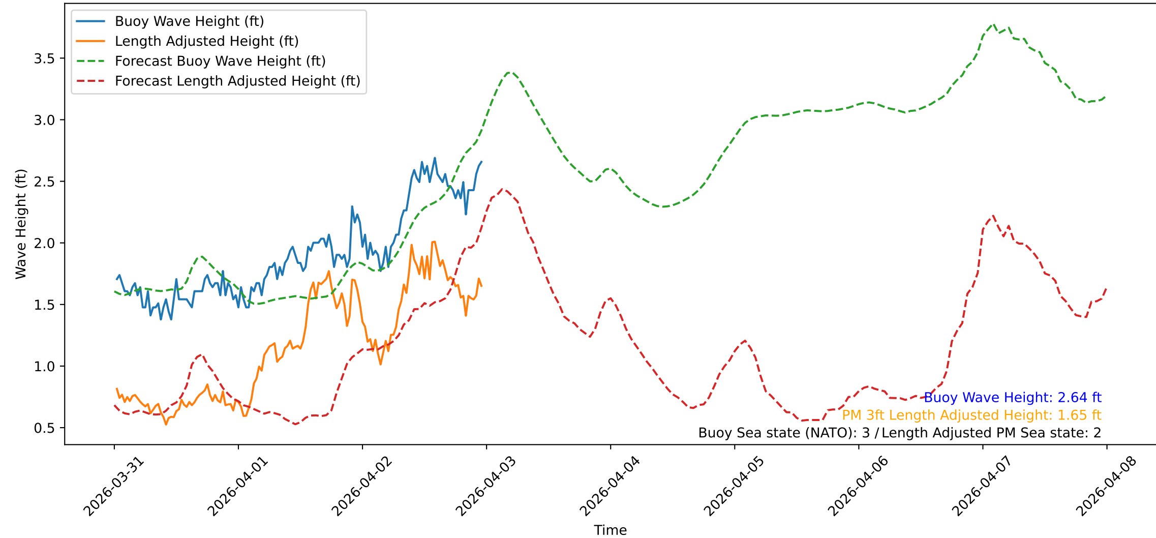
Wave Heights over Time for Red Beach at 2026-04-03 00:10:47
