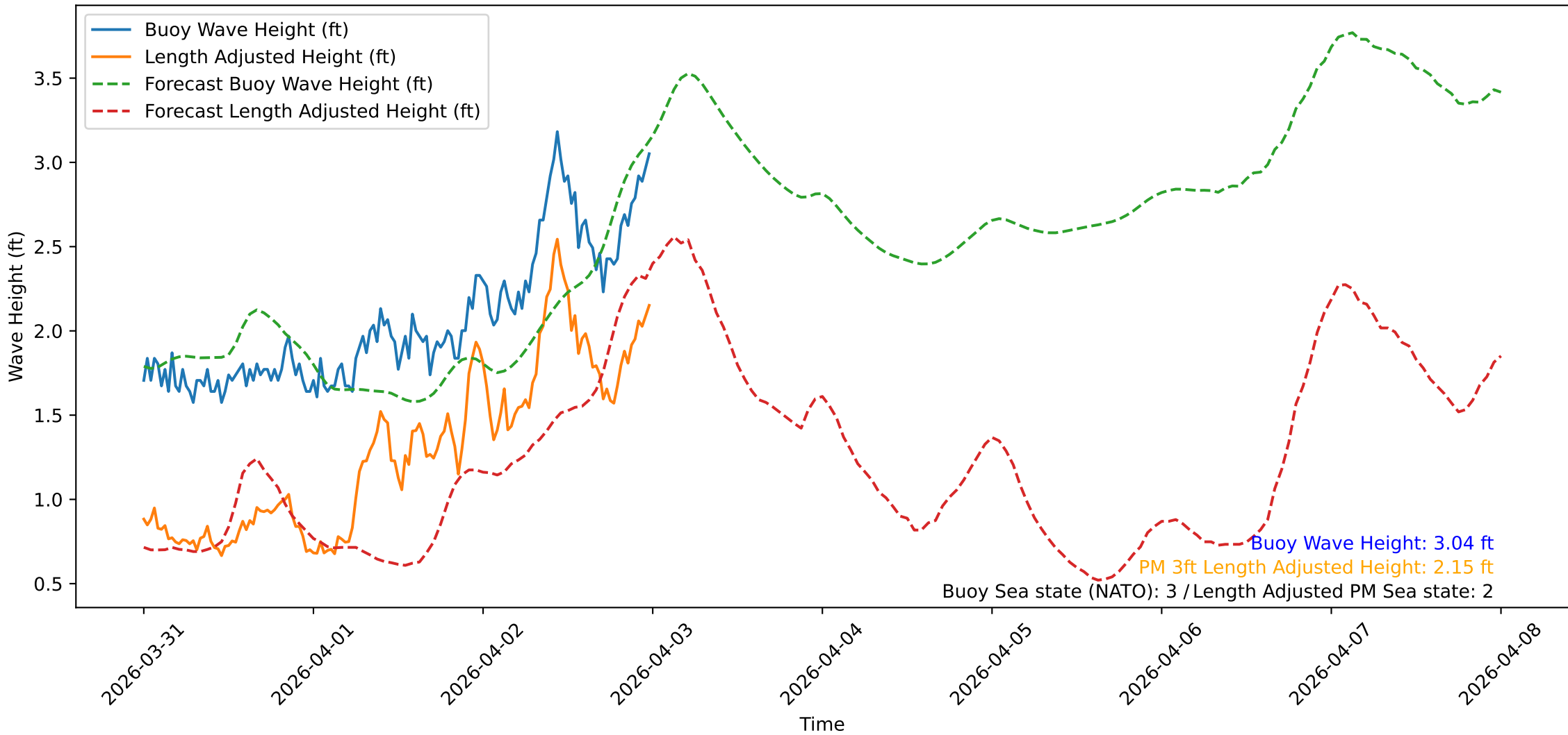
Wave Heights over Time for Oceanside Harbor at 2026-04-03 00:10:31
