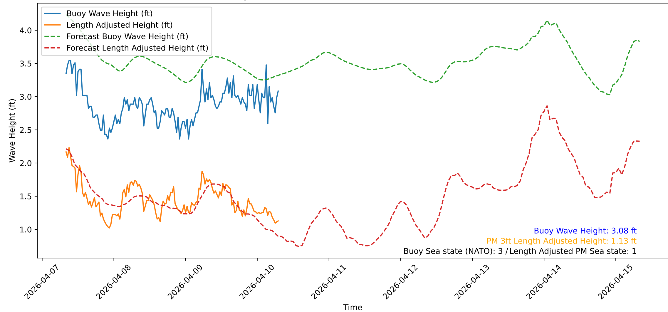
Wave Heights over Time for Green Beach at 2026-04-10 08:01:13
