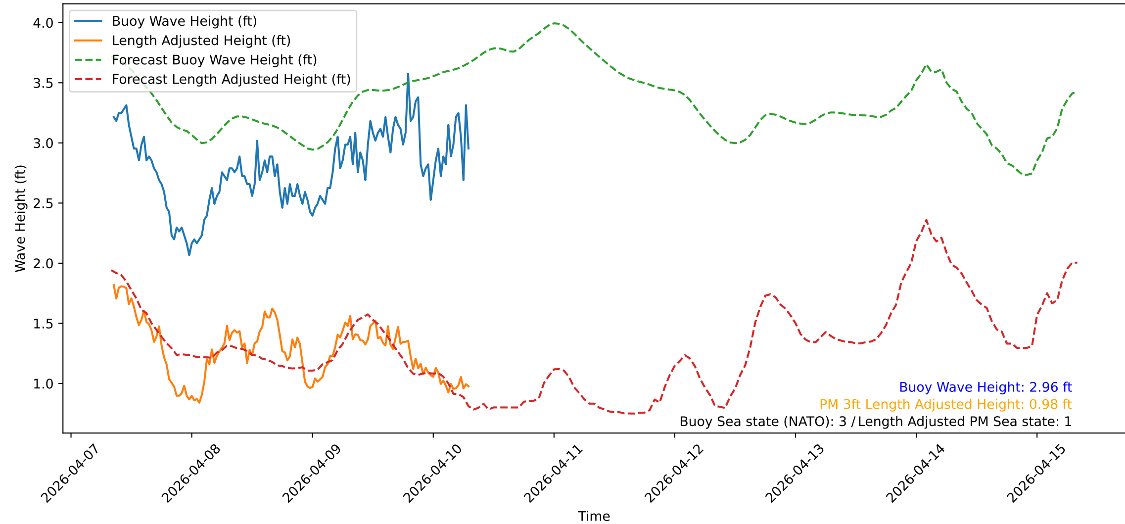
Wave Heights over Time for Red Beach at 2026-04-10 08:00:51
