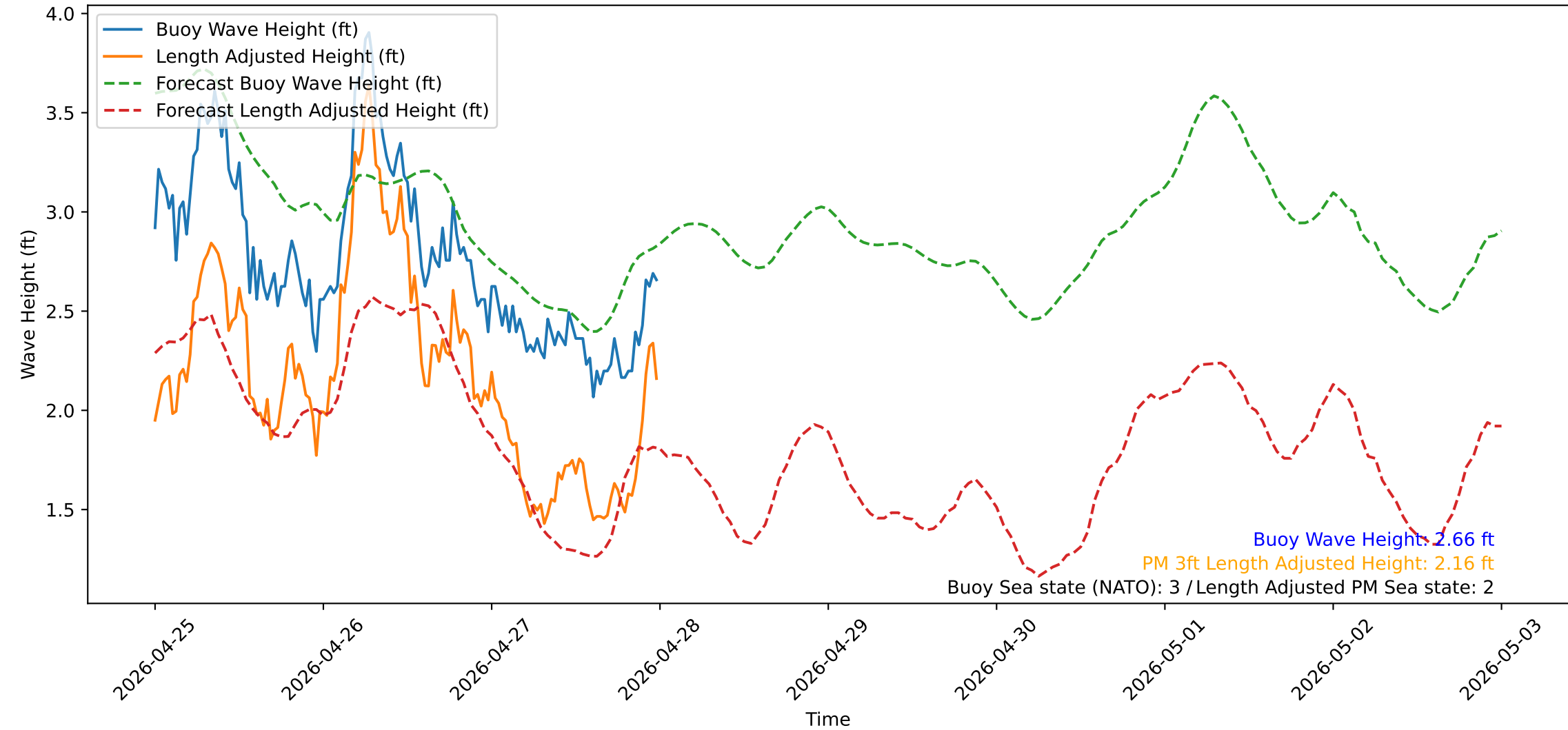
Wave Heights over Time for Oceanside Harbor at 2026-04-28 00:00:31
