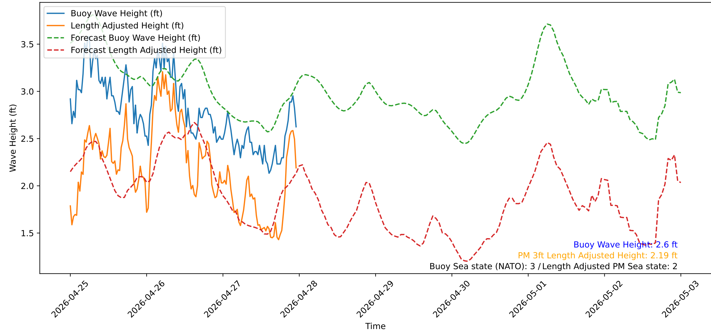
Wave Heights over Time for Green Beach at 2026-04-28 00:01:13
