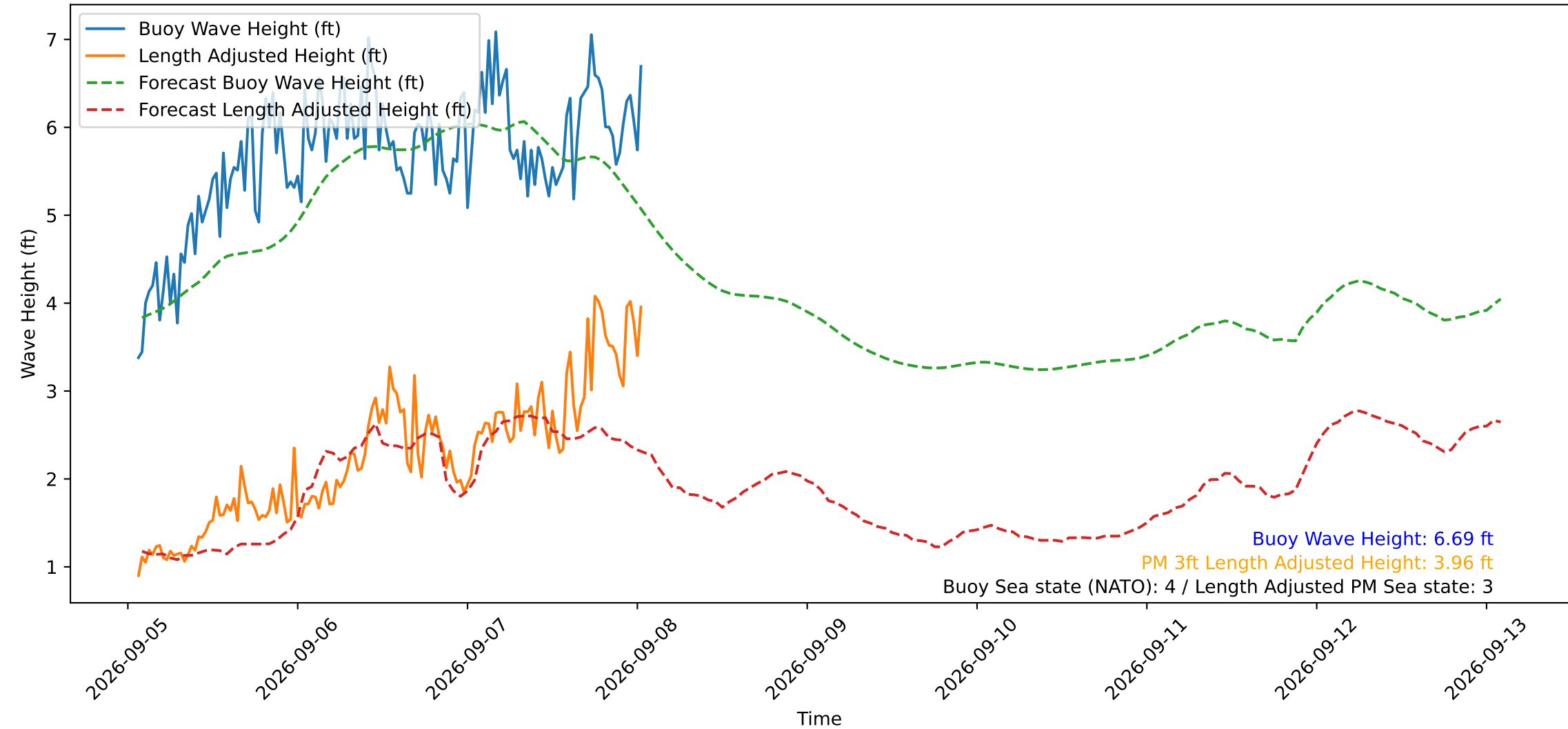
Wave Heights over Time for Oceanside Harbor at 2026-09-08 01:30:30
