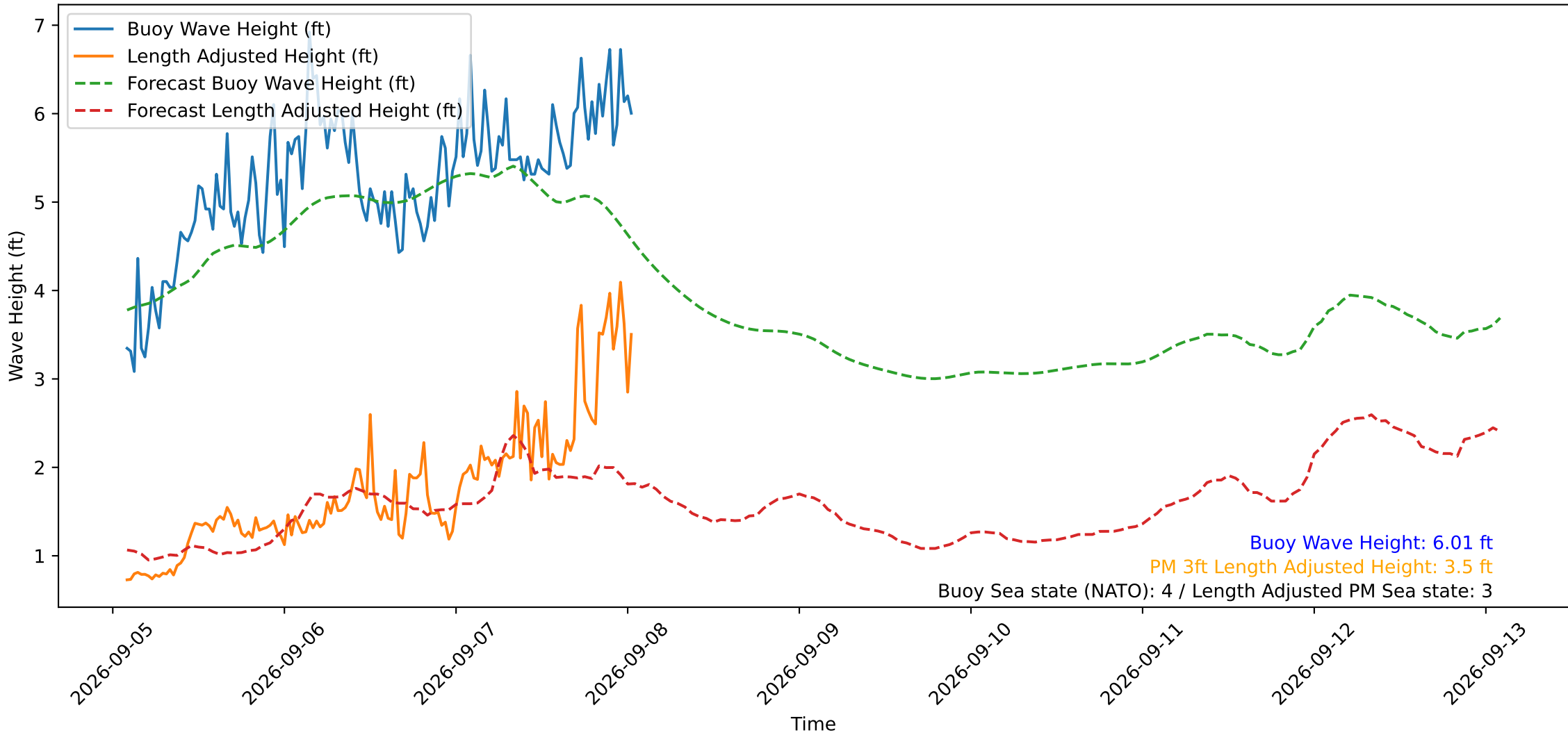
Wave Heights over Time for Red Beach at 2026-09-08 01:30:49
