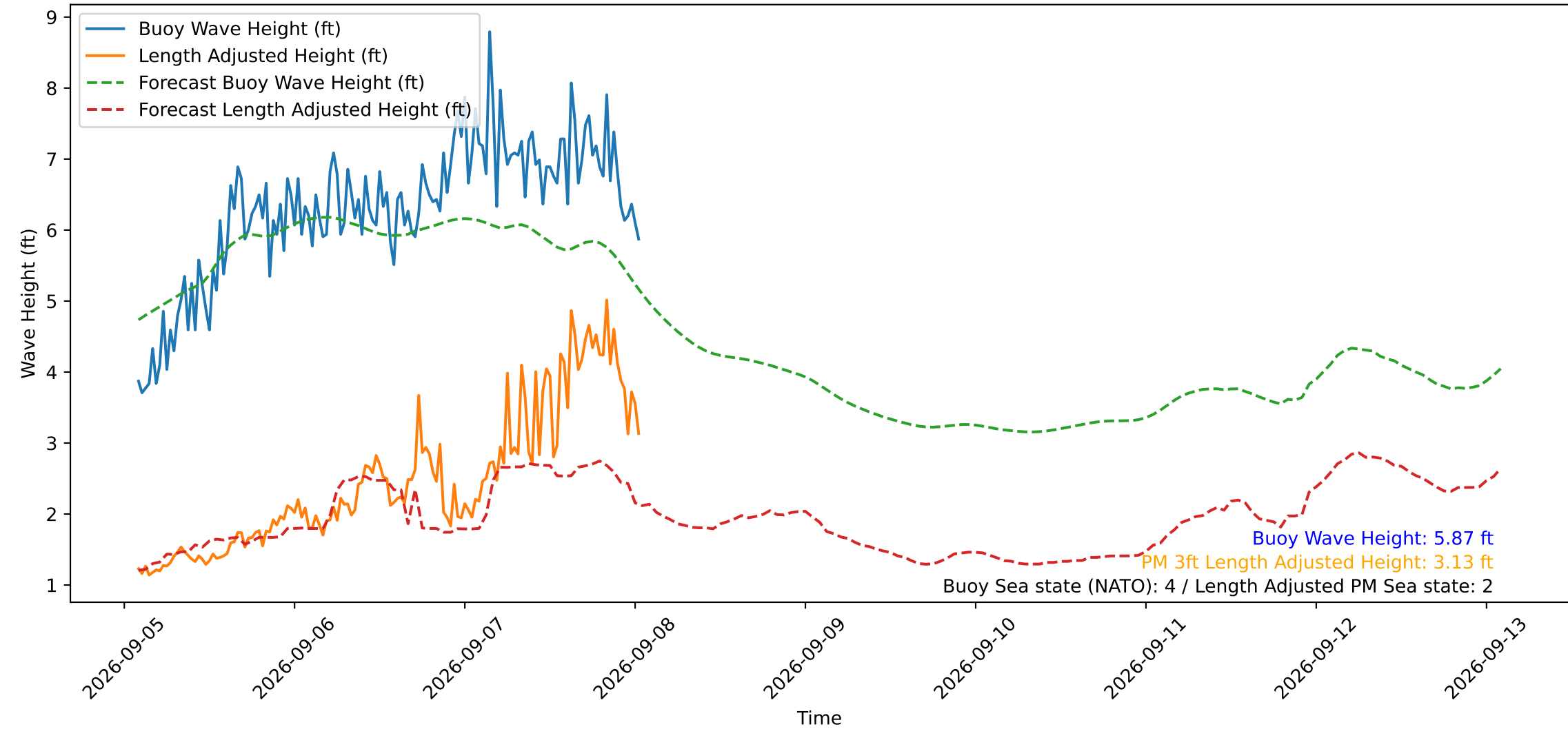
Wave Heights over Time for Green Beach at 2026-09-08 01:31:12
