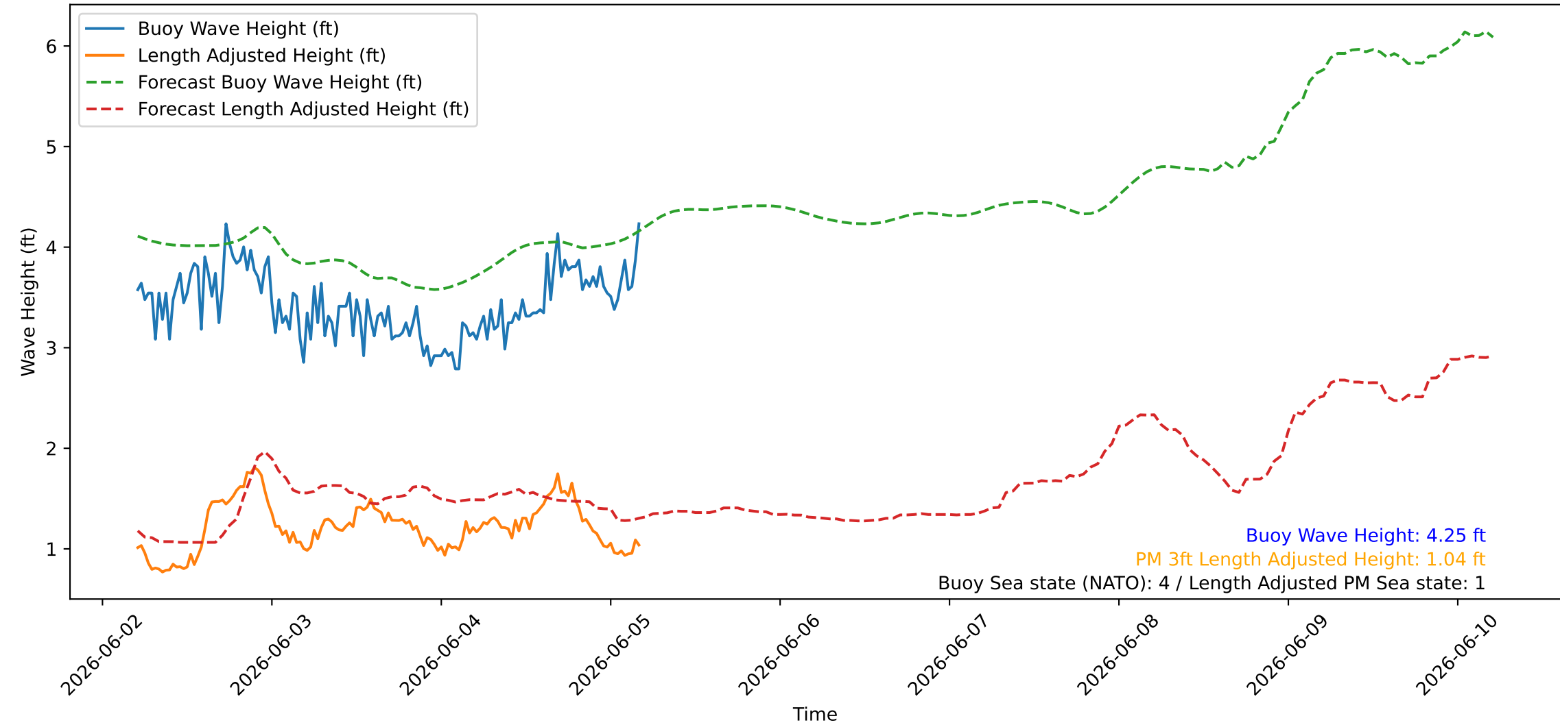
Wave Heights over Time for Green Beach at 2026-06-05 04:51:08
