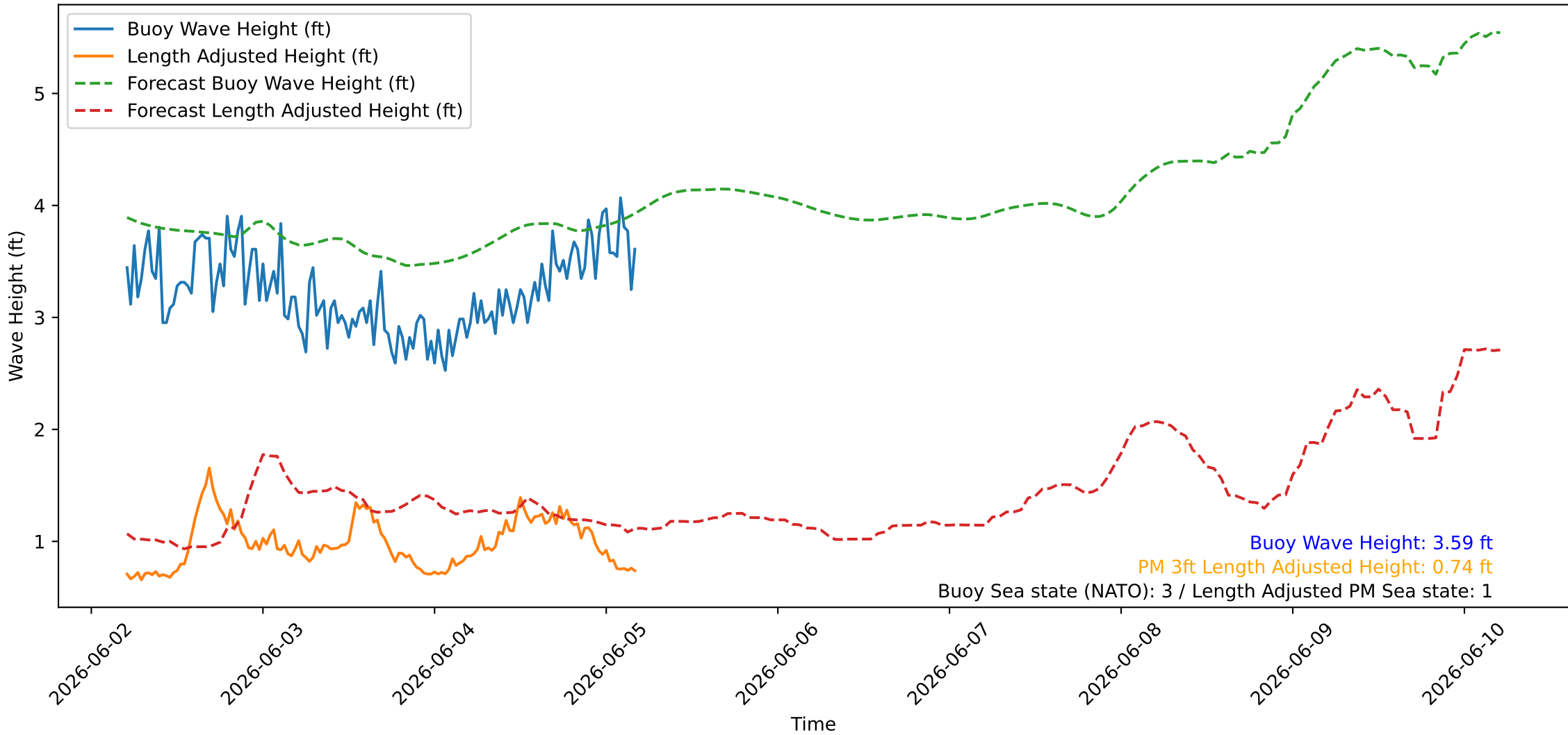
Wave Heights over Time for Red Beach at 2026-06-05 04:50:46
