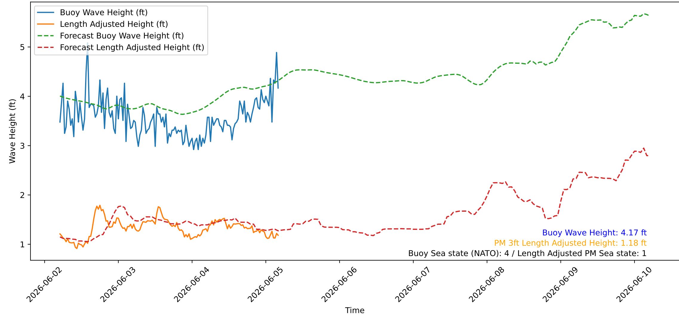
Wave Heights over Time for Oceanside Harbor at 2026-06-05 04:50:25
