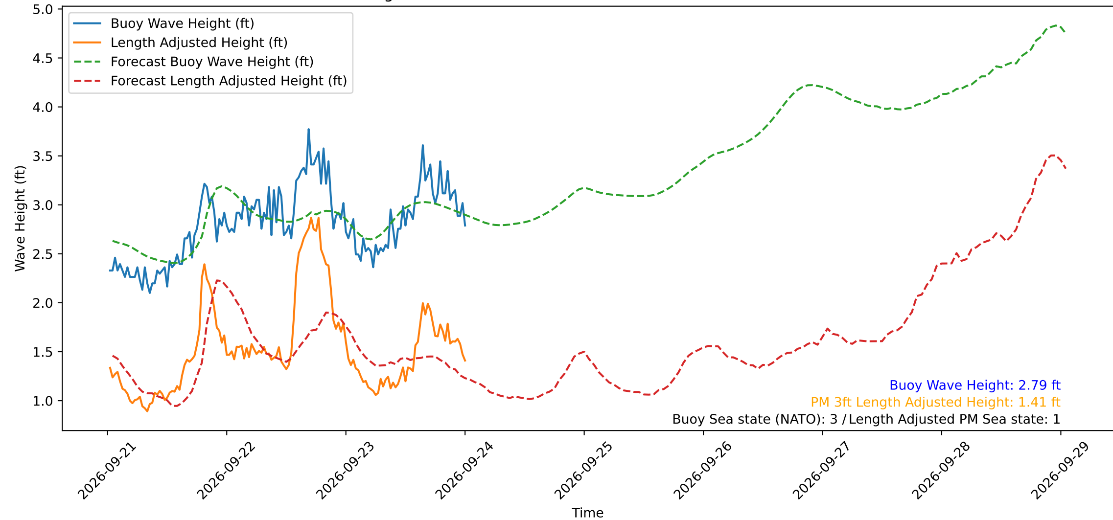
Wave Heights over Time for Oceanside Harbor at 2026-09-24 00:30:29
