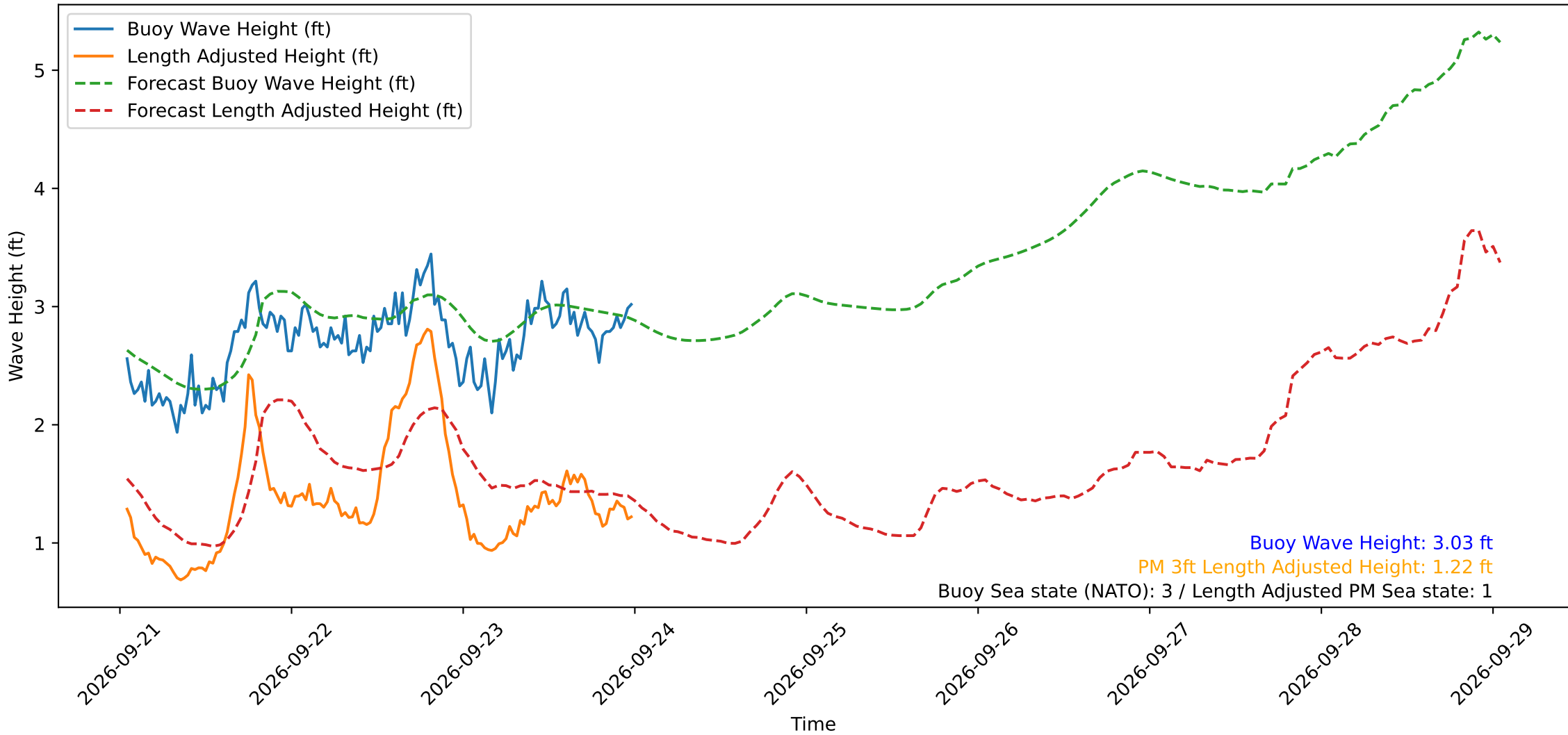
Wave Heights over Time for Green Beach at 2026-09-24 00:31:11
