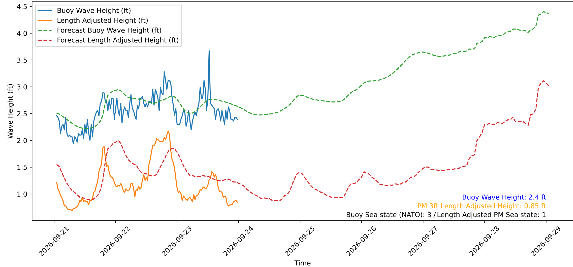
Wave Heights over Time for Red Beach at 2026-09-24 00:30:48
