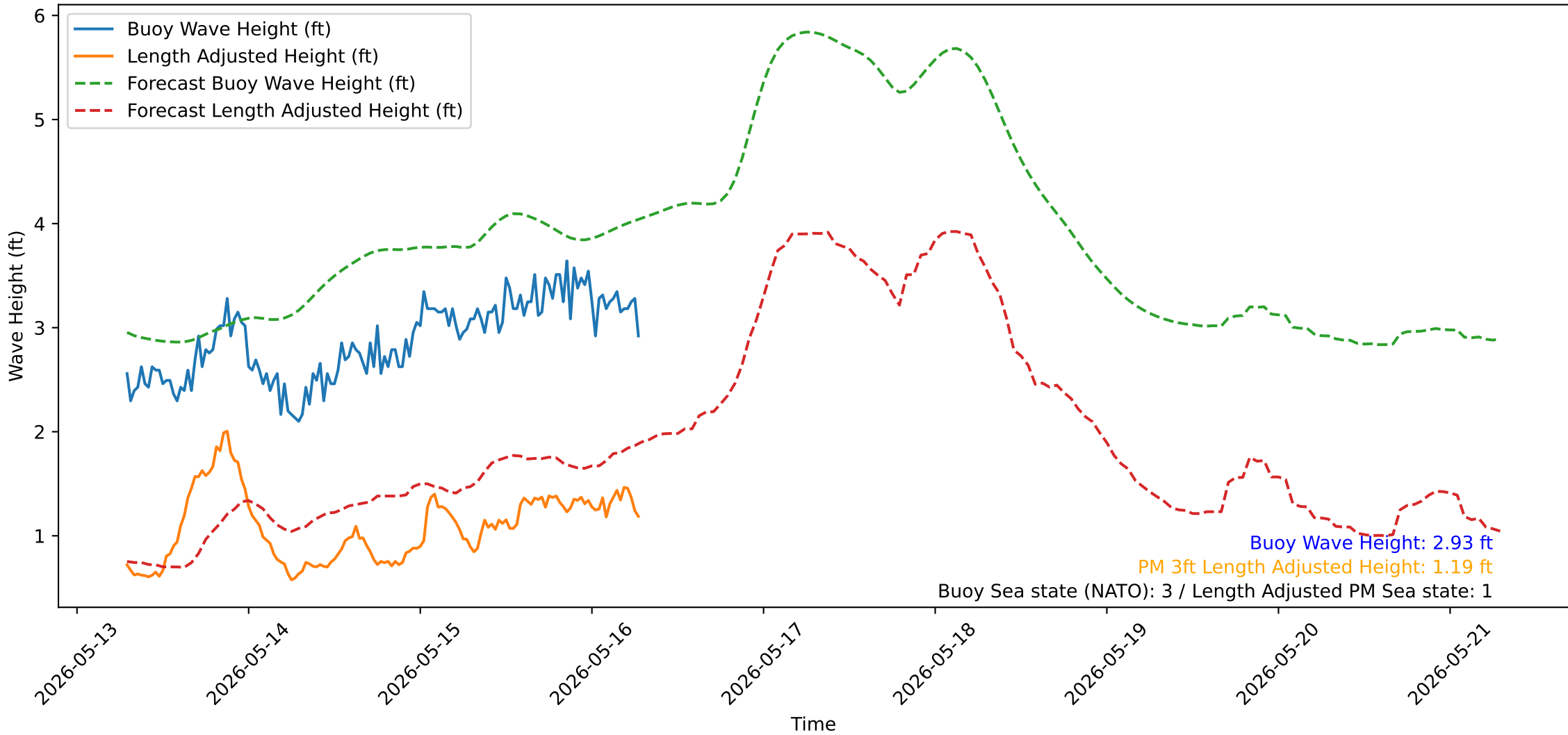
Wave Heights over Time for Green Beach at 2026-05-16 07:11:14
