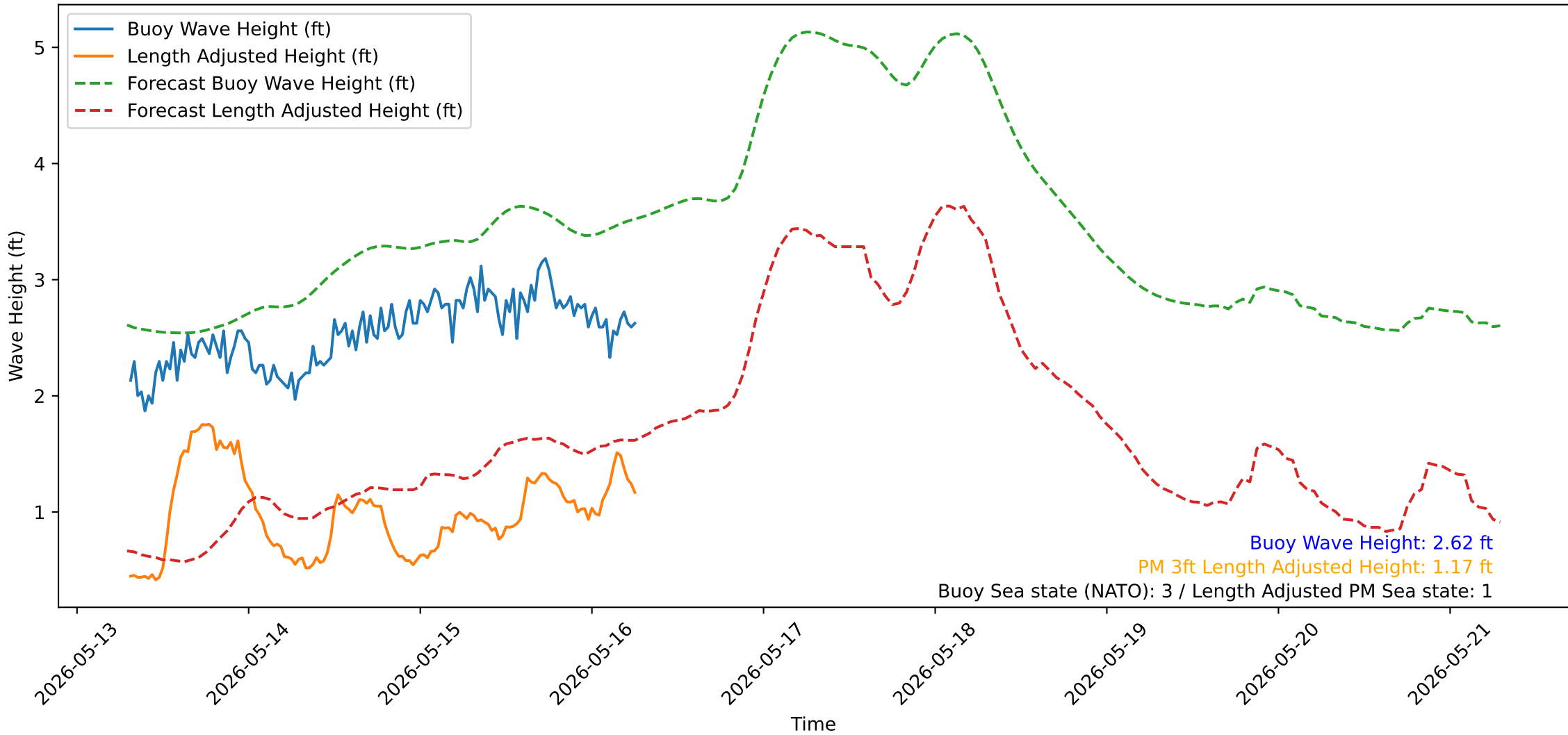
Wave Heights over Time for Red Beach at 2026-05-16 07:10:52
