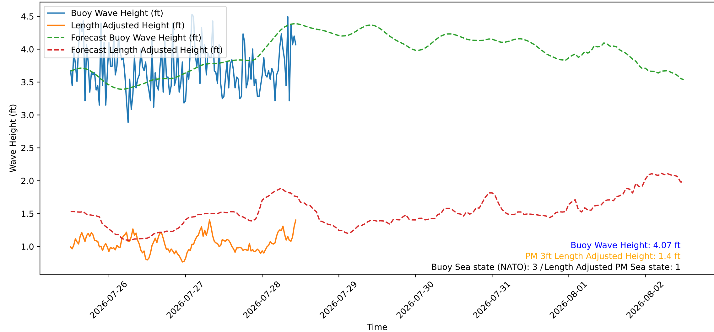
Wave Heights over Time for Red Beach at 2026-07-28 11:30:45
