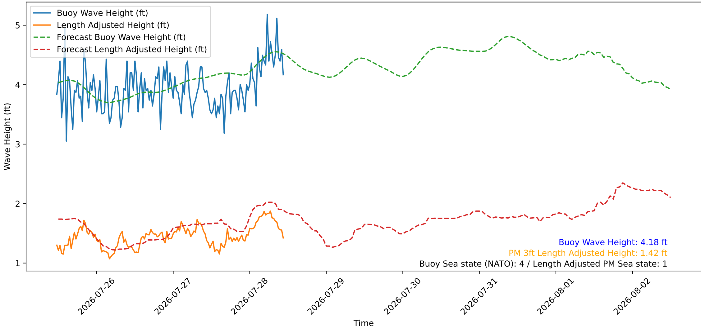
Wave Heights over Time for Oceanside Harbor at 2026-07-28 11:30:26
