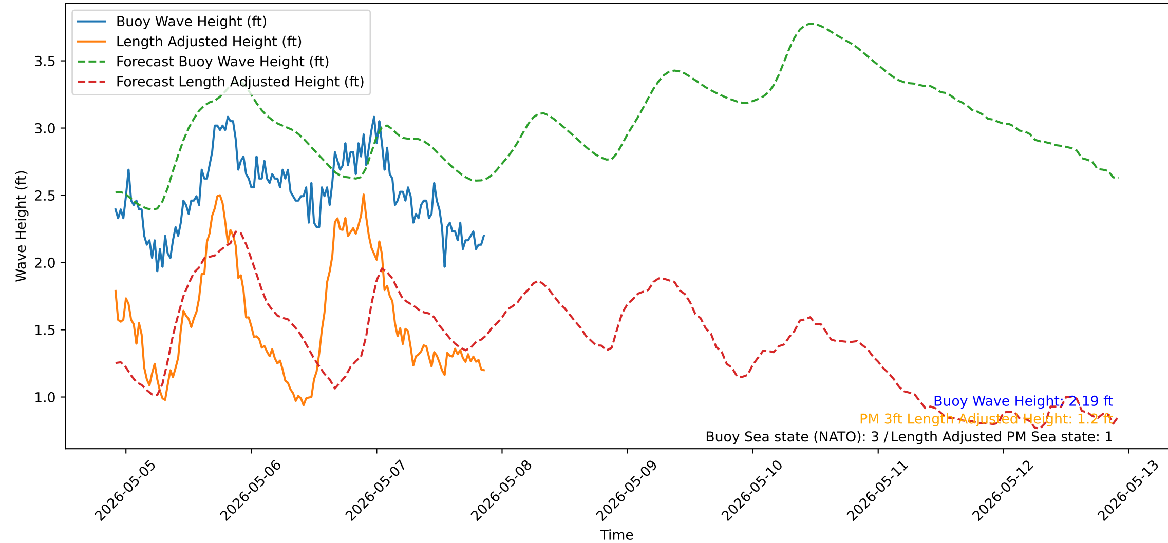
Wave Heights over Time for Red Beach at 2026-05-07 21:30:50
