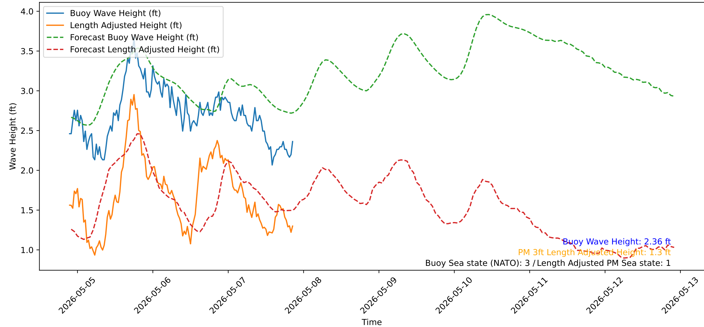
Wave Heights over Time for Green Beach at 2026-05-07 21:31:12
