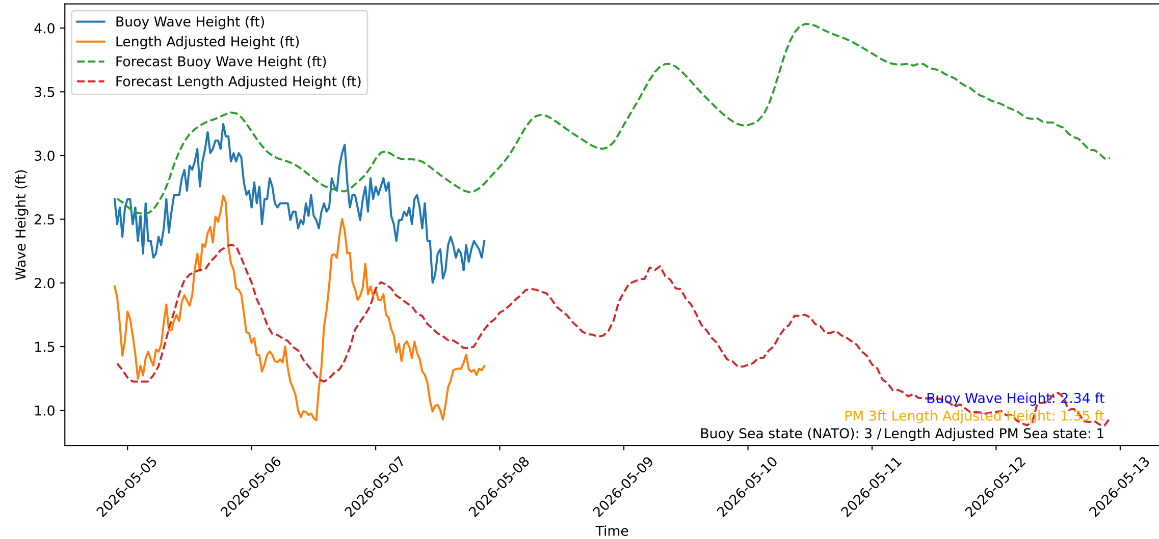
Wave Heights over Time for Oceanside Harbor at 2026-05-07 21:30:31
