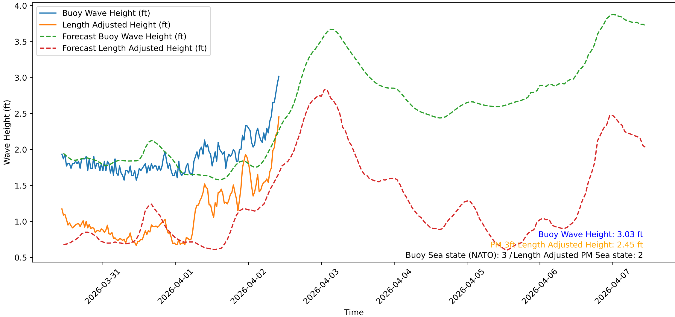
Wave Heights over Time for Oceanside Harbor at 2026-04-02 10:40:31
