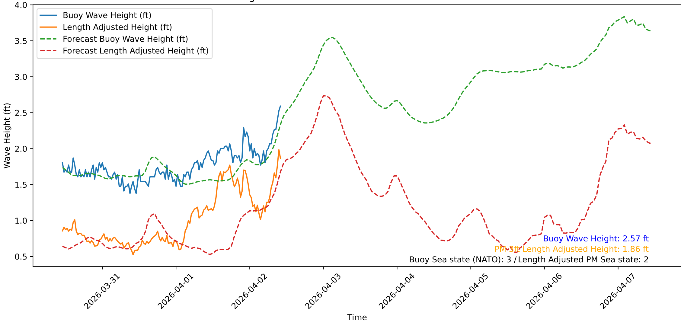
Wave Heights over Time for Red Beach at 2026-04-02 10:40:48
