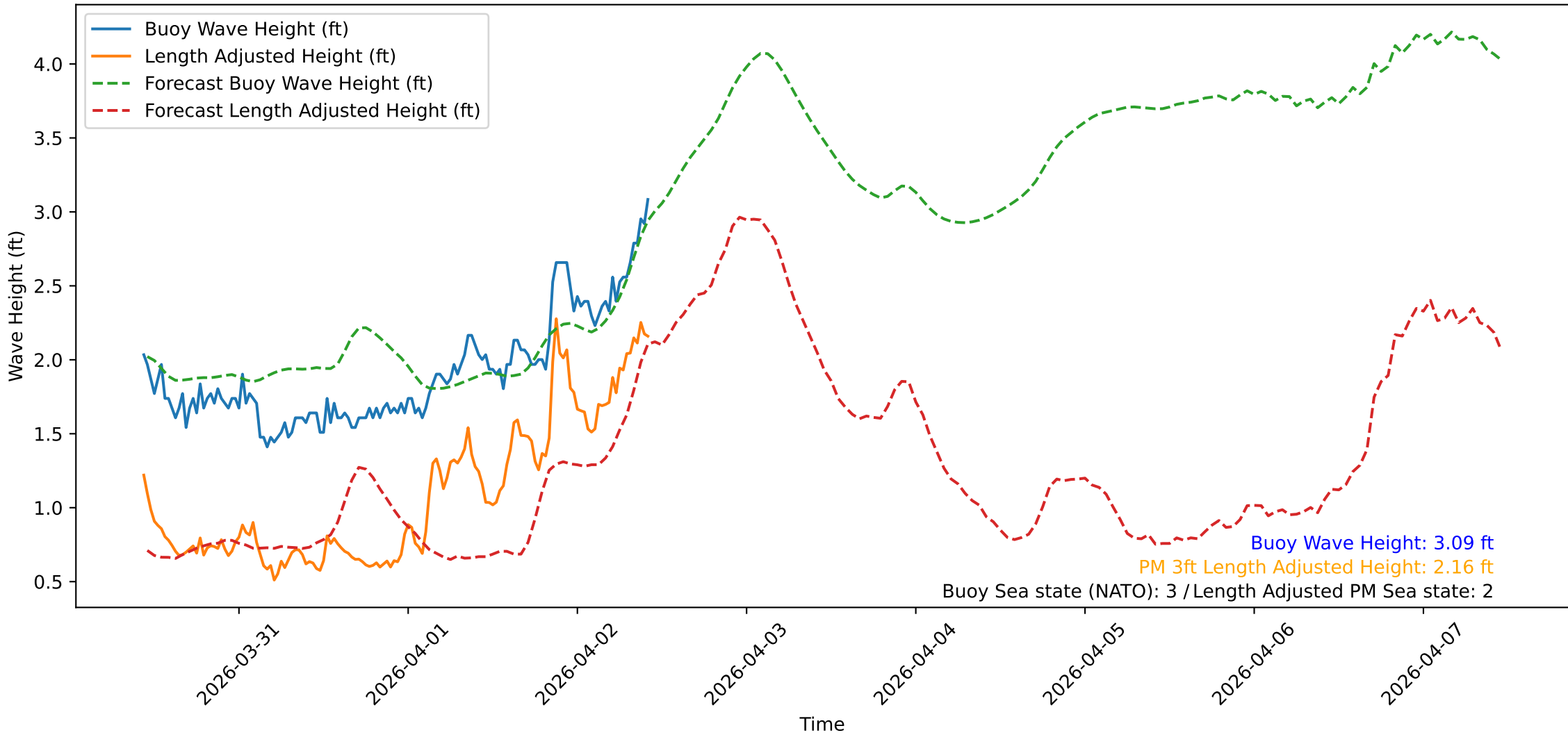
Wave Heights over Time for Green Beach at 2026-04-02 10:41:10
