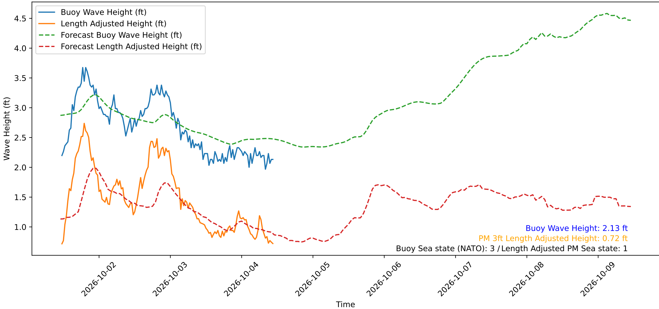
Wave Heights over Time for Green Beach at 2026-10-04 11:21:14
