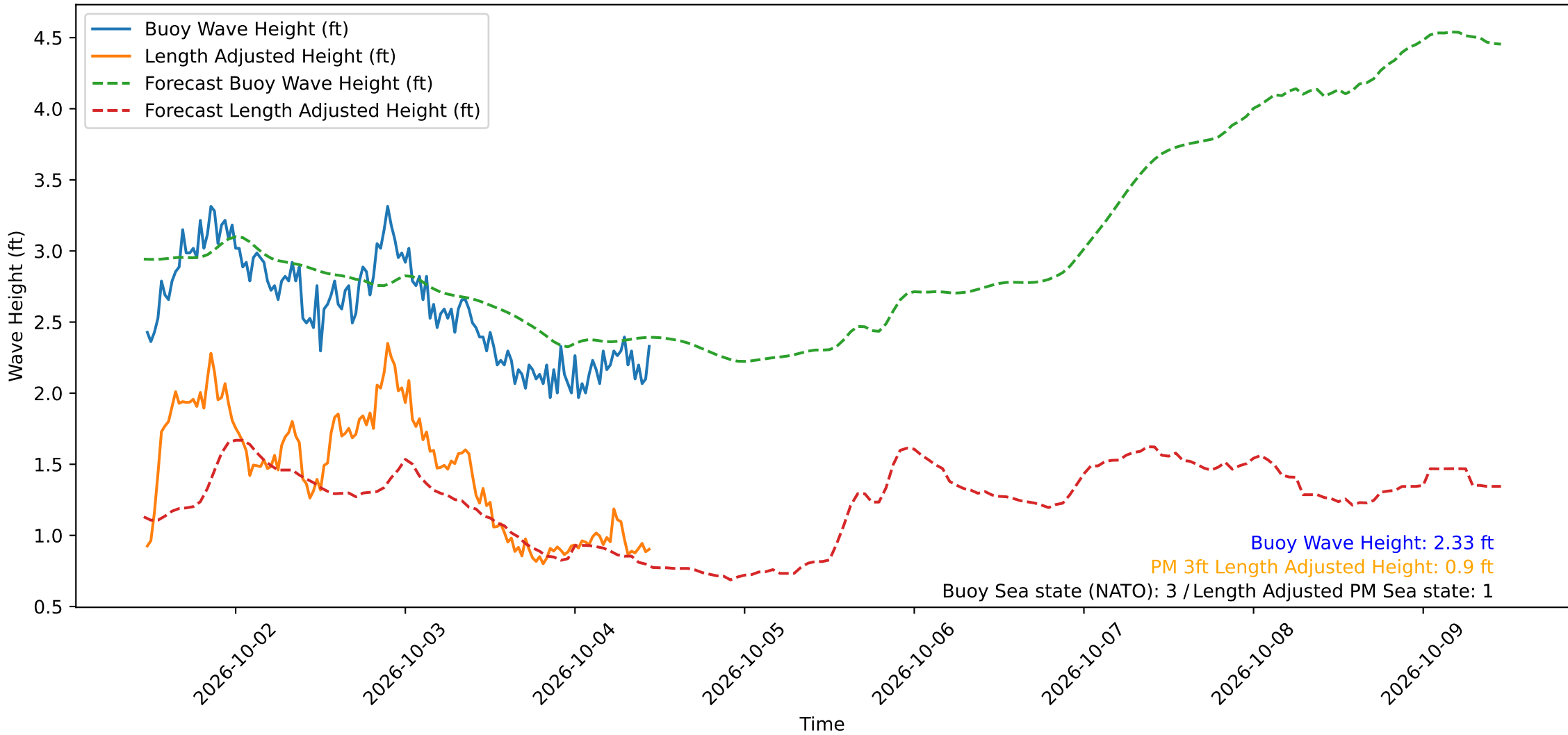
Wave Heights over Time for Oceanside Harbor at 2026-10-04 11:20:29
