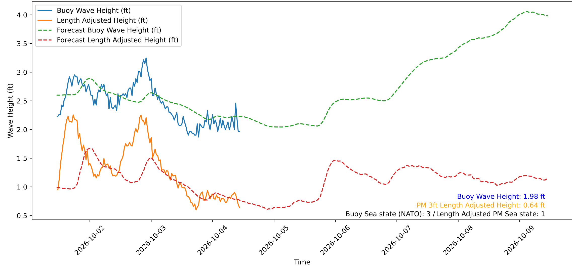
Wave Heights over Time for Red Beach at 2026-10-04 11:20:50
