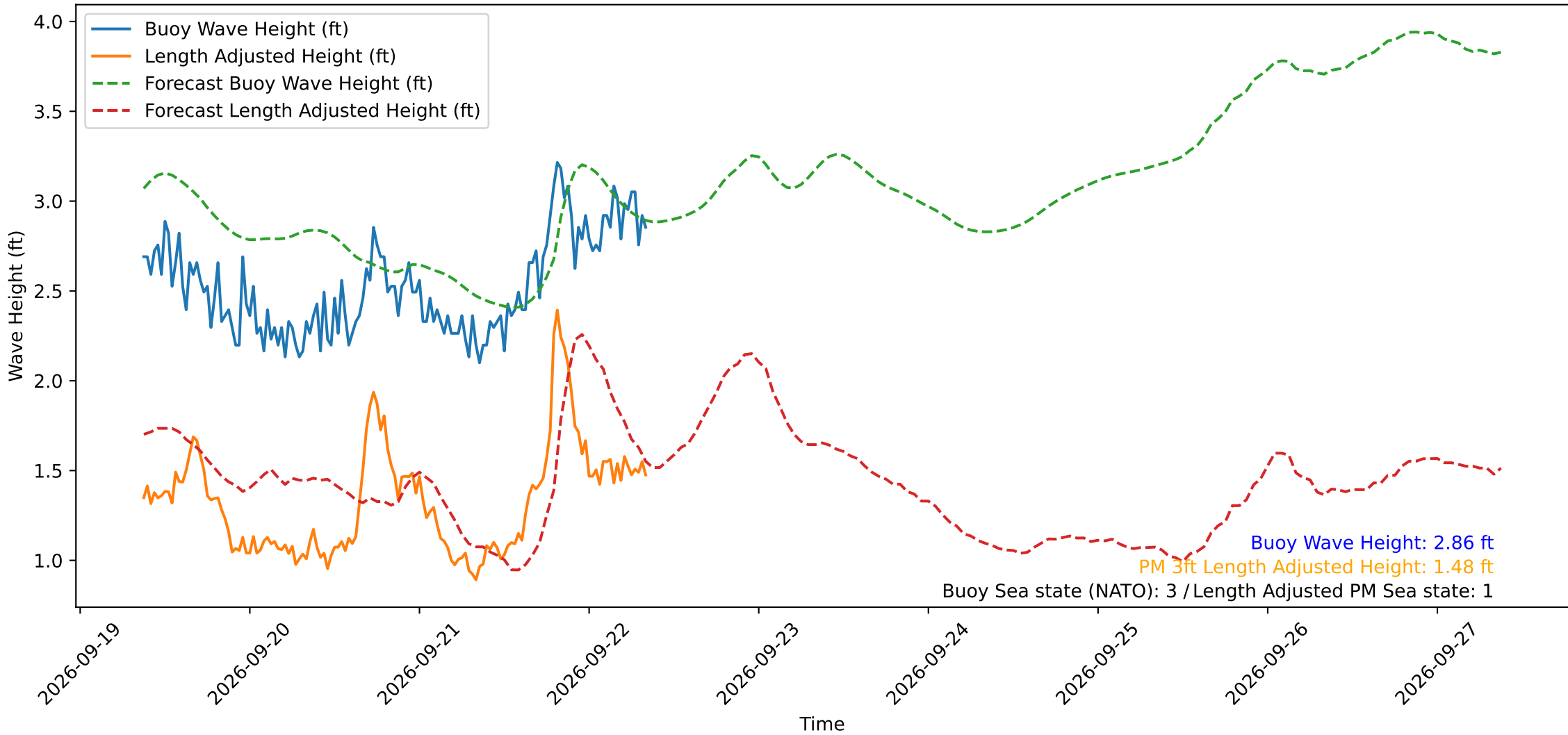
Wave Heights over Time for Oceanside Harbor at 2026-09-22 08:50:29
