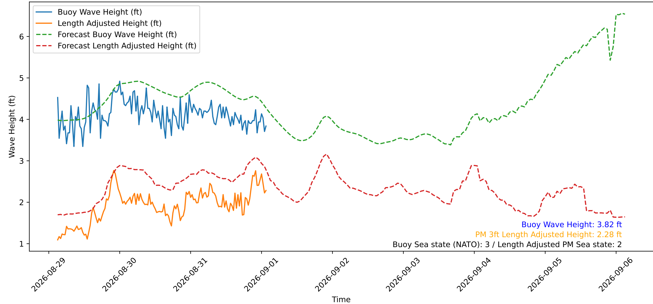
Wave Heights over Time for Green Beach at 2026-09-01 02:31:12
