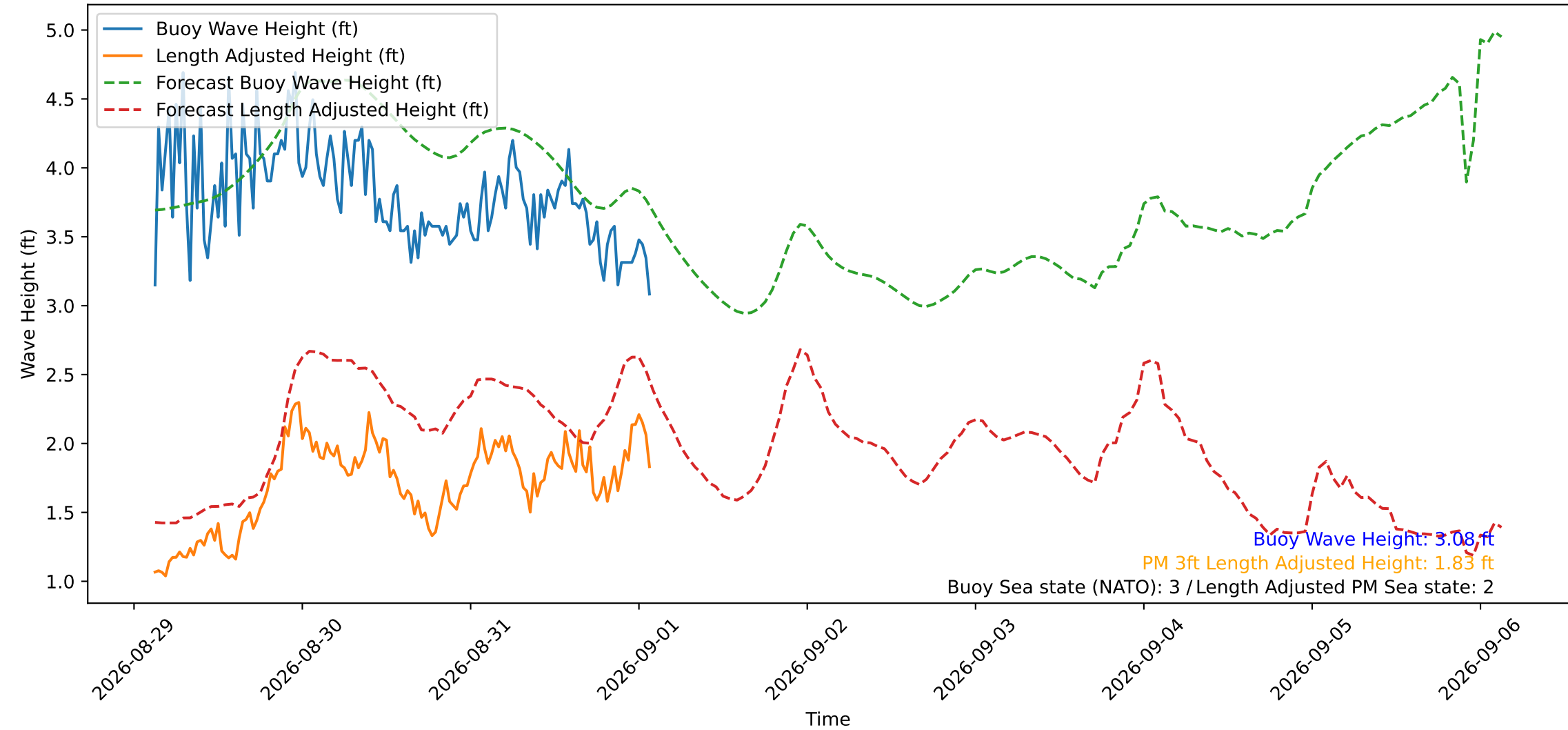
Wave Heights over Time for Red Beach at 2026-09-01 02:30:49
