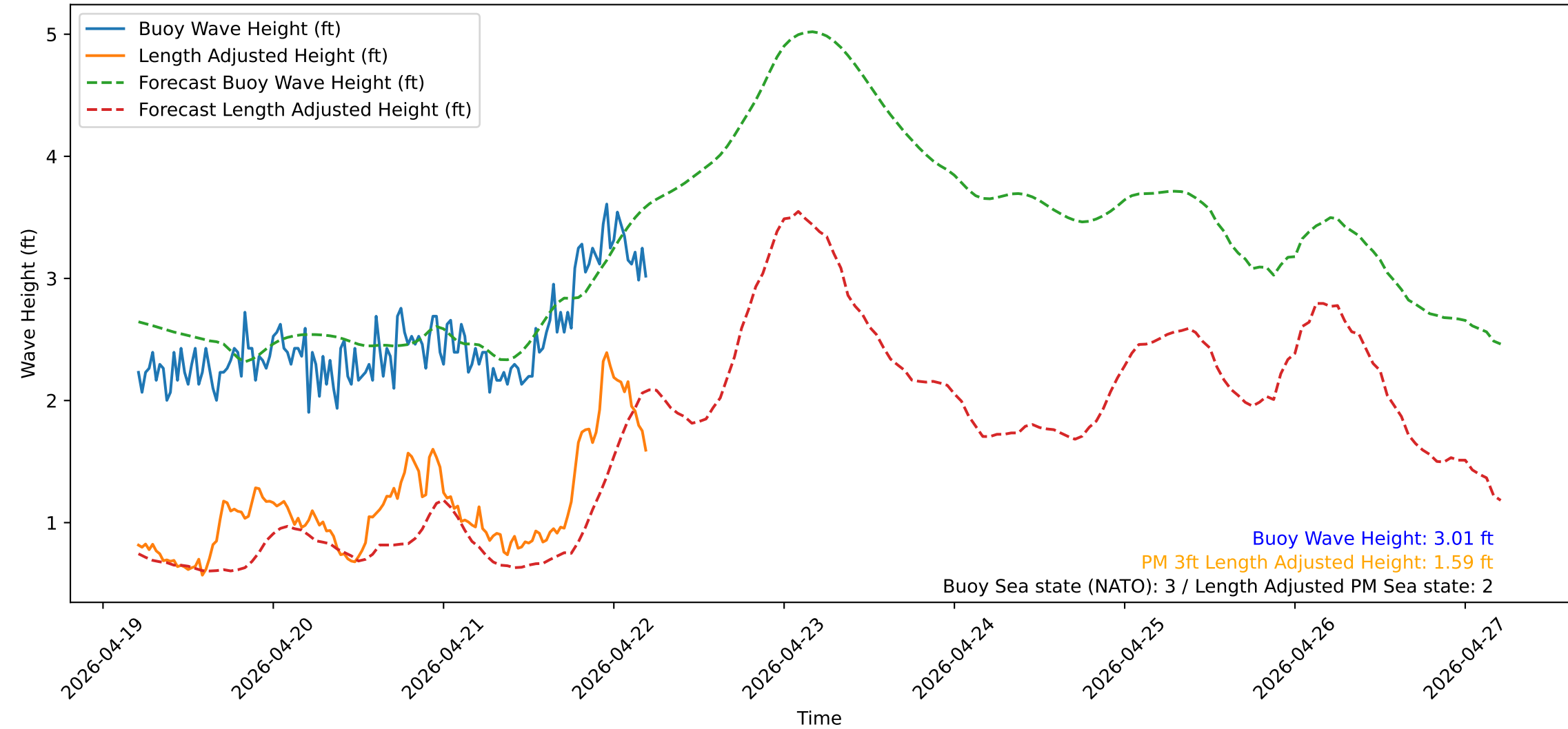
Wave Heights over Time for Oceanside Harbor at 2026-04-22 05:10:31
