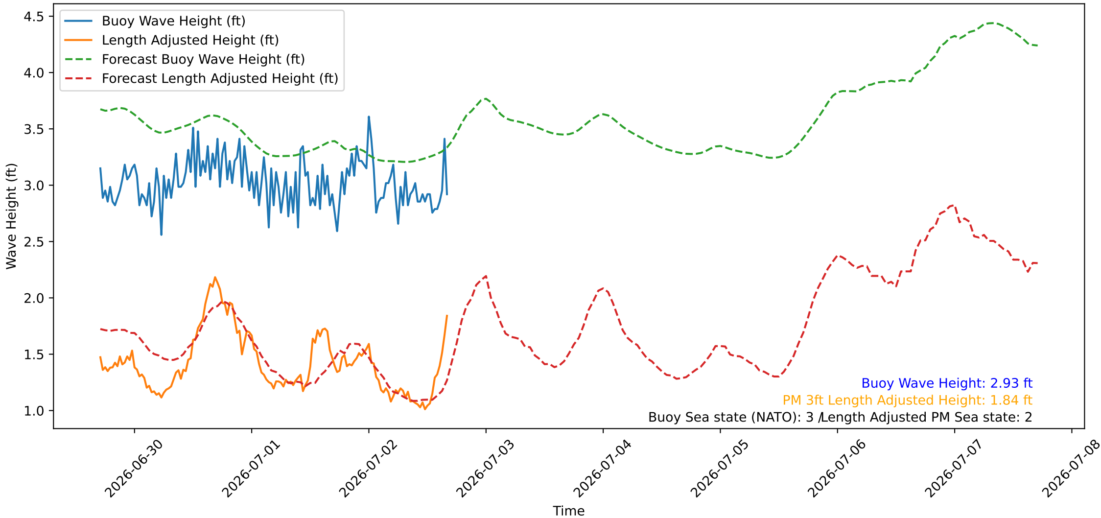
Wave Heights over Time for Oceanside Harbor at 2026-07-02 16:50:26
