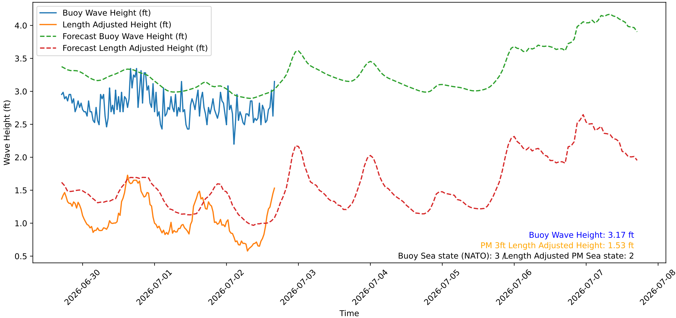
Wave Heights over Time for Red Beach at 2026-07-02 16:50:47
