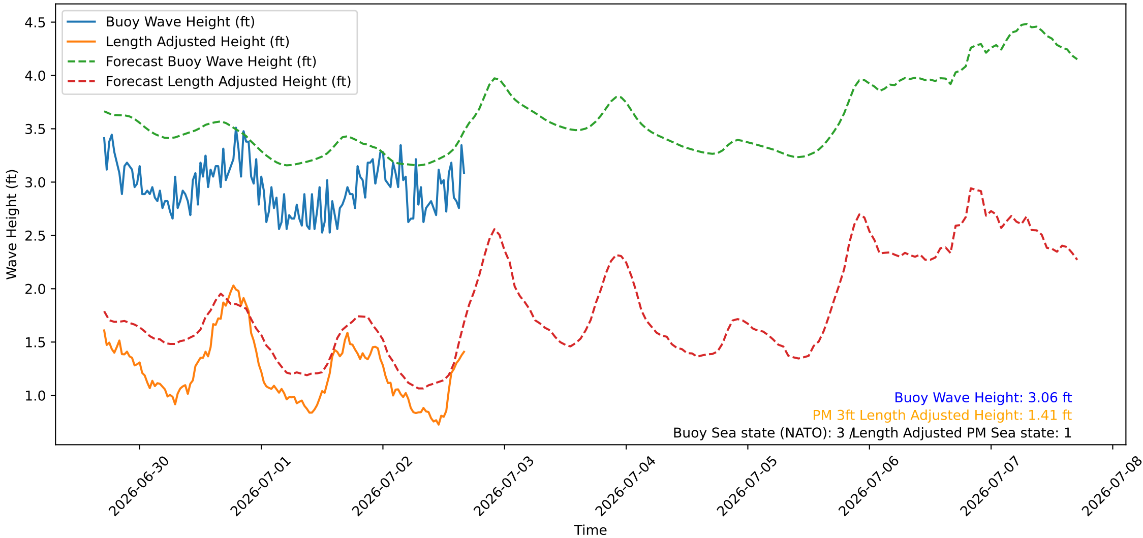
Wave Heights over Time for Green Beach at 2026-07-02 16:51:10
