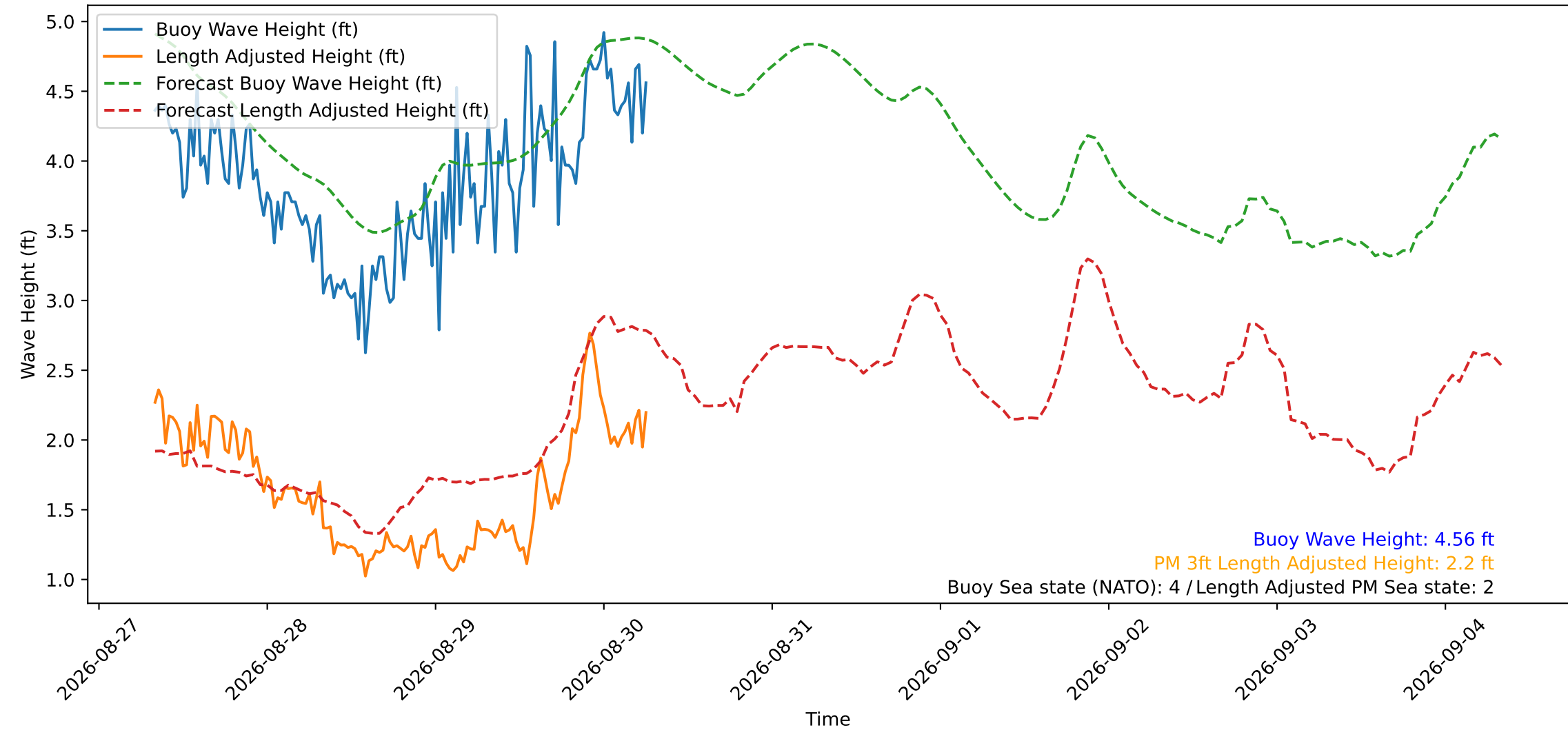
Wave Heights over Time for Green Beach at 2026-08-30 07:51:15
