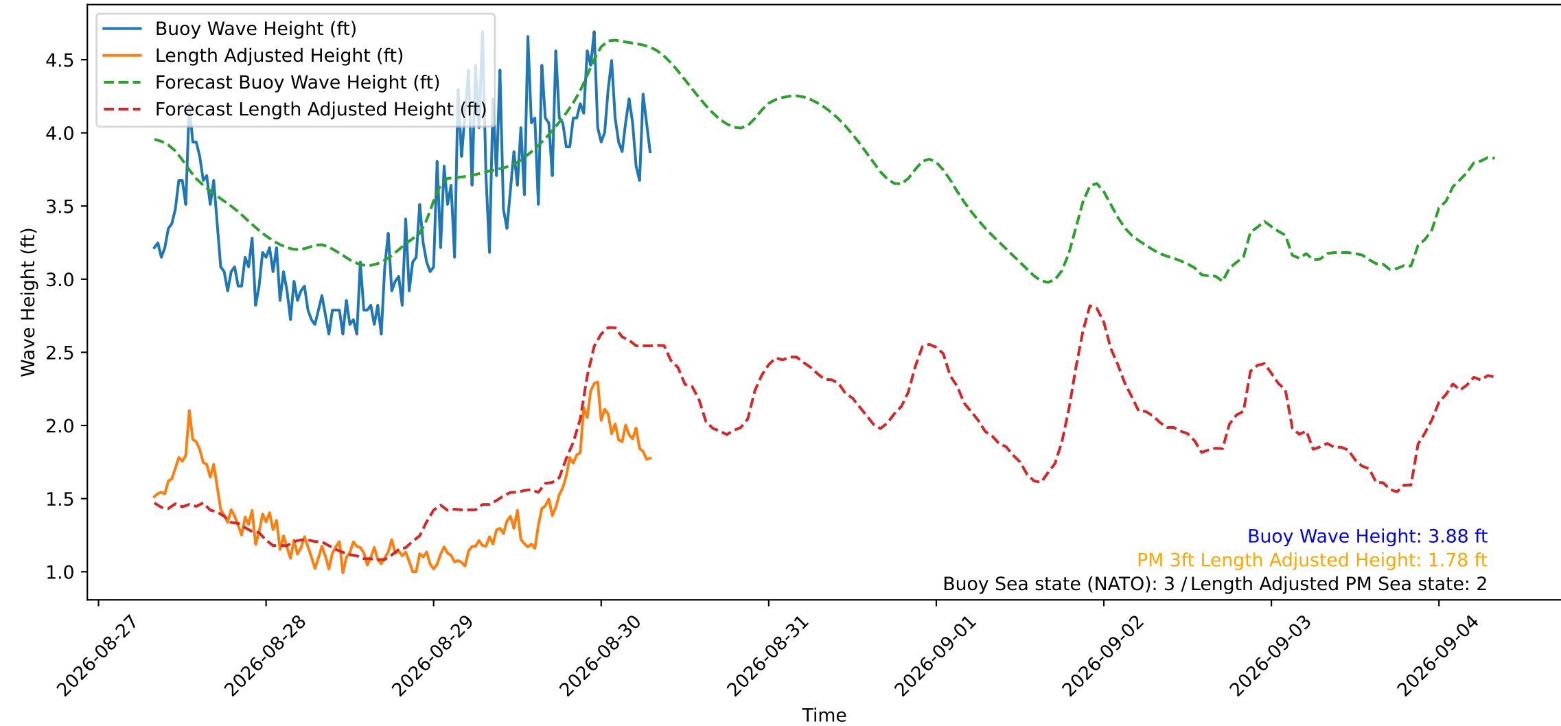
Wave Heights over Time for Red Beach at 2026-08-30 07:50:51
