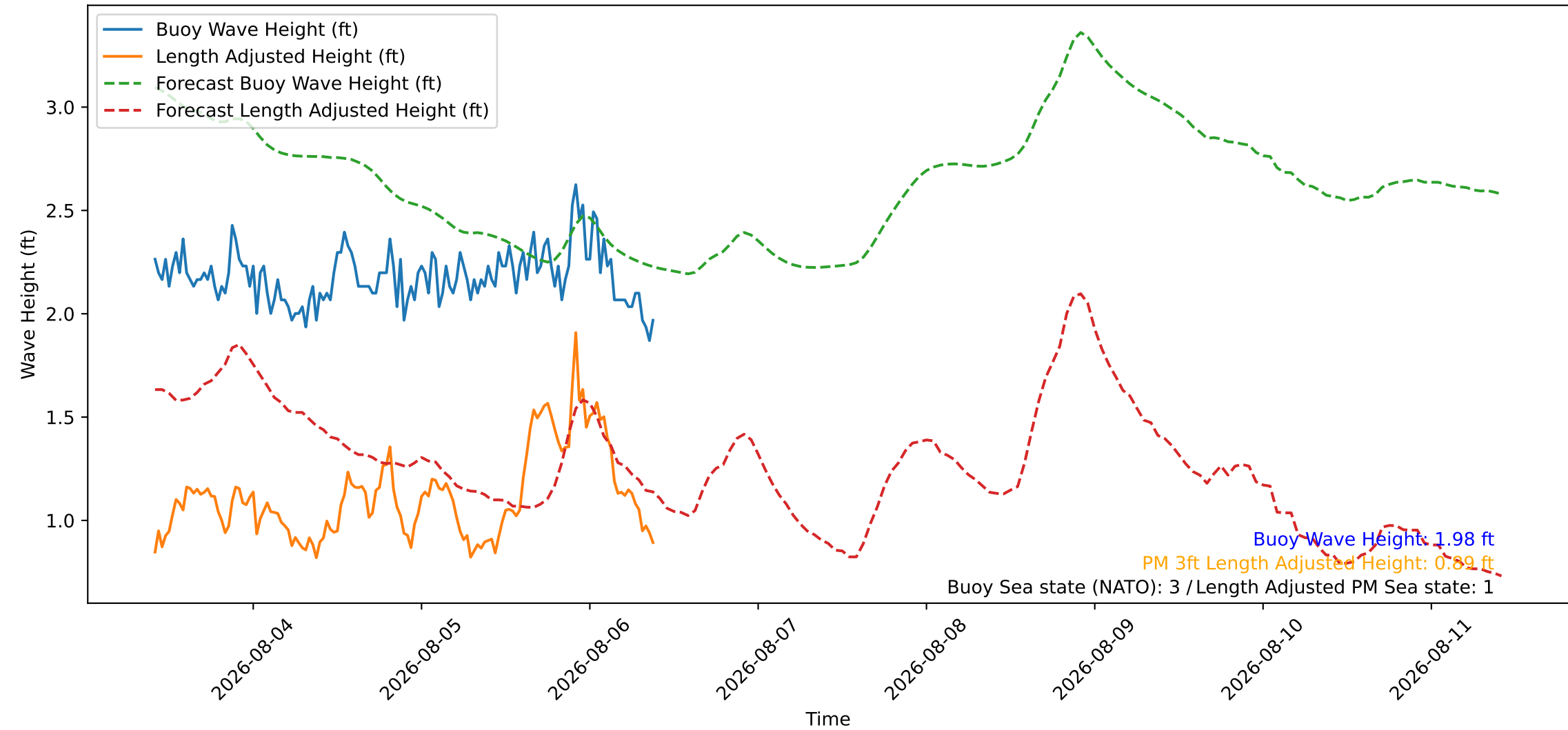
Wave Heights over Time for Green Beach at 2026-08-06 10:01:07
