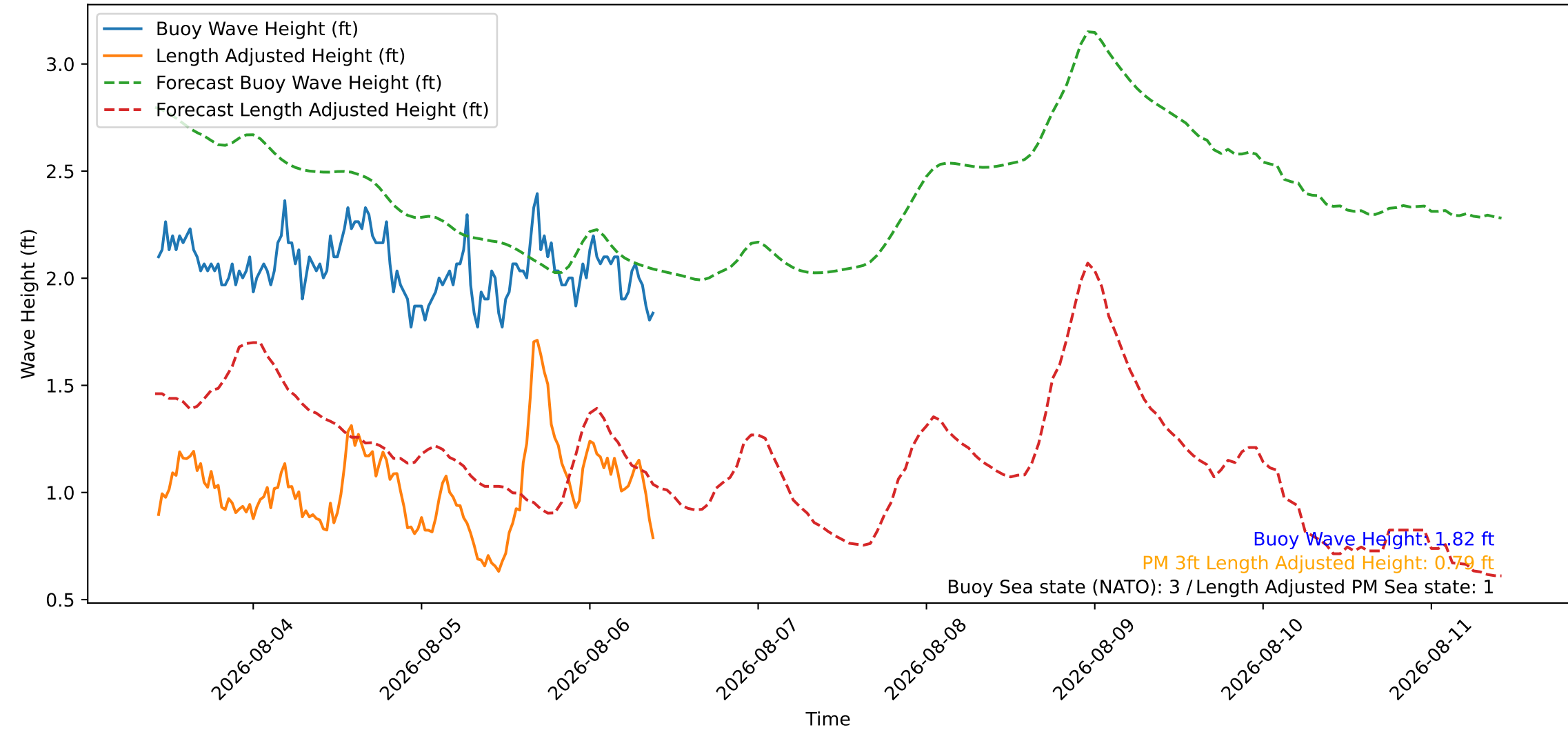
Wave Heights over Time for Red Beach at 2026-08-06 10:00:45
