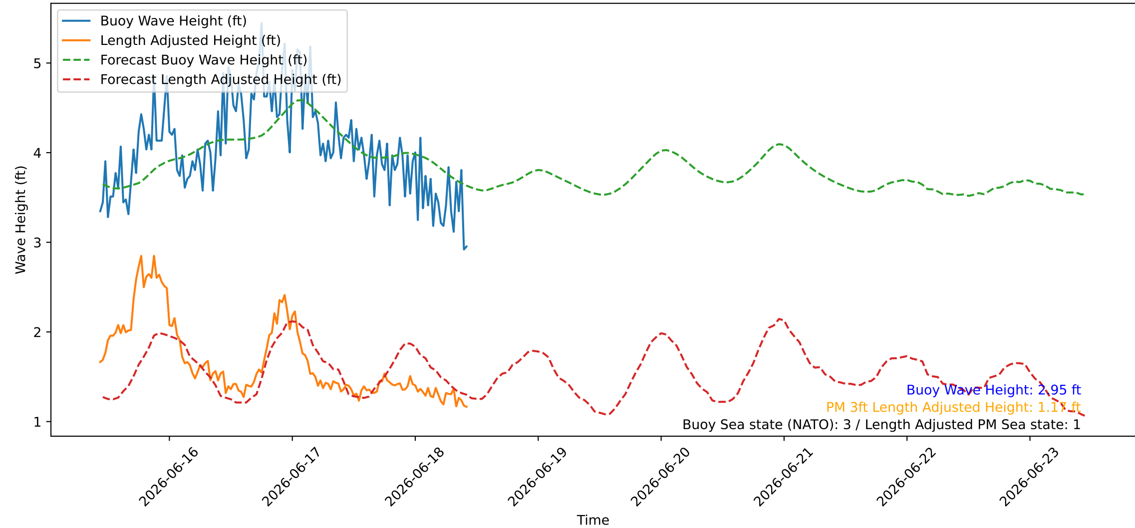
Wave Heights over Time for Oceanside Harbor at 2026-06-18 10:40:26
