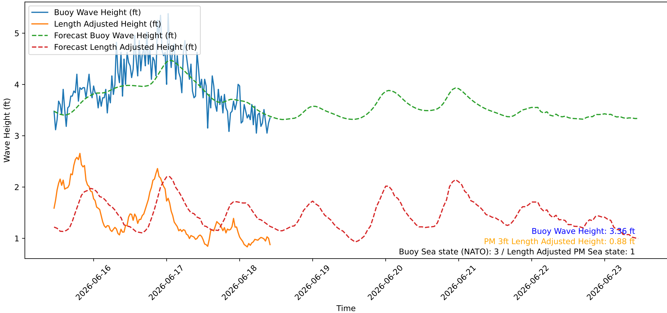
Wave Heights over Time for Red Beach at 2026-06-18 10:40:46
