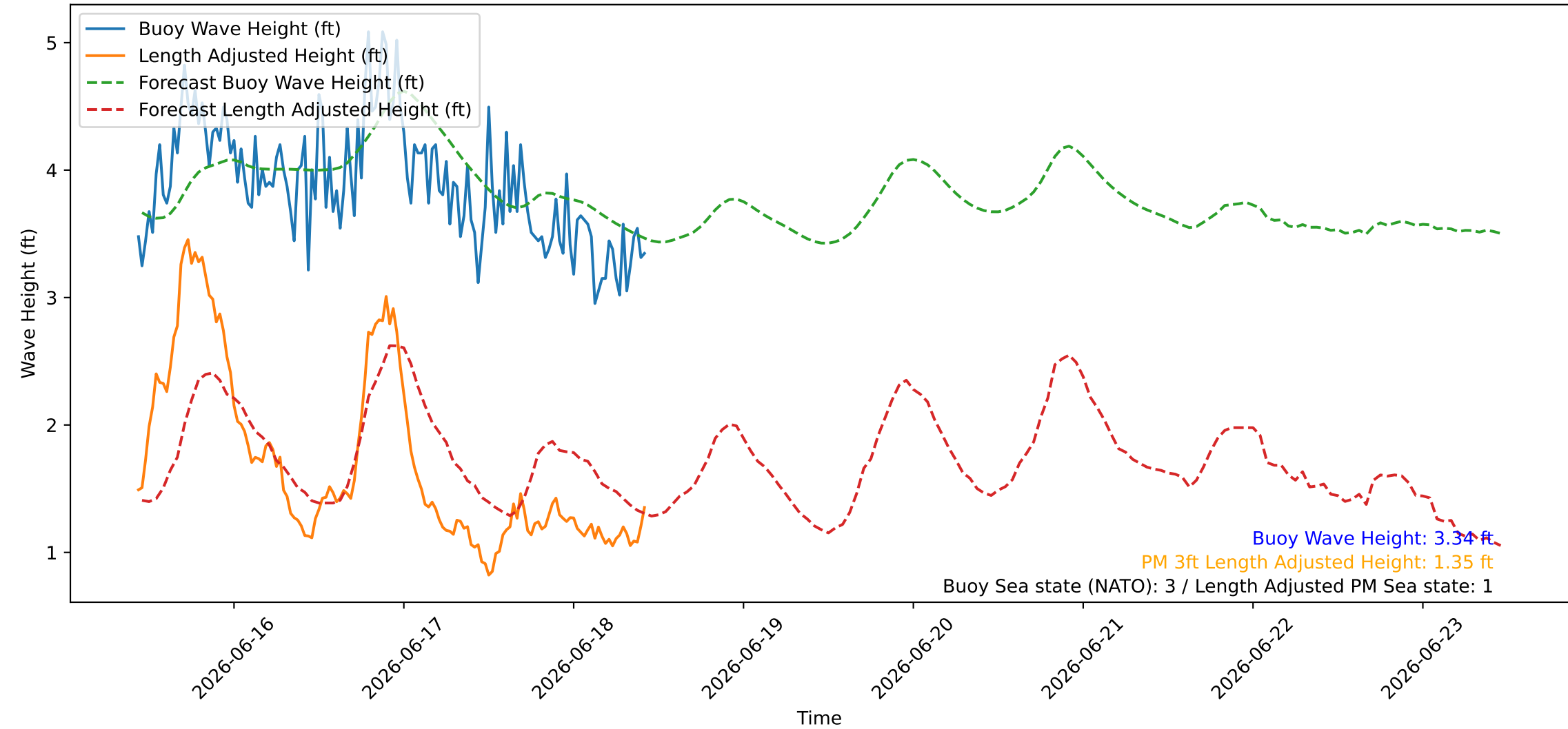
Wave Heights over Time for Green Beach at 2026-06-18 10:41:08
