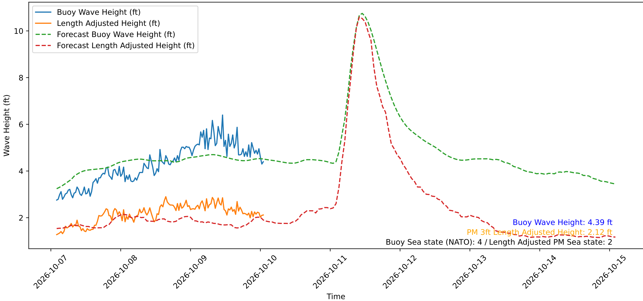
Wave Heights over Time for Oceanside Harbor at 2026-10-10 02:00:30
