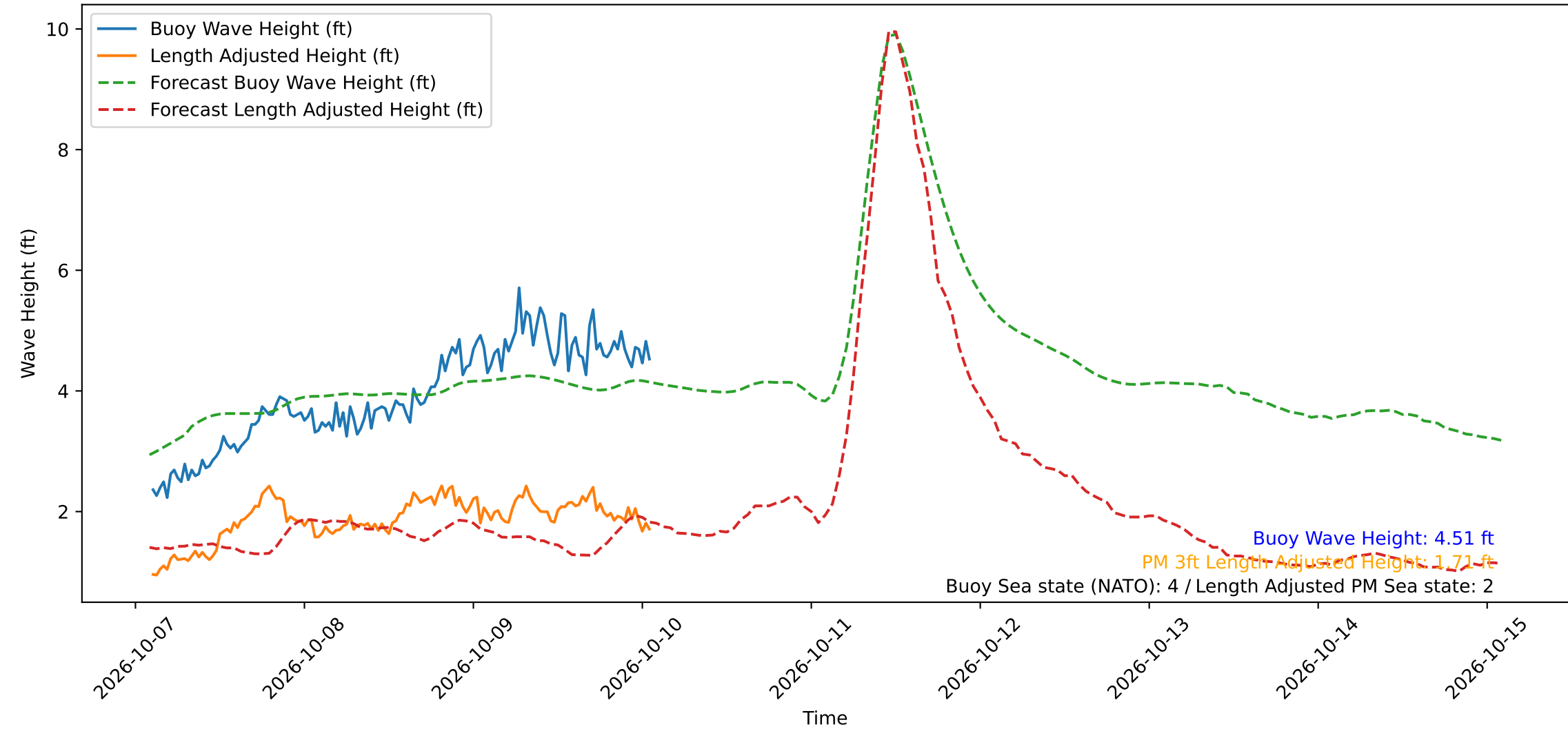
Wave Heights over Time for Red Beach at 2026-10-10 02:00:49
