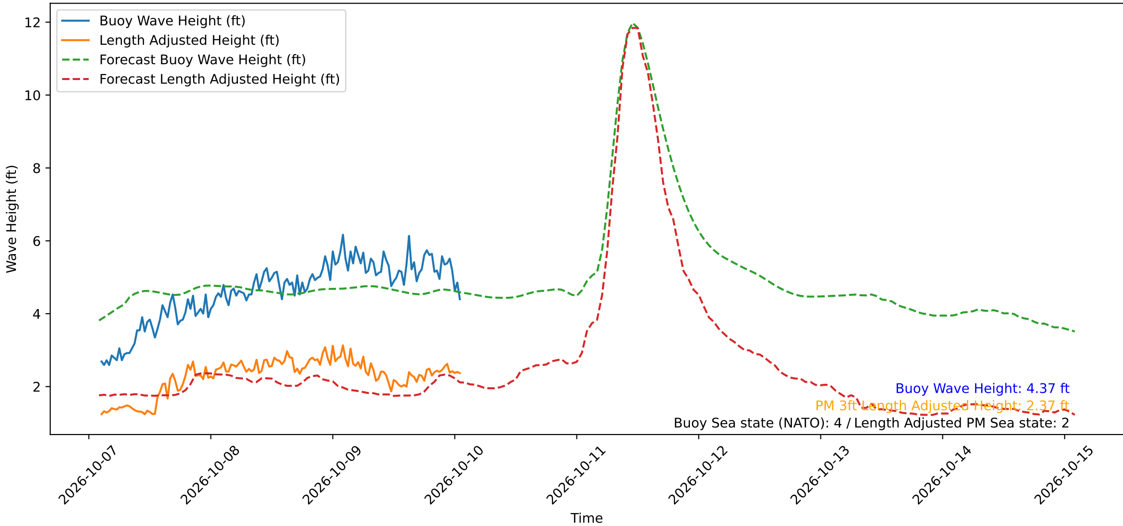
Wave Heights over Time for Green Beach at 2026-10-10 02:01:12
