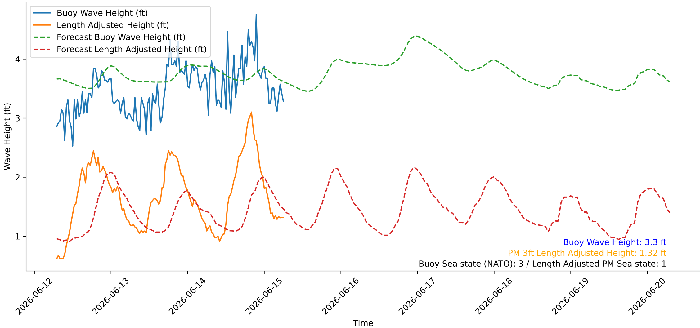
Wave Heights over Time for Red Beach at 2026-06-15 06:50:48
