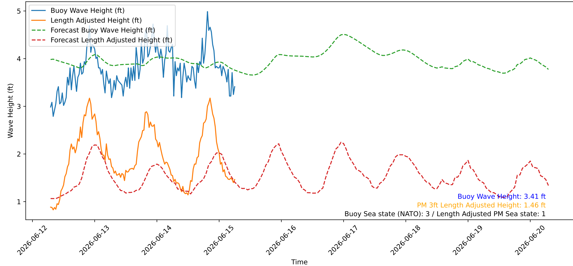
Wave Heights over Time for Oceanside Harbor at 2026-06-15 06:50:27
