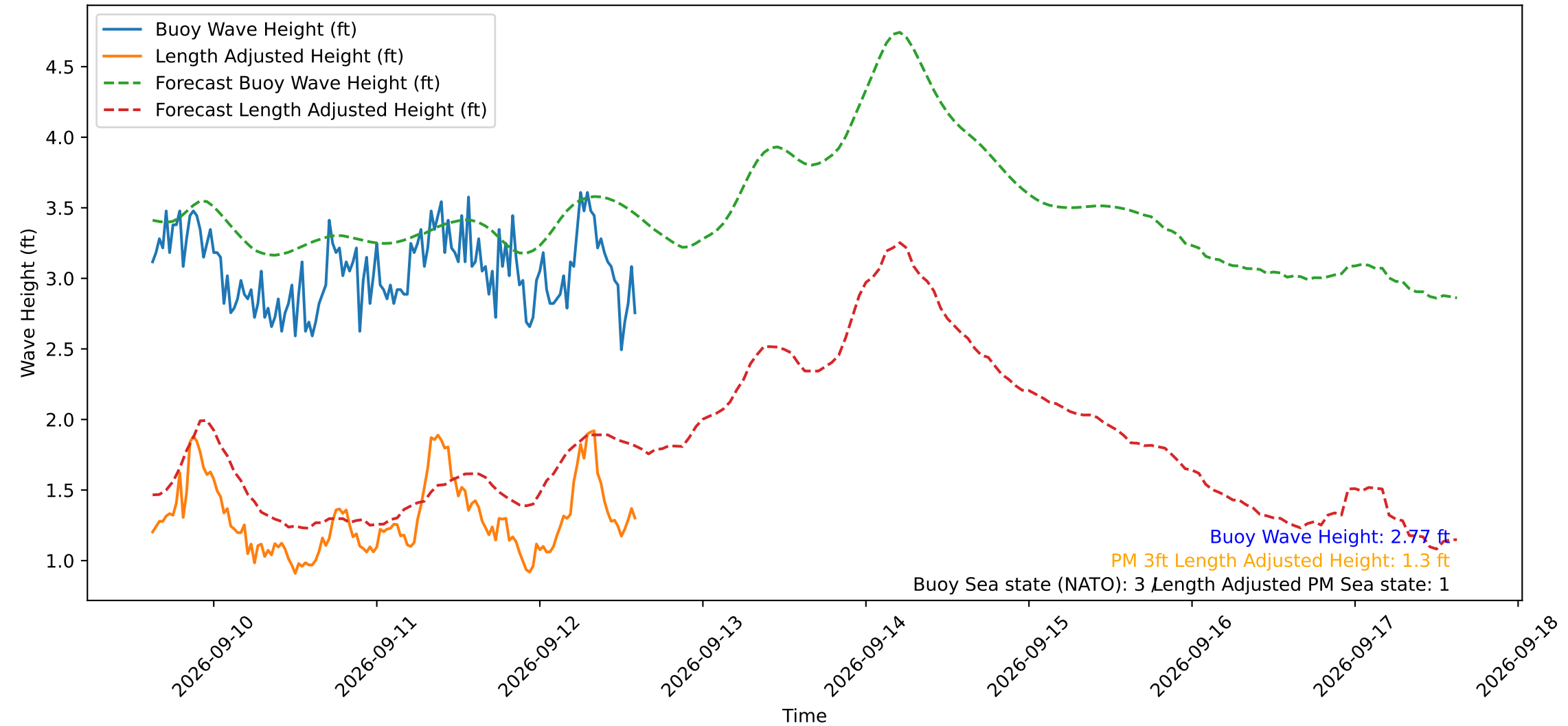
Wave Heights over Time for Green Beach at 2026-09-12 14:51:14
