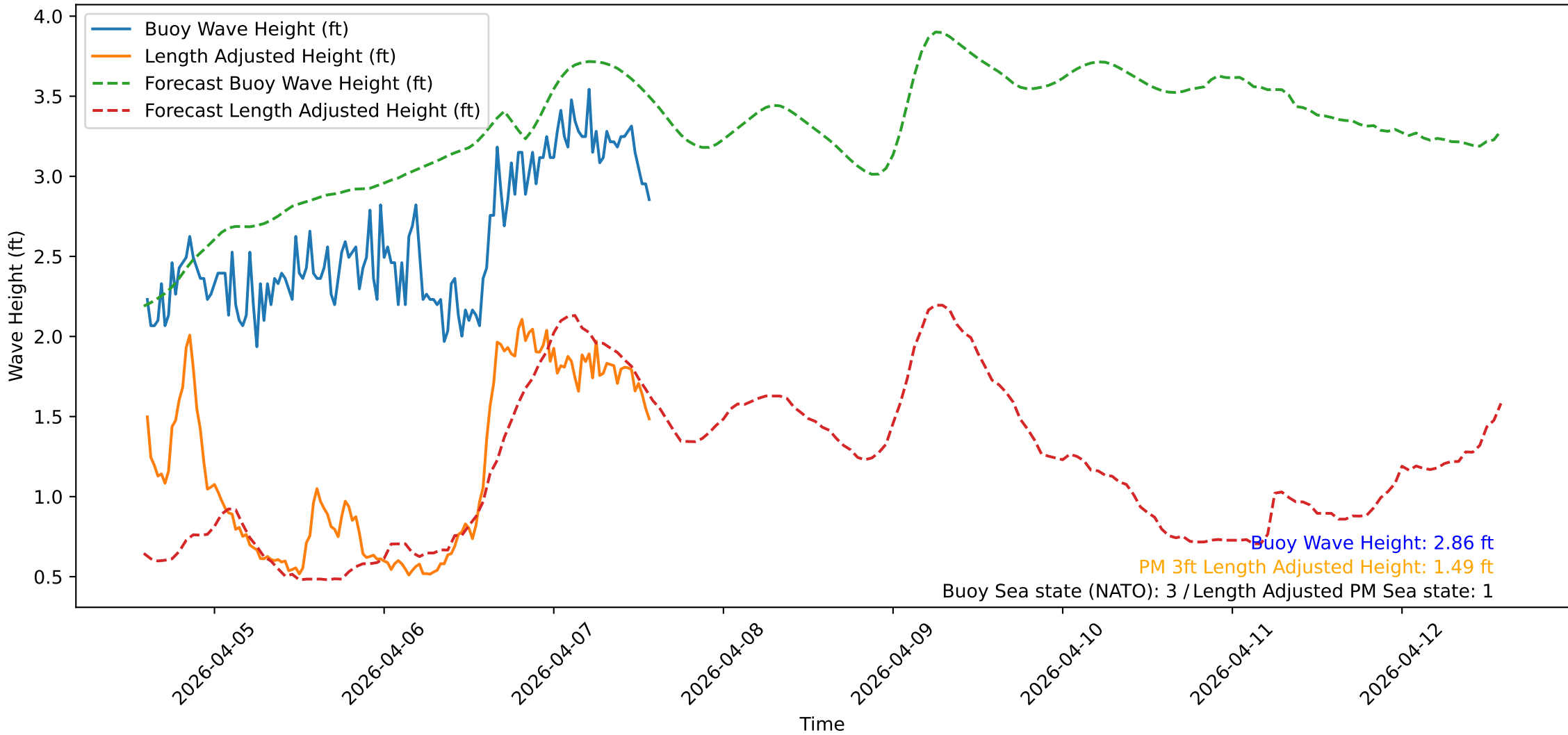
Wave Heights over Time for Red Beach at 2026-04-07 14:20:48
