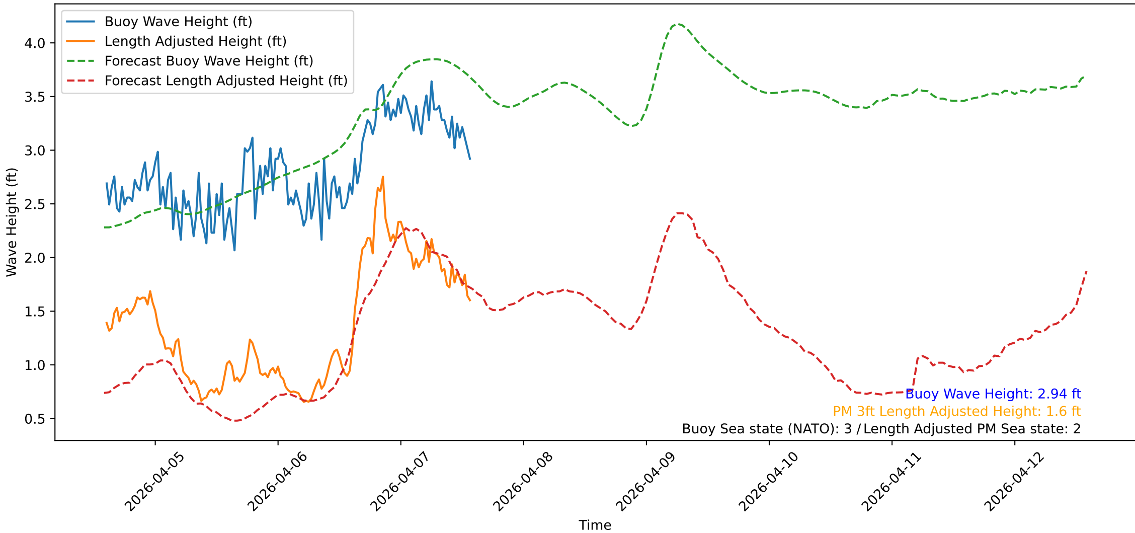
Wave Heights over Time for Oceanside Harbor at 2026-04-07 14:20:31
