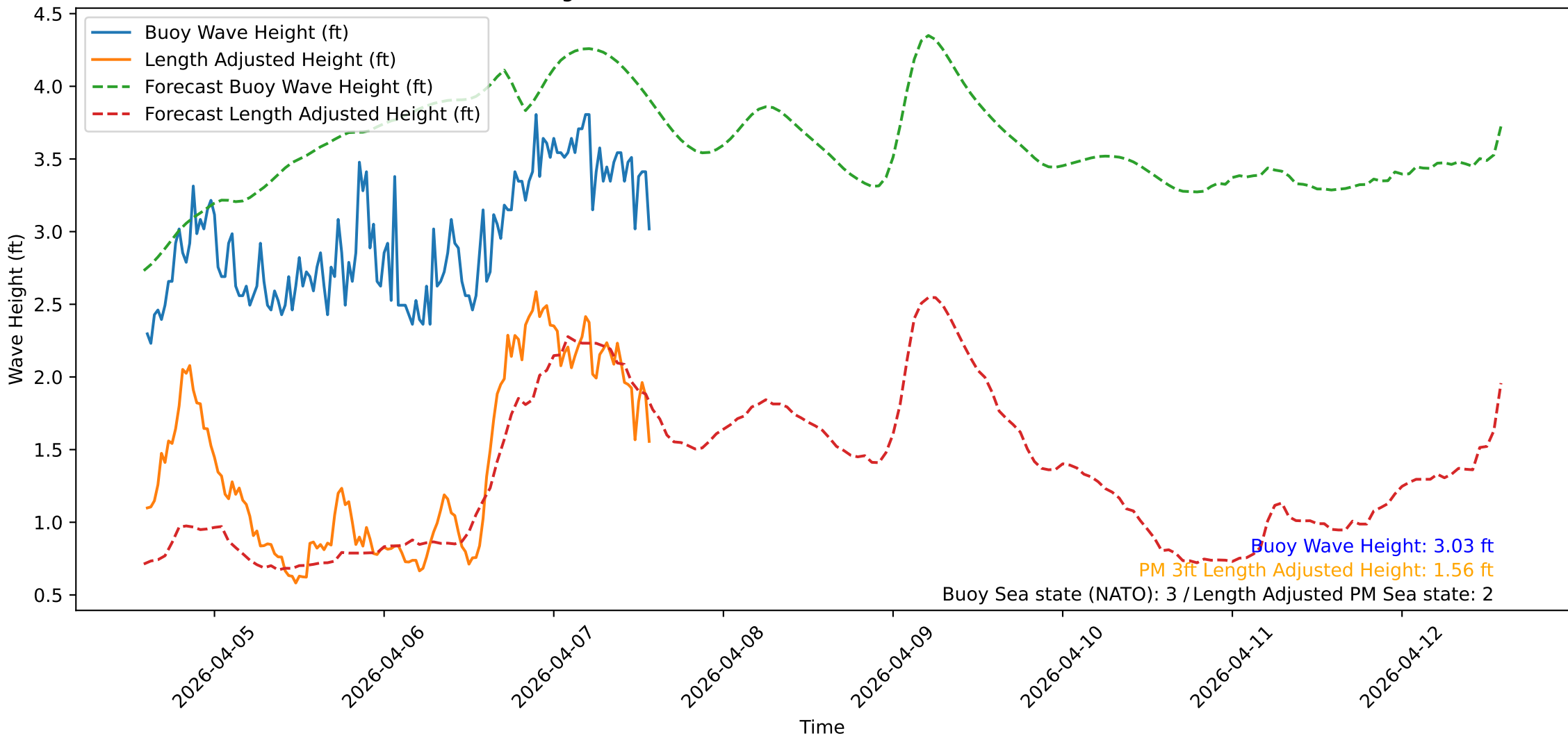
Wave Heights over Time for Green Beach at 2026-04-07 14:21:11
