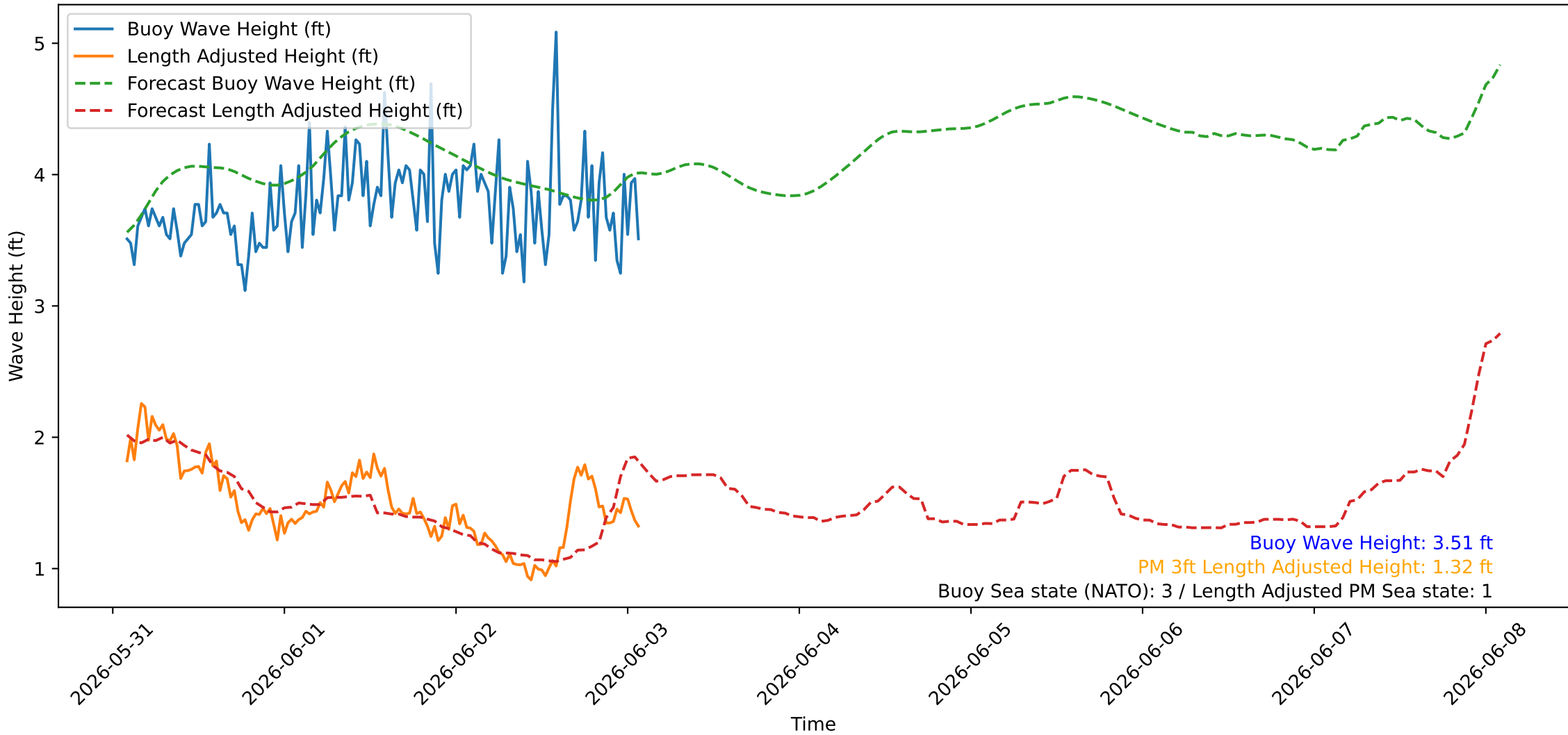
Wave Heights over Time for Oceanside Harbor at 2026-06-03 02:10:25
