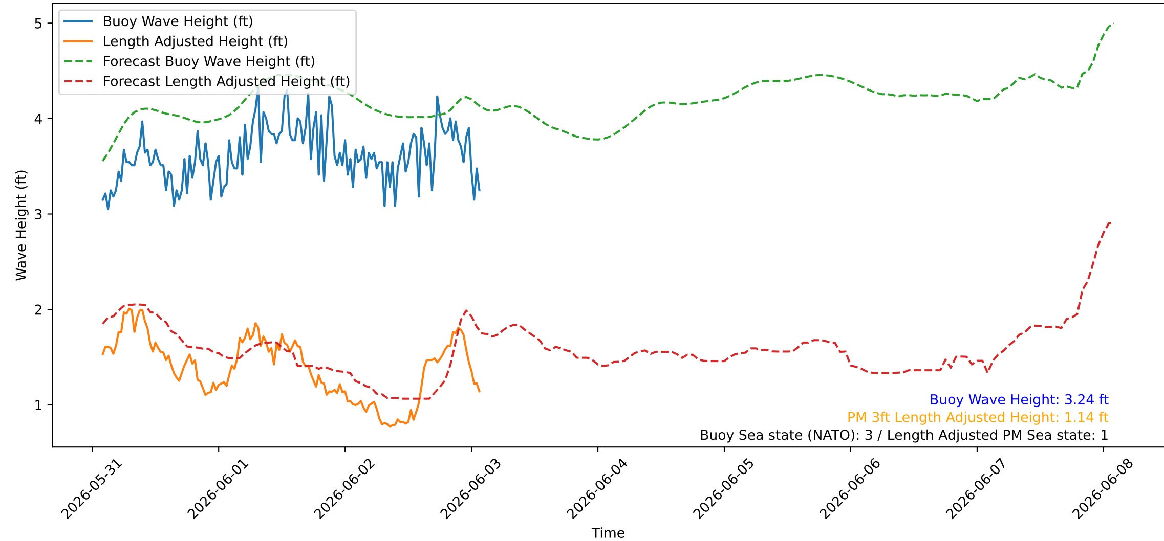
Wave Heights over Time for Green Beach at 2026-06-03 02:11:07
