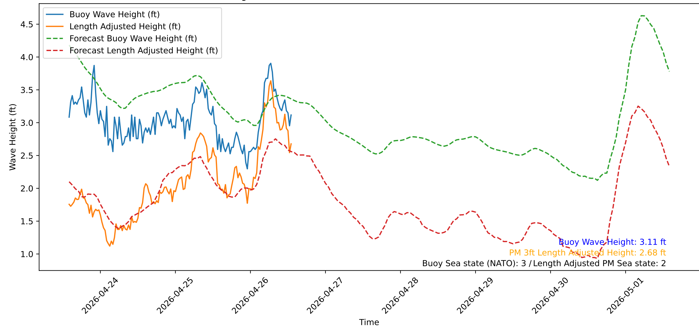
Wave Heights over Time for Oceanside Harbor at 2026-04-26 13:50:31
