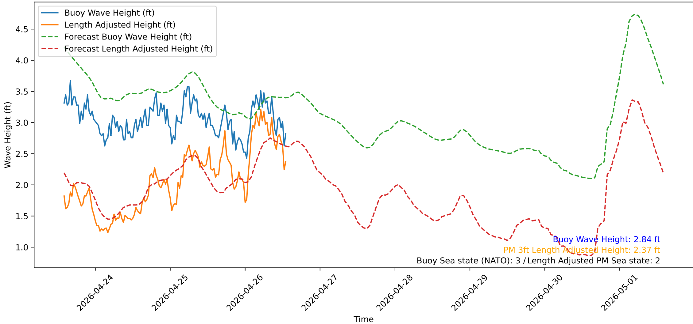
Wave Heights over Time for Green Beach at 2026-04-26 13:51:13
