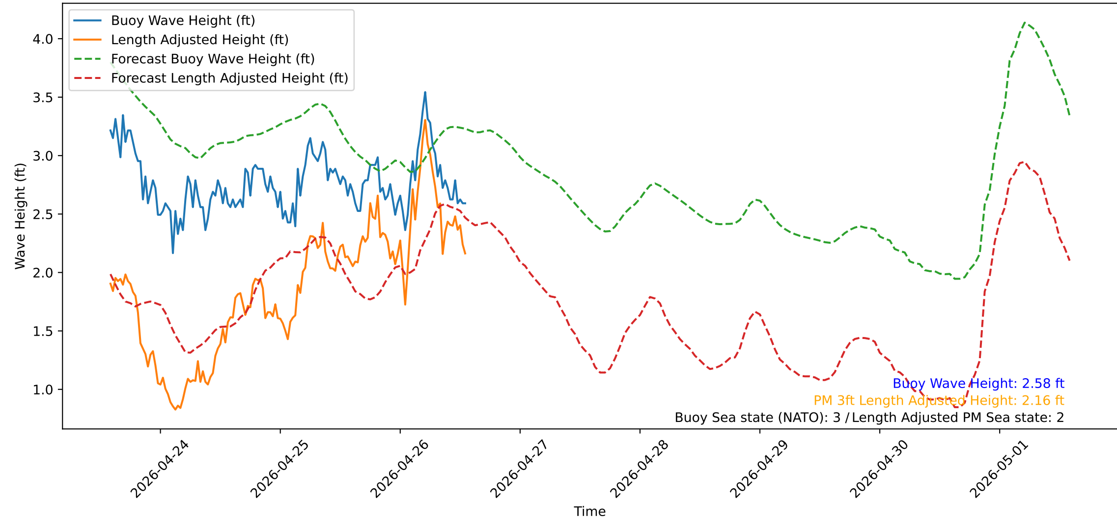
Wave Heights over Time for Red Beach at 2026-04-26 13:50:51
