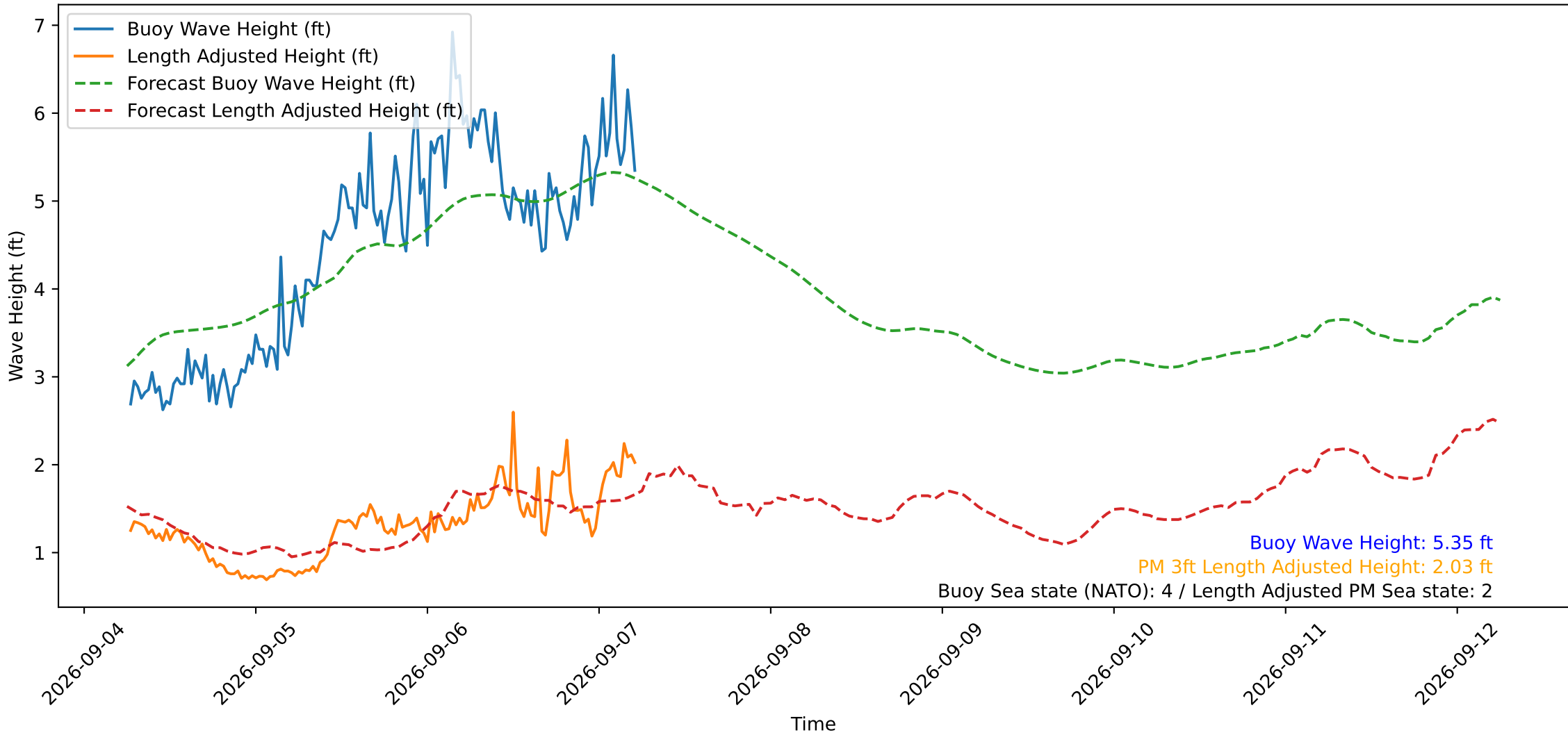
Wave Heights over Time for Red Beach at 2026-09-07 06:00:49
