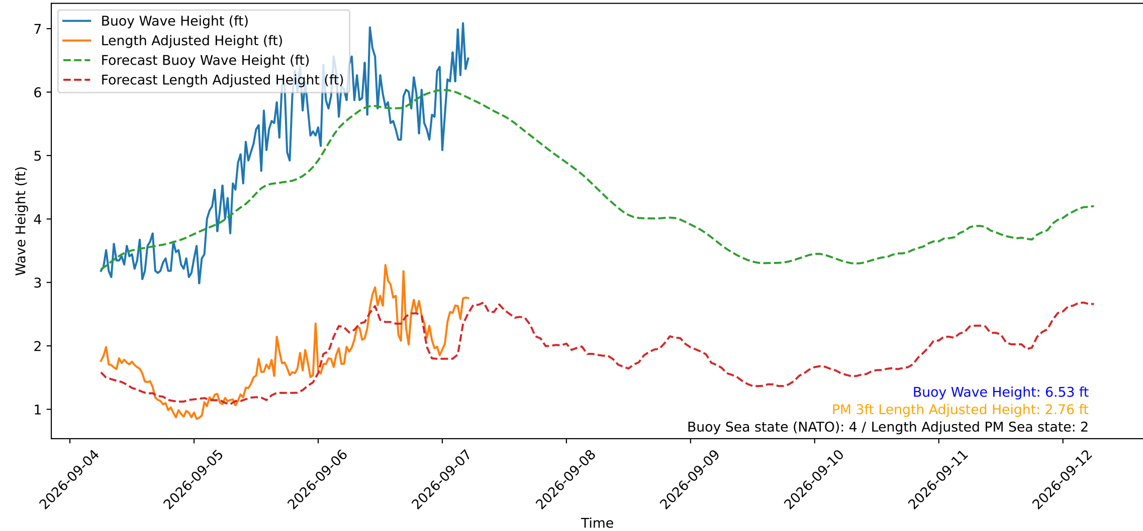
Wave Heights over Time for Oceanside Harbor at 2026-09-07 06:00:29
