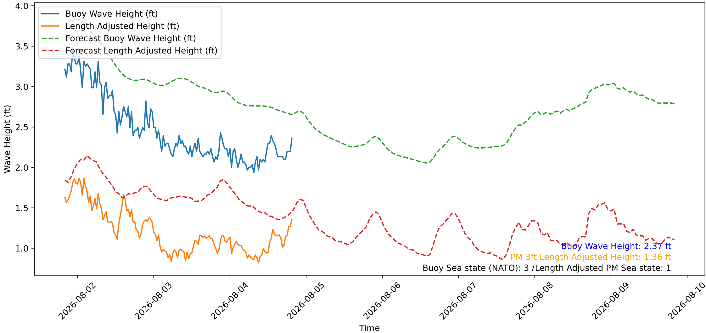
Wave Heights over Time for Green Beach at 2026-08-04 20:11:09
