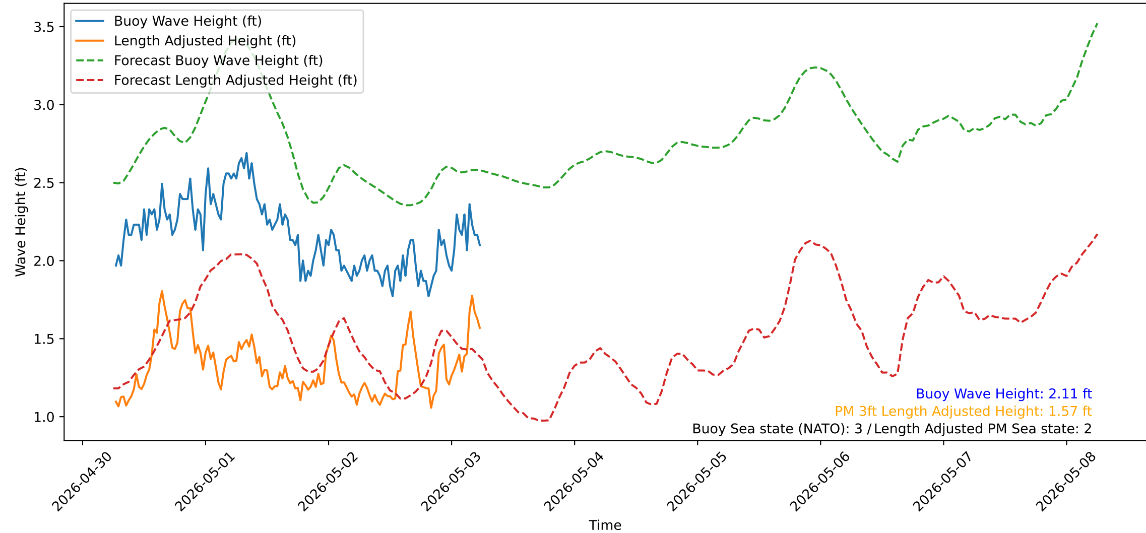
Wave Heights over Time for Oceanside Harbor at 2026-05-03 06:20:31
