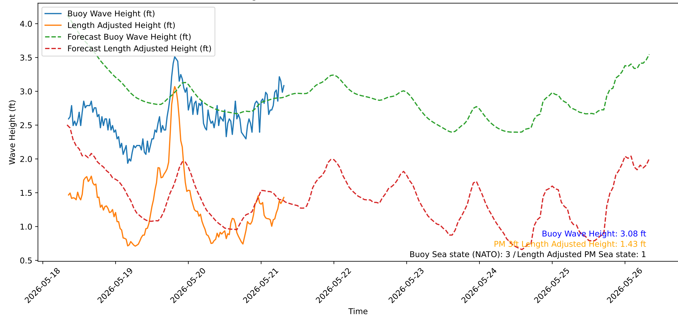
Wave Heights over Time for Red Beach at 2026-05-21 08:10:51
