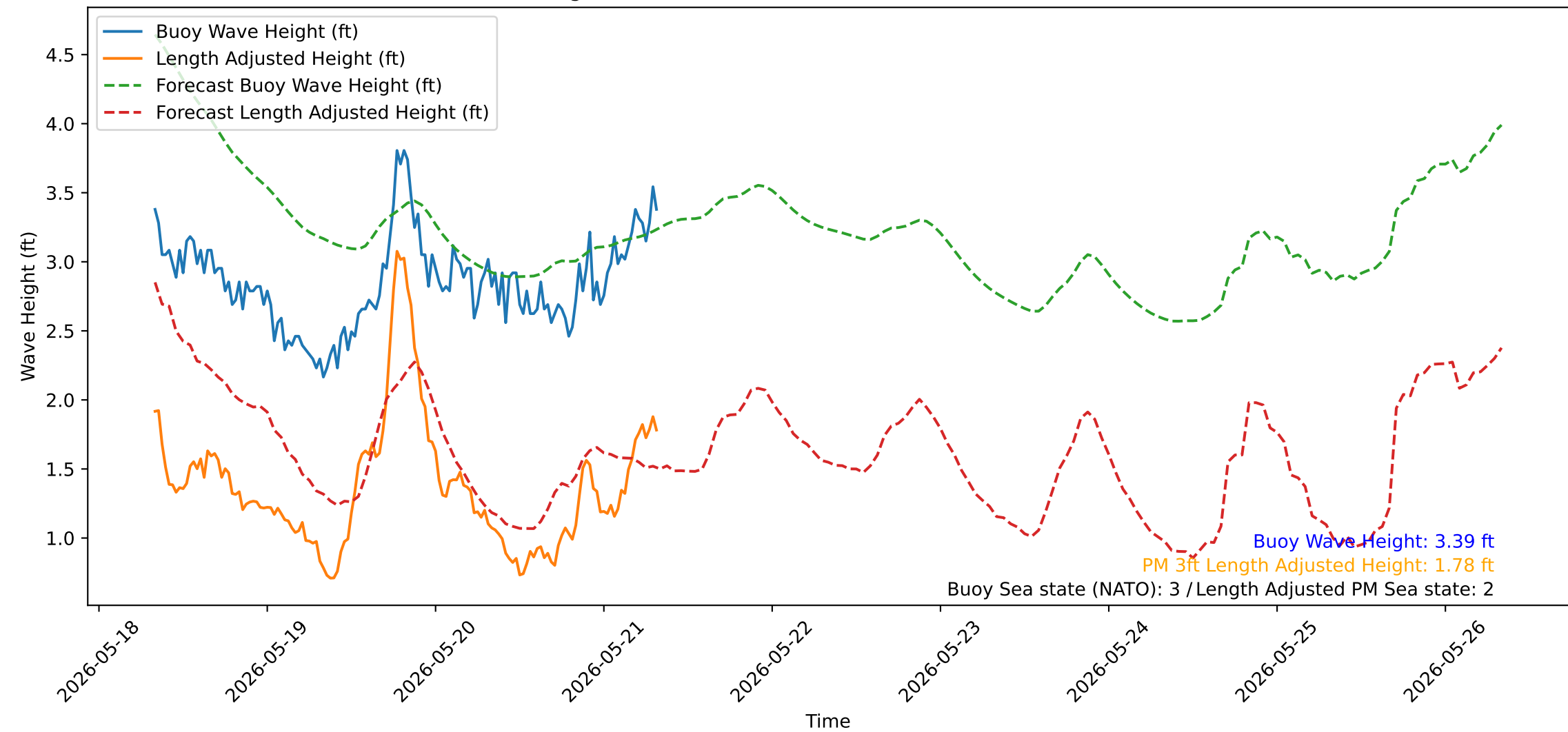
Wave Heights over Time for Green Beach at 2026-05-21 08:11:14
