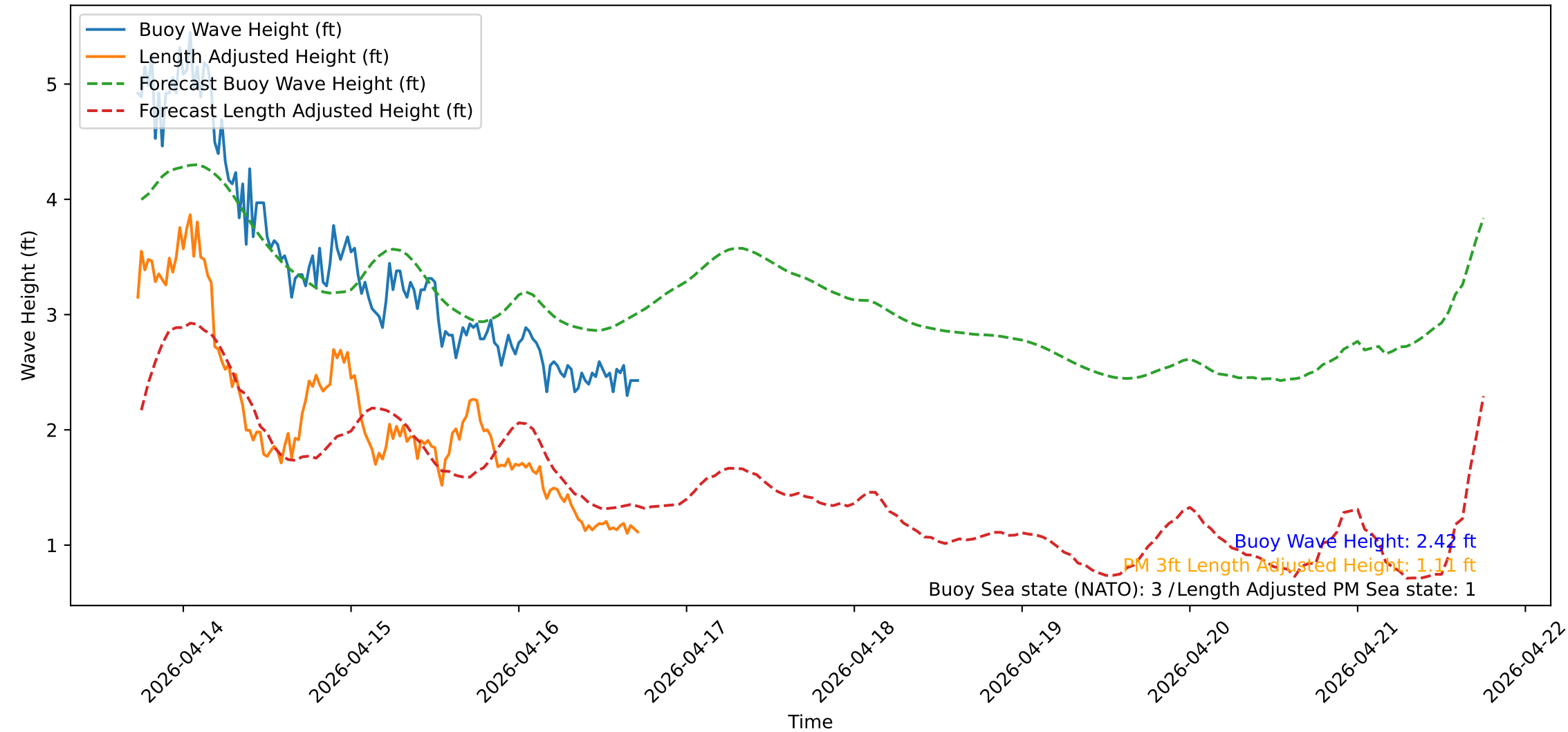
Wave Heights over Time for Oceanside Harbor at 2026-04-16 17:40:32
