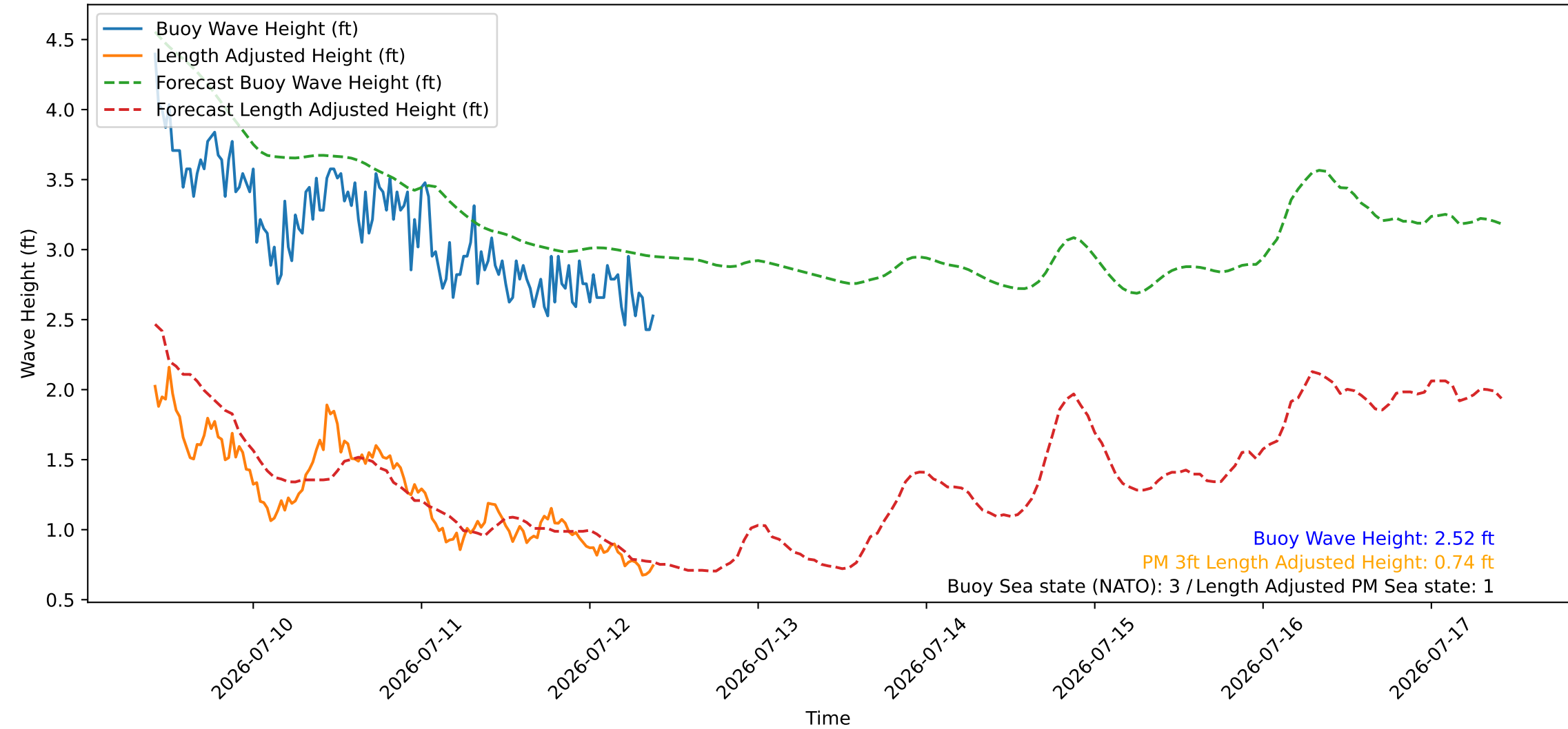
Wave Heights over Time for Green Beach at 2026-07-12 09:51:09
