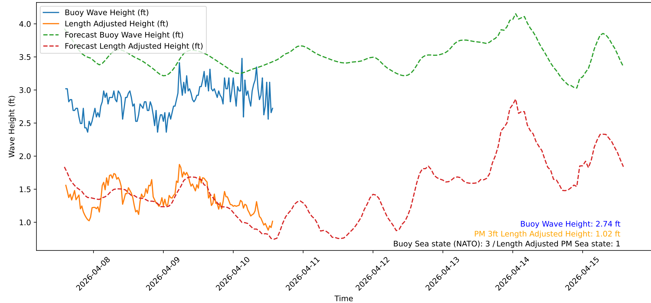
Wave Heights over Time for Green Beach at 2026-04-10 14:21:14
