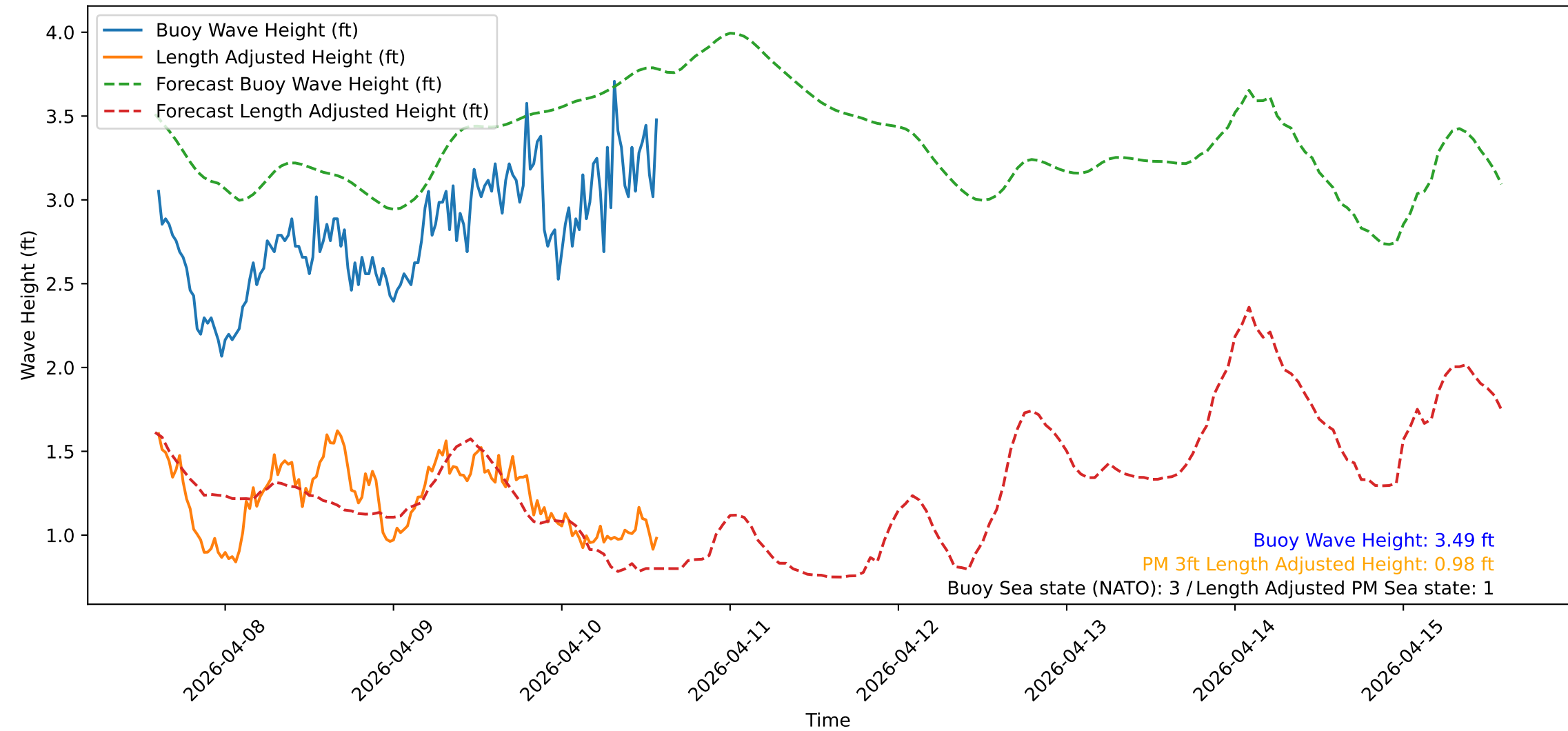
Wave Heights over Time for Red Beach at 2026-04-10 14:20:51
