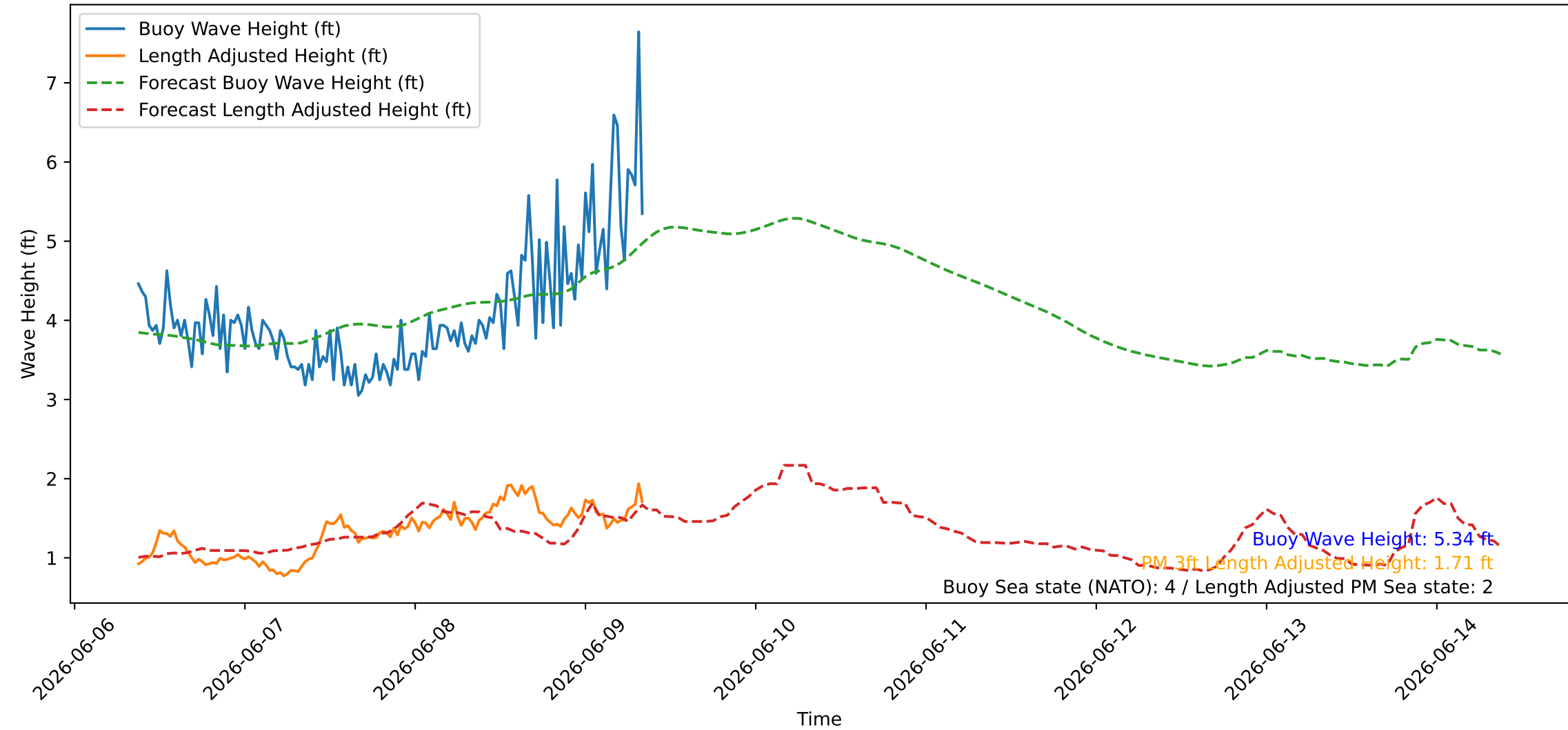
Wave Heights over Time for Red Beach at 2026-06-09 08:50:47
