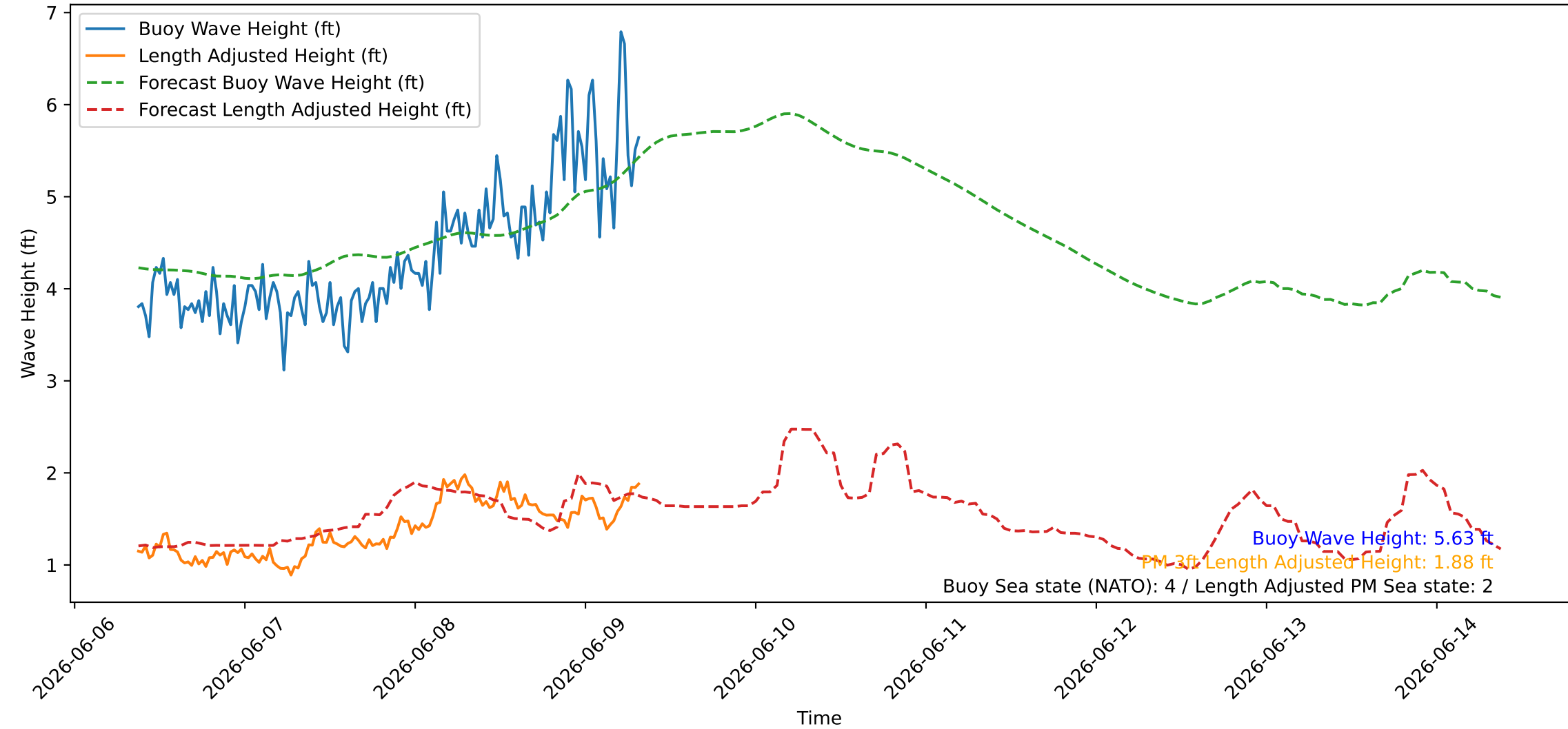
Wave Heights over Time for Green Beach at 2026-06-09 08:51:11
