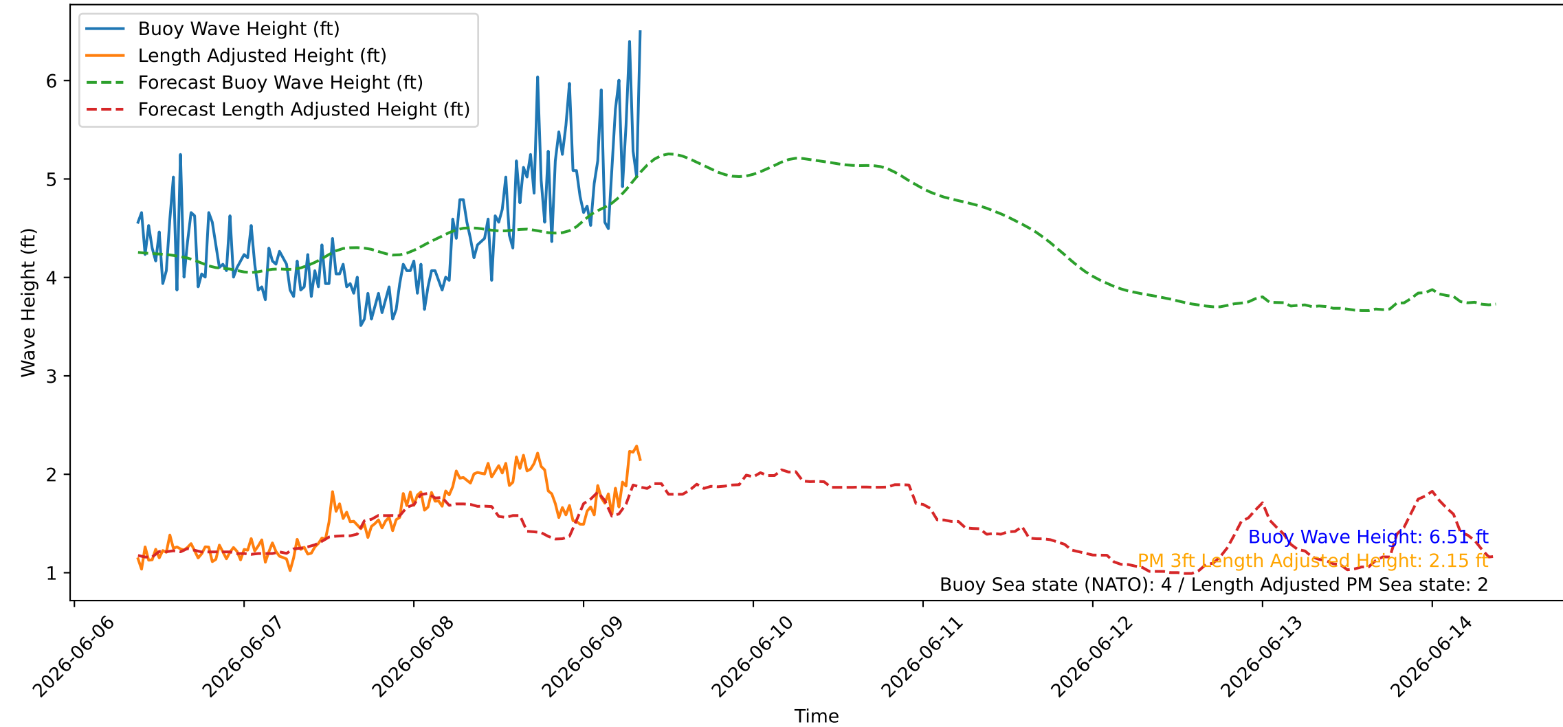
Wave Heights over Time for Oceanside Harbor at 2026-06-09 08:50:26
