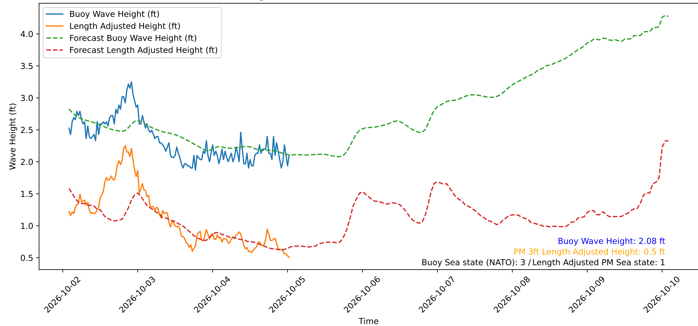
Wave Heights over Time for Red Beach at 2026-10-05 01:30:50
