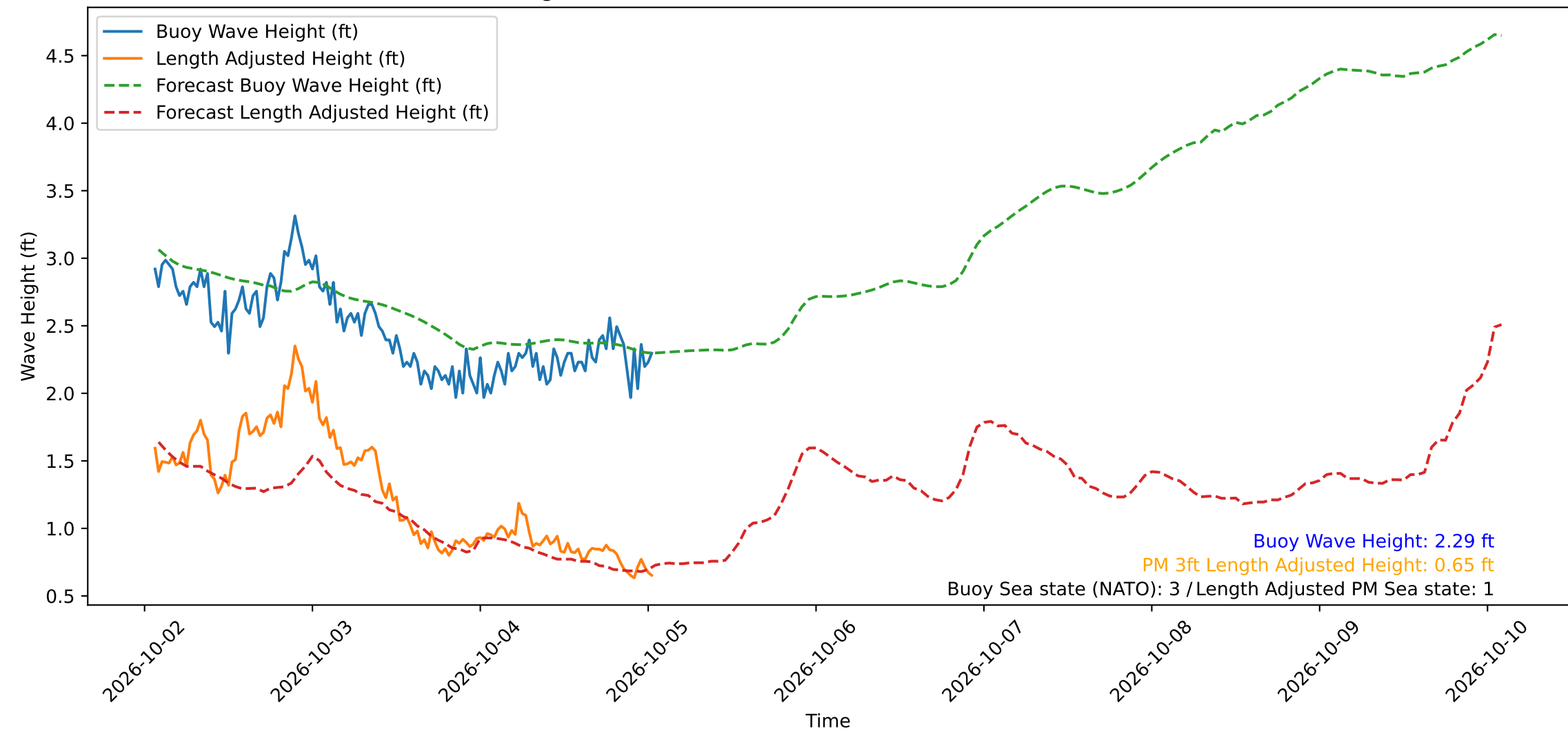
Wave Heights over Time for Oceanside Harbor at 2026-10-05 01:30:30
