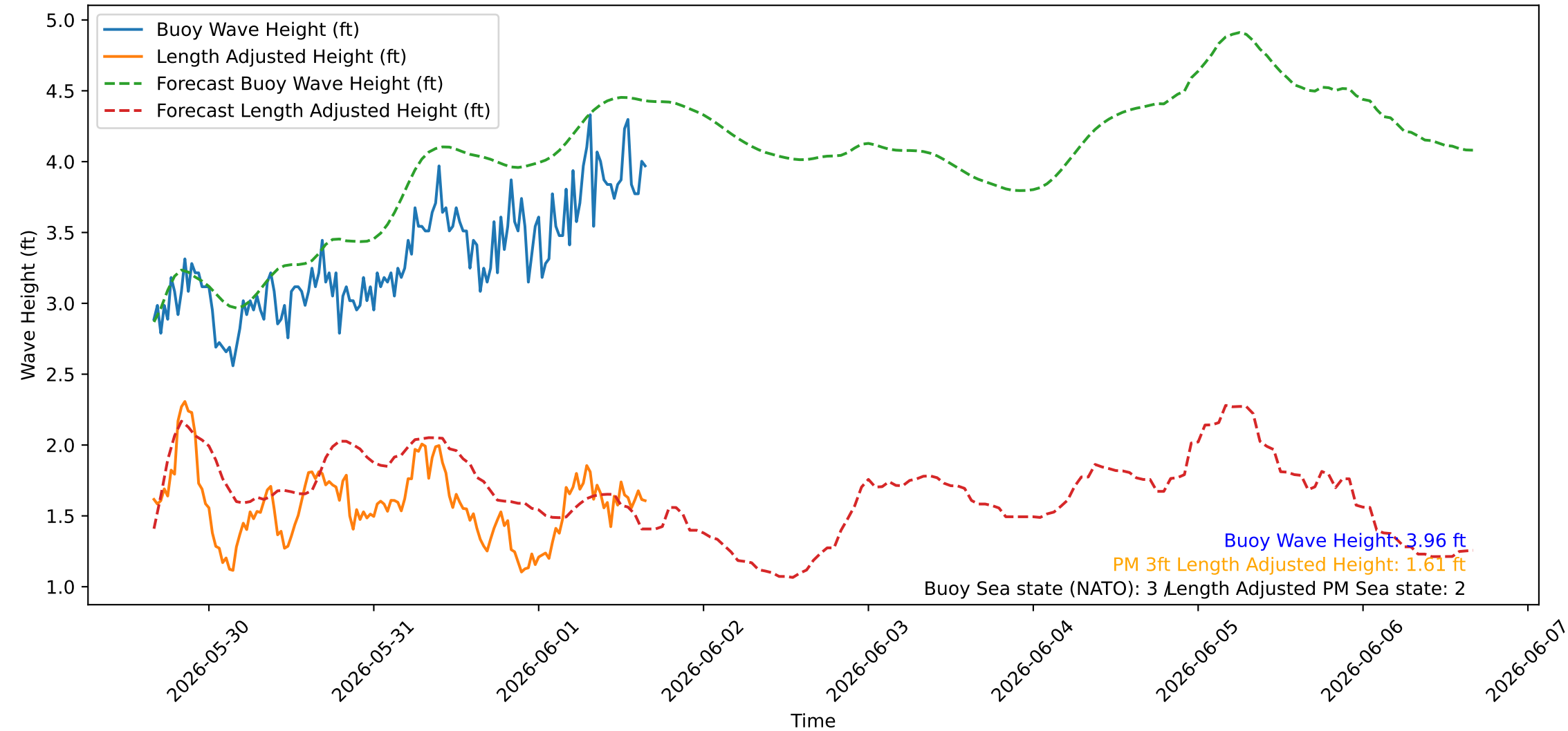
Wave Heights over Time for Green Beach at 2026-06-01 16:11:06
