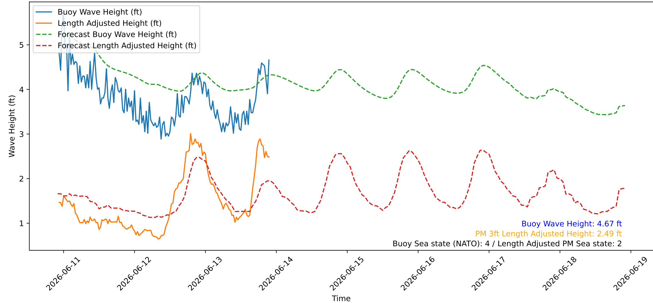
Wave Heights over Time for Green Beach at 2026-06-13 22:21:10
