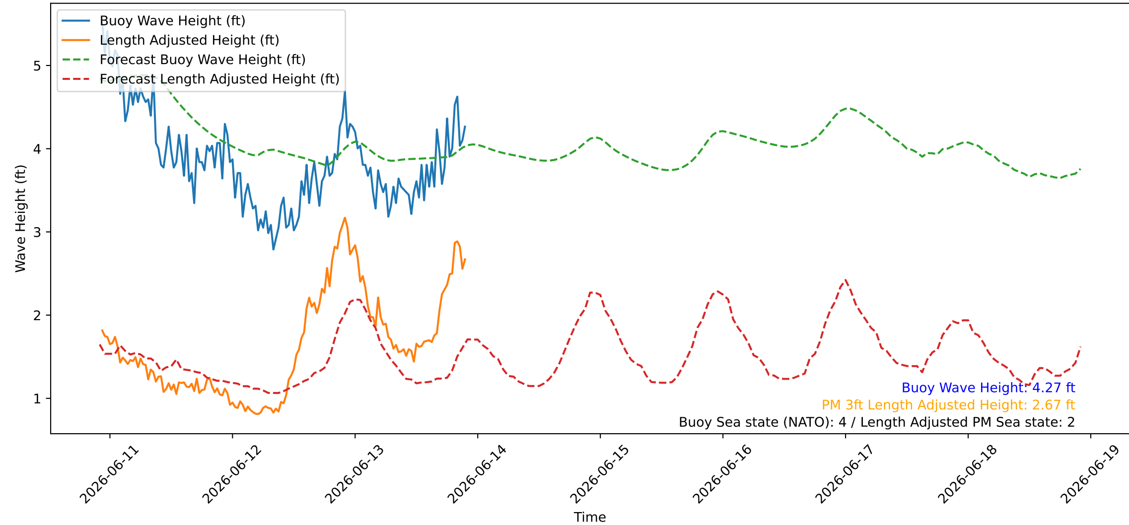
Wave Heights over Time for Oceanside Harbor at 2026-06-13 22:20:26
