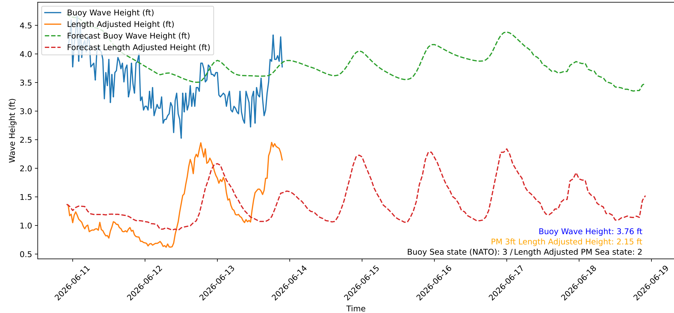
Wave Heights over Time for Red Beach at 2026-06-13 22:20:47
