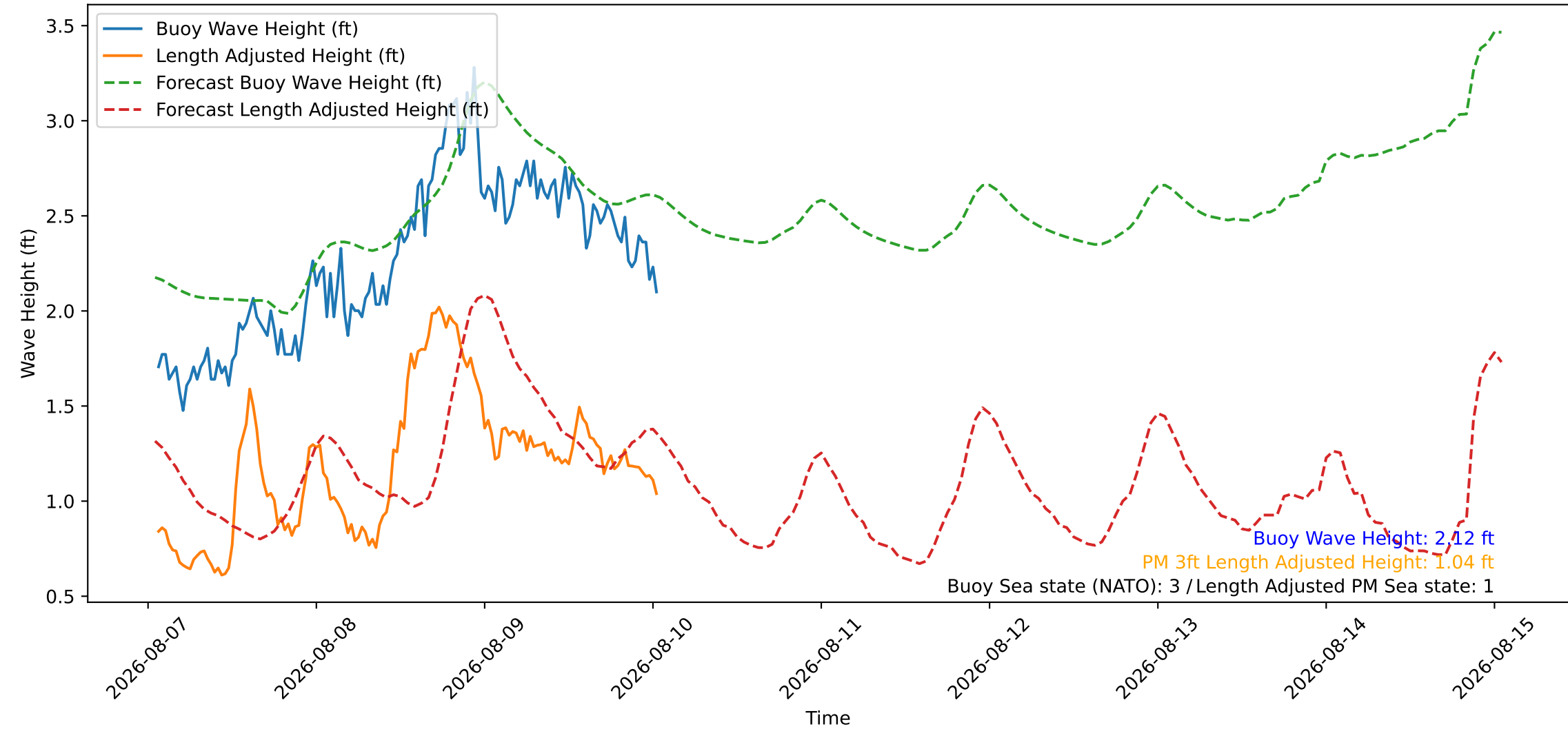
Wave Heights over Time for Red Beach at 2026-08-10 01:20:48
