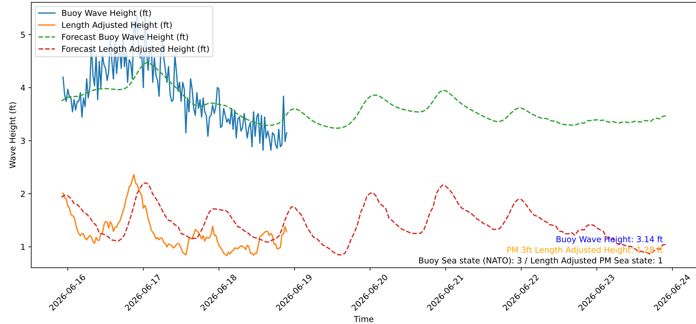
Wave Heights over Time for Red Beach at 2026-06-18 22:20:46
