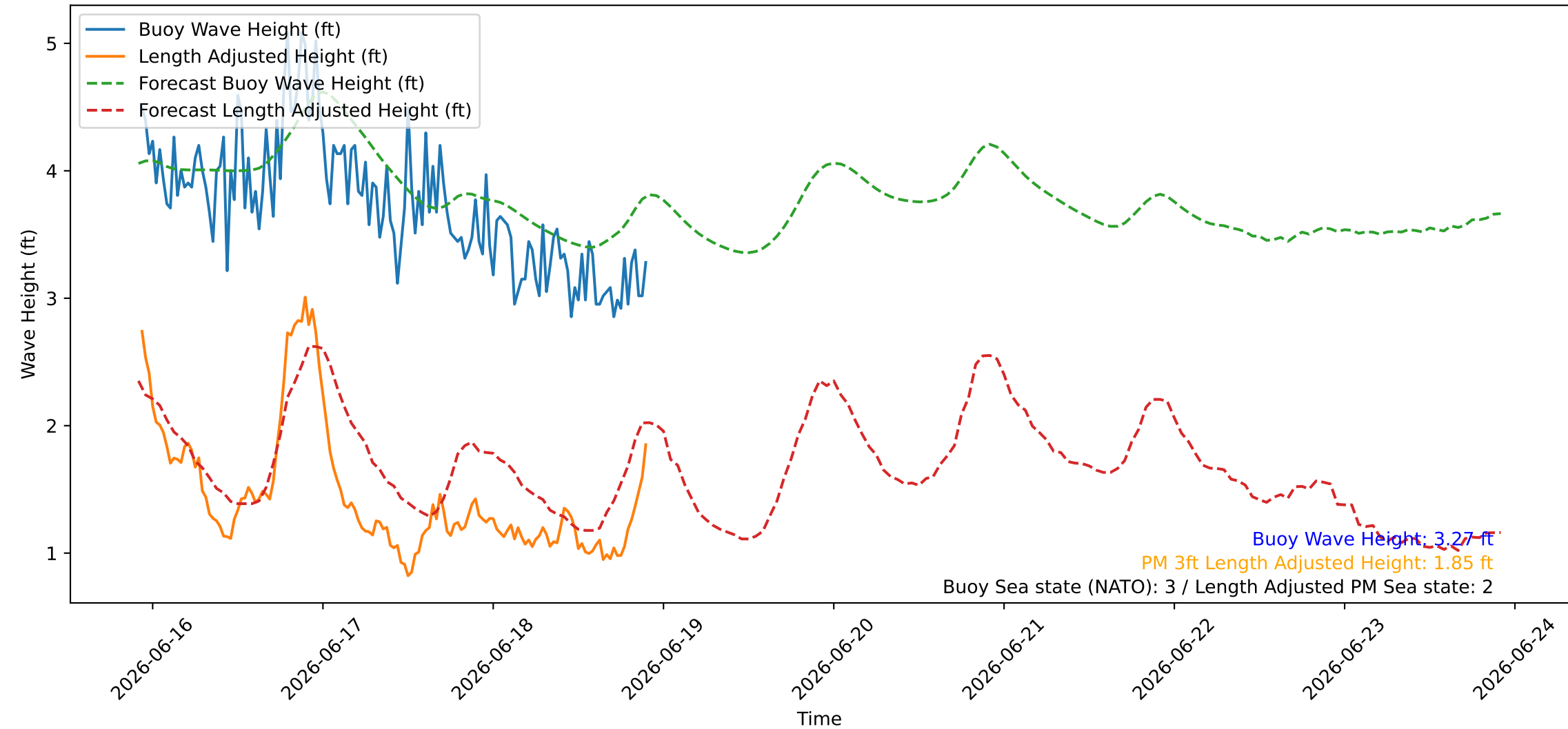
Wave Heights over Time for Green Beach at 2026-06-18 22:21:09
