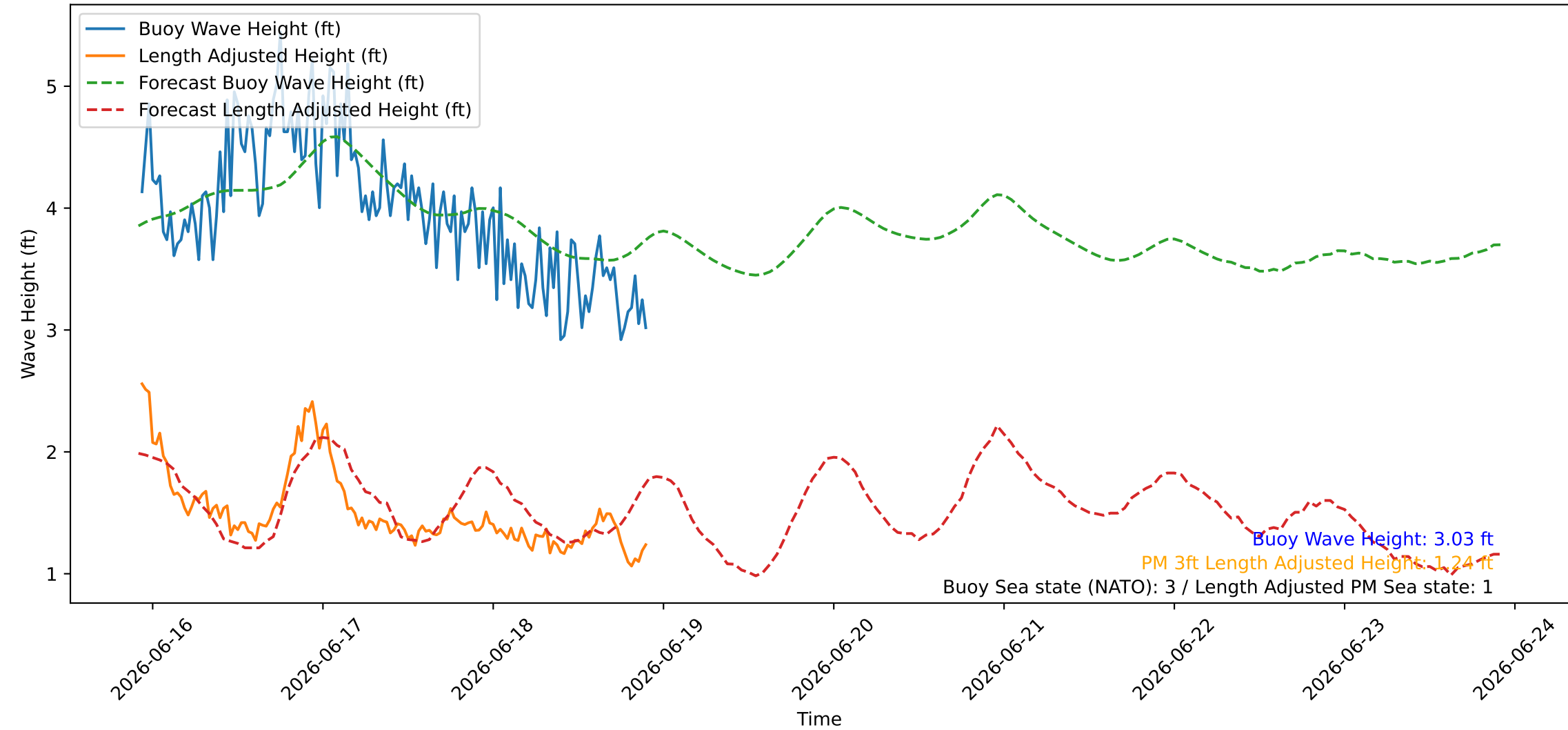
Wave Heights over Time for Oceanside Harbor at 2026-06-18 22:20:25
