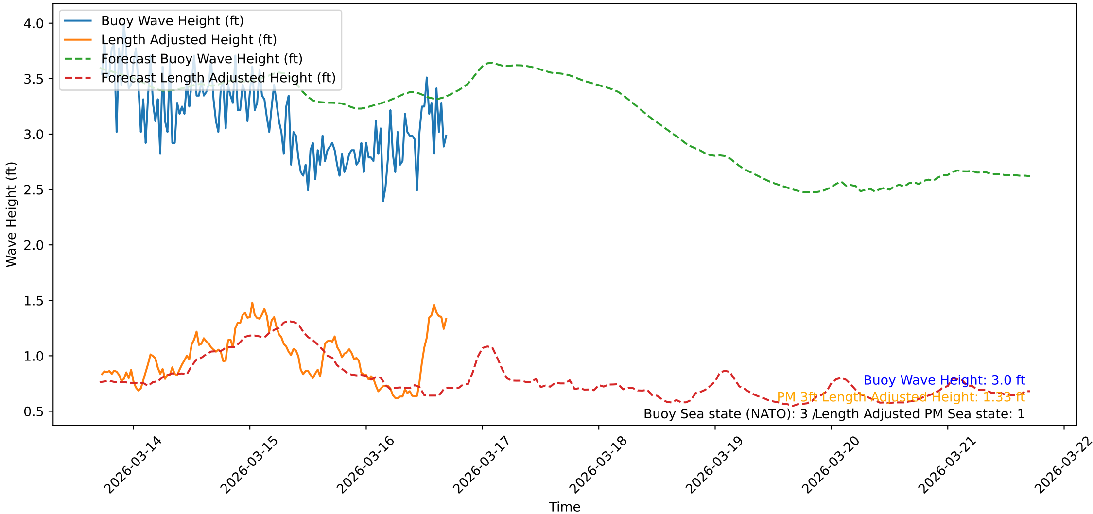
Wave Heights over Time for Oceanside Harbor at 2026-03-16 17:20:42
