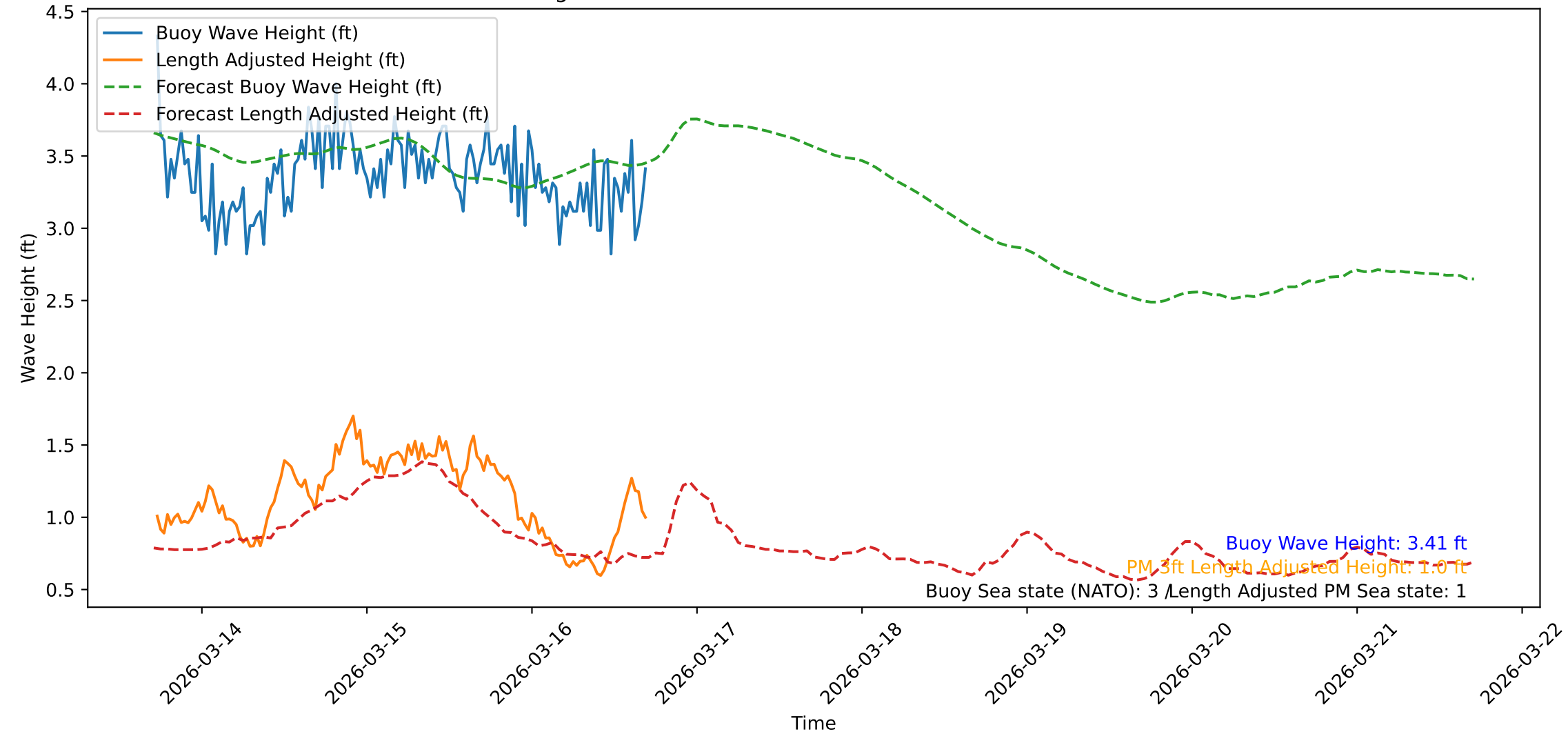
Wave Heights over Time for Green Beach at 2026-03-16 17:21:41
