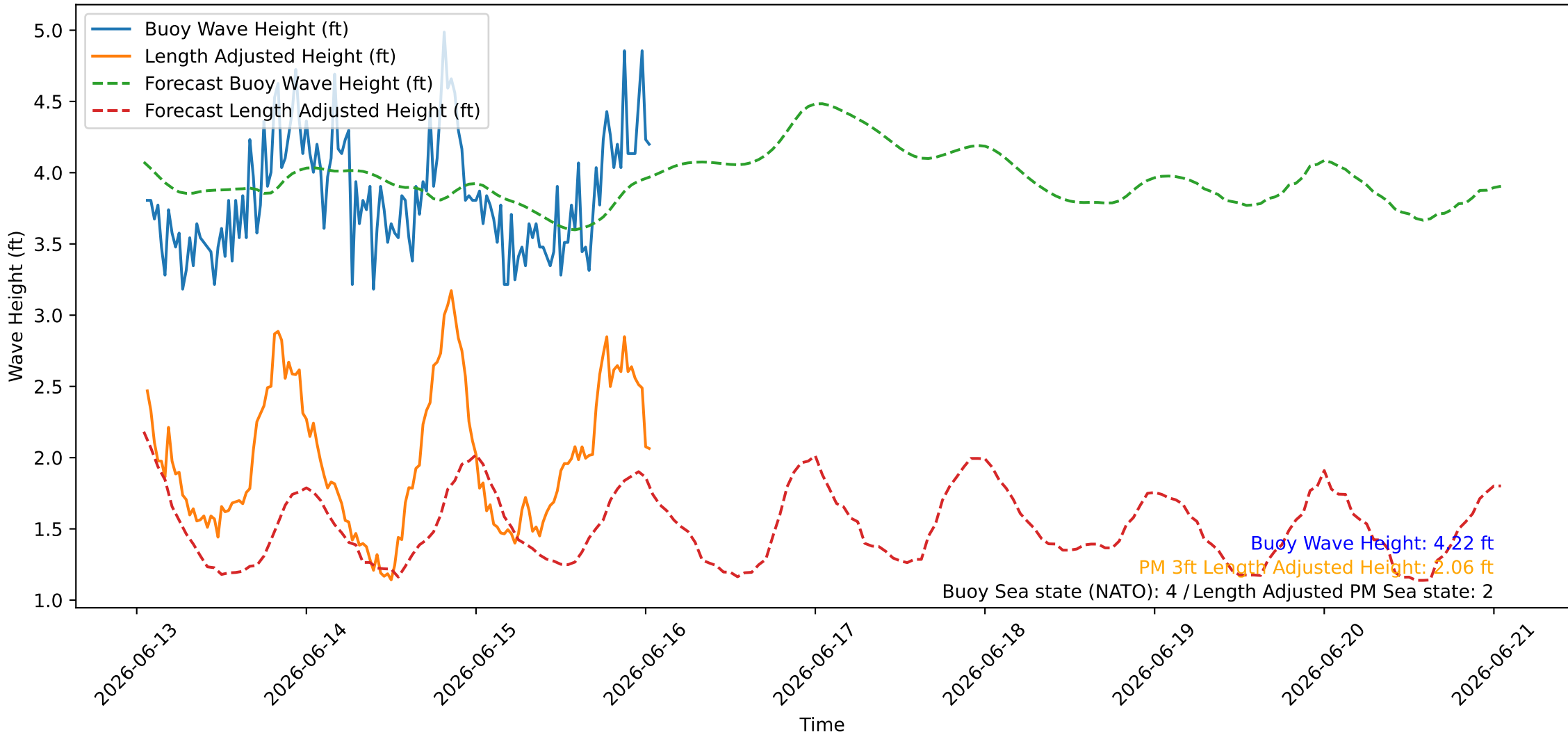
Wave Heights over Time for Oceanside Harbor at 2026-06-16 01:20:26
