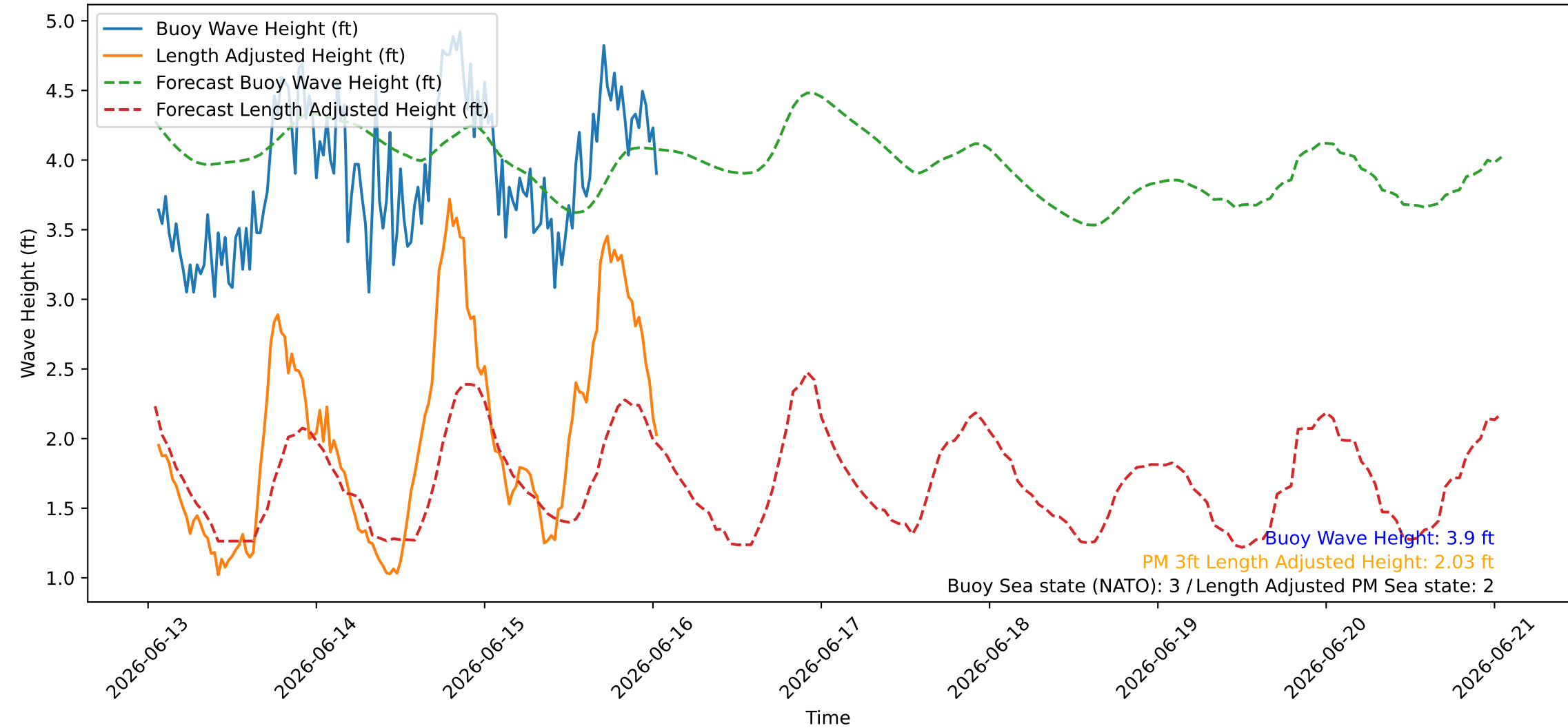
Wave Heights over Time for Green Beach at 2026-06-16 01:21:09
