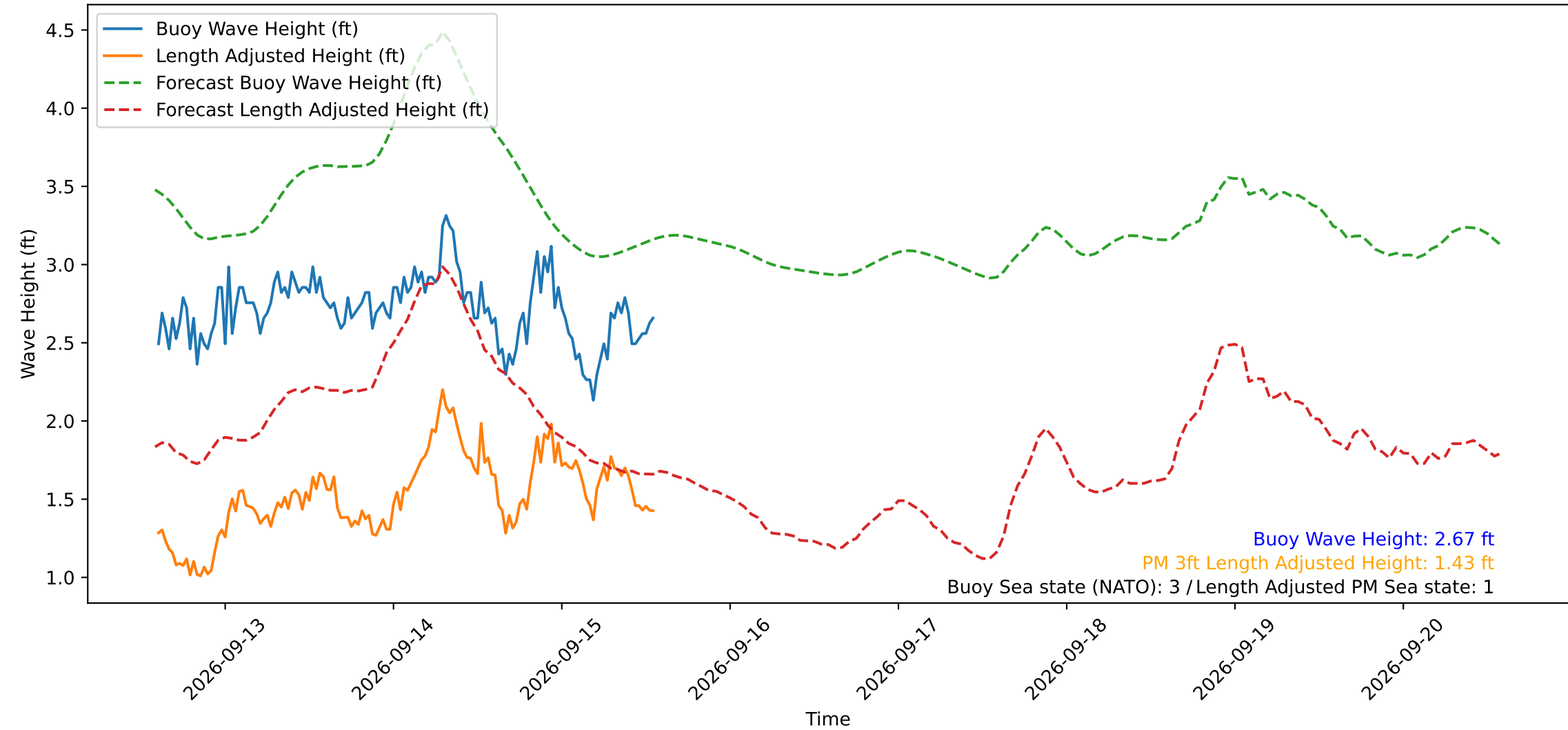
Wave Heights over Time for Green Beach at 2026-09-15 14:01:11
