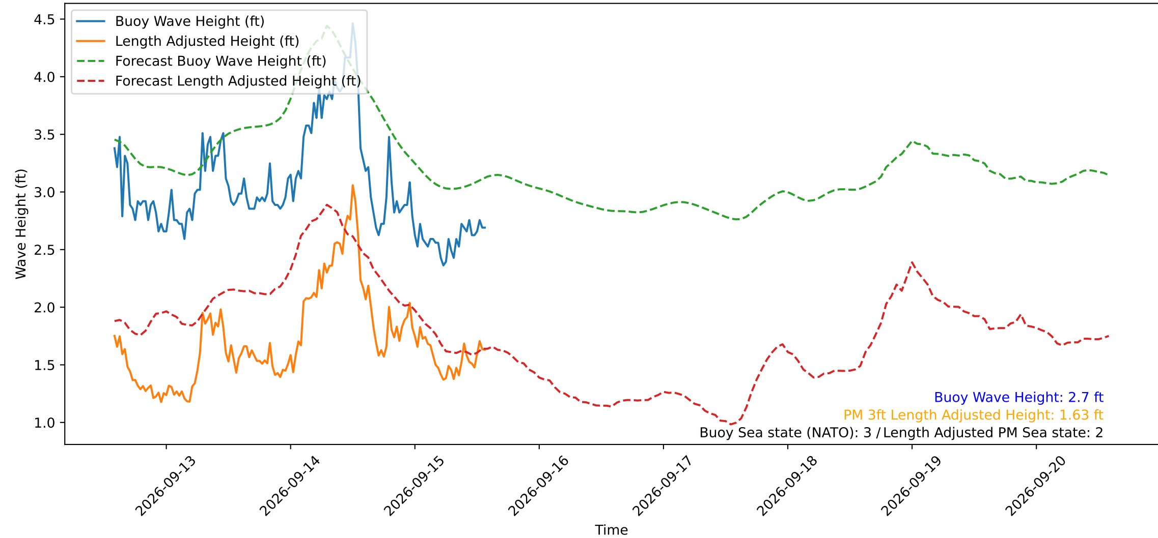
Wave Heights over Time for Oceanside Harbor at 2026-09-15 14:00:29
