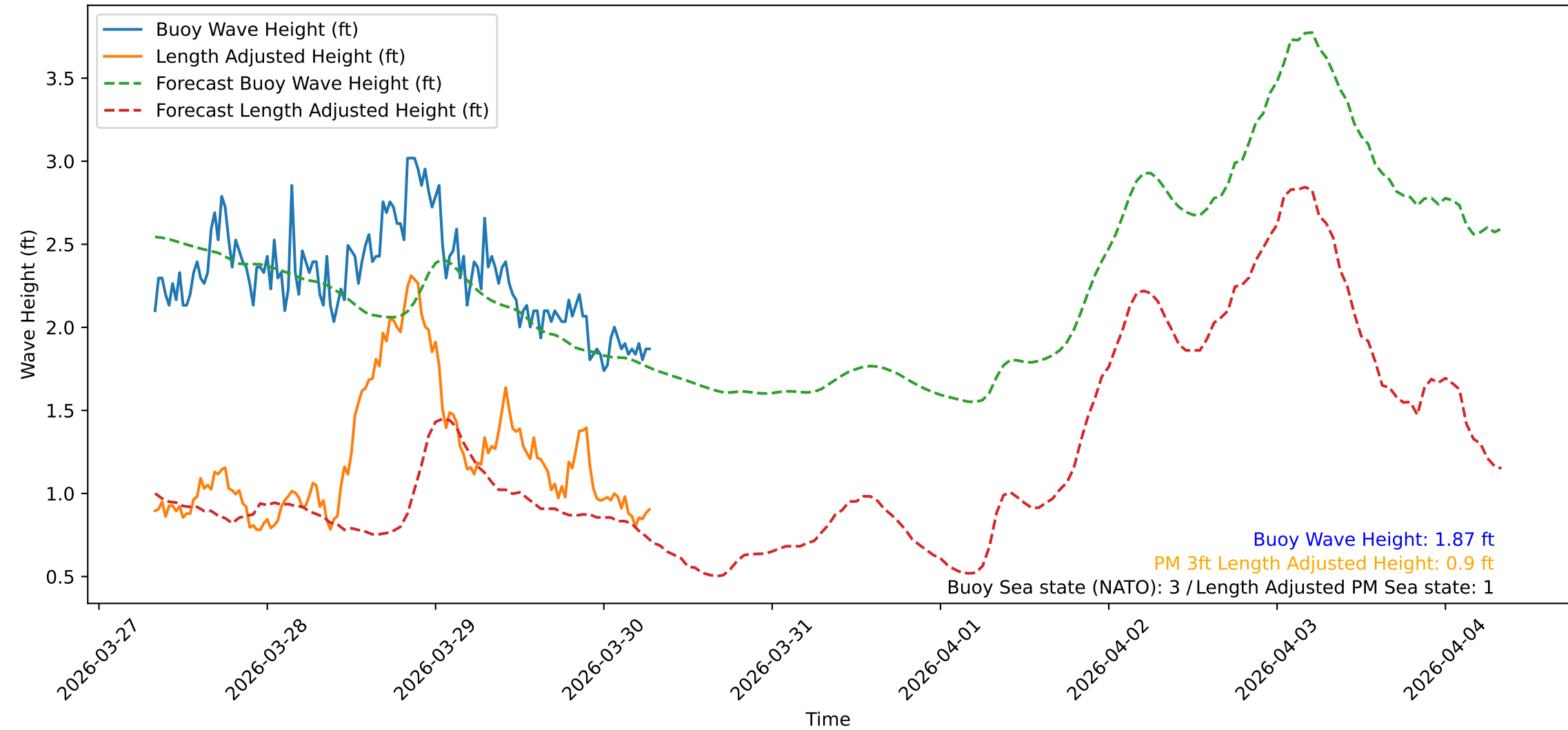
Wave Heights over Time for Red Beach at 2026-03-30 07:30:48
