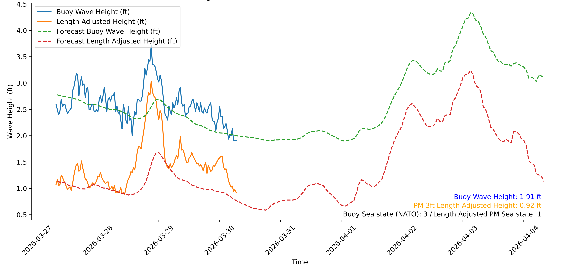
Wave Heights over Time for Green Beach at 2026-03-30 07:31:10
