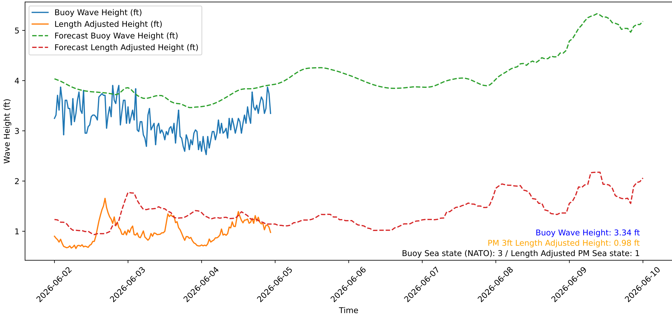
Wave Heights over Time for Red Beach at 2026-06-04 23:30:45
