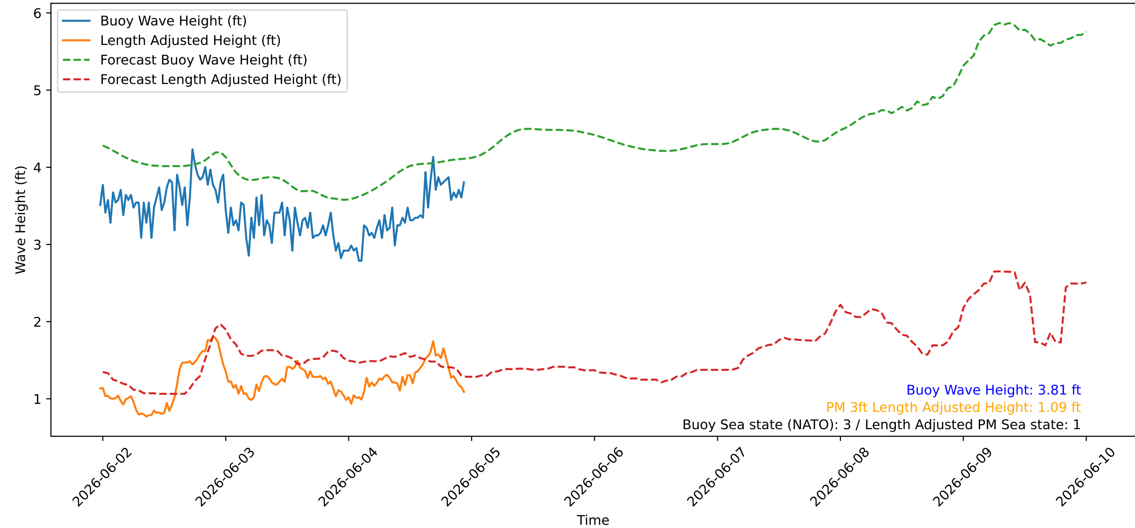
Wave Heights over Time for Green Beach at 2026-06-04 23:31:07
