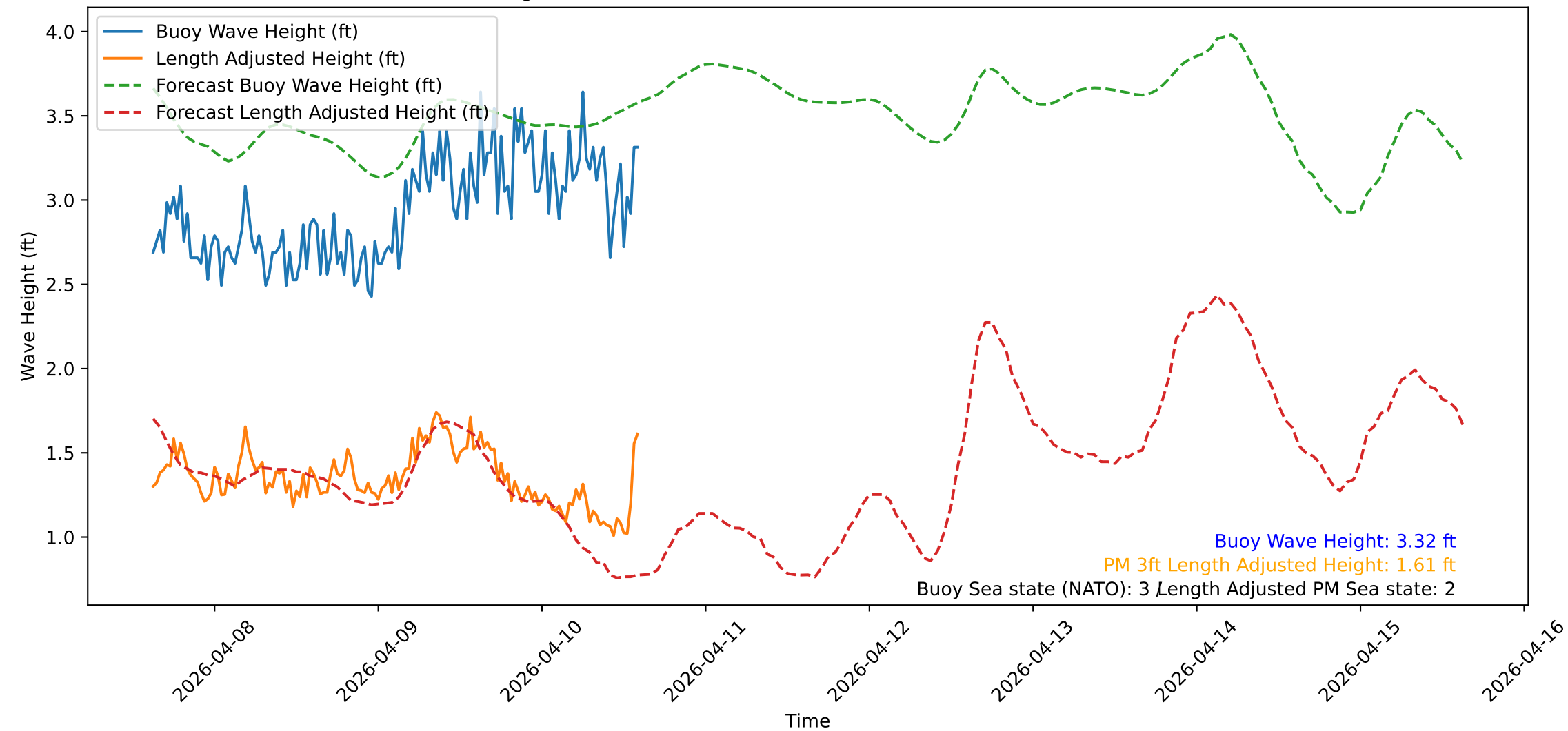
Wave Heights over Time for Oceanside Harbor at 2026-04-10 15:00:31
