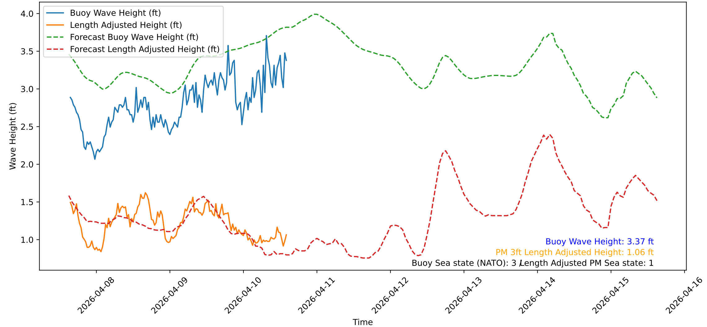
Wave Heights over Time for Red Beach at 2026-04-10 15:00:50
