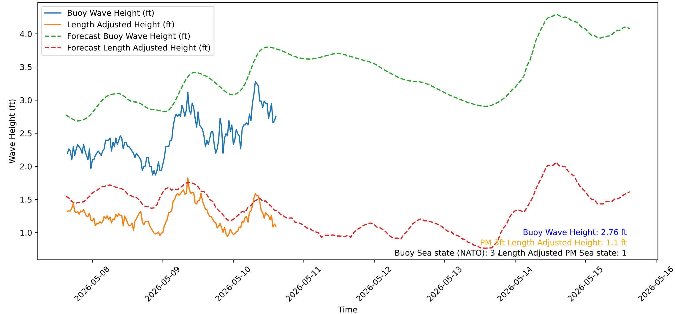
Wave Heights over Time for Oceanside Harbor at 2026-05-10 15:20:31
