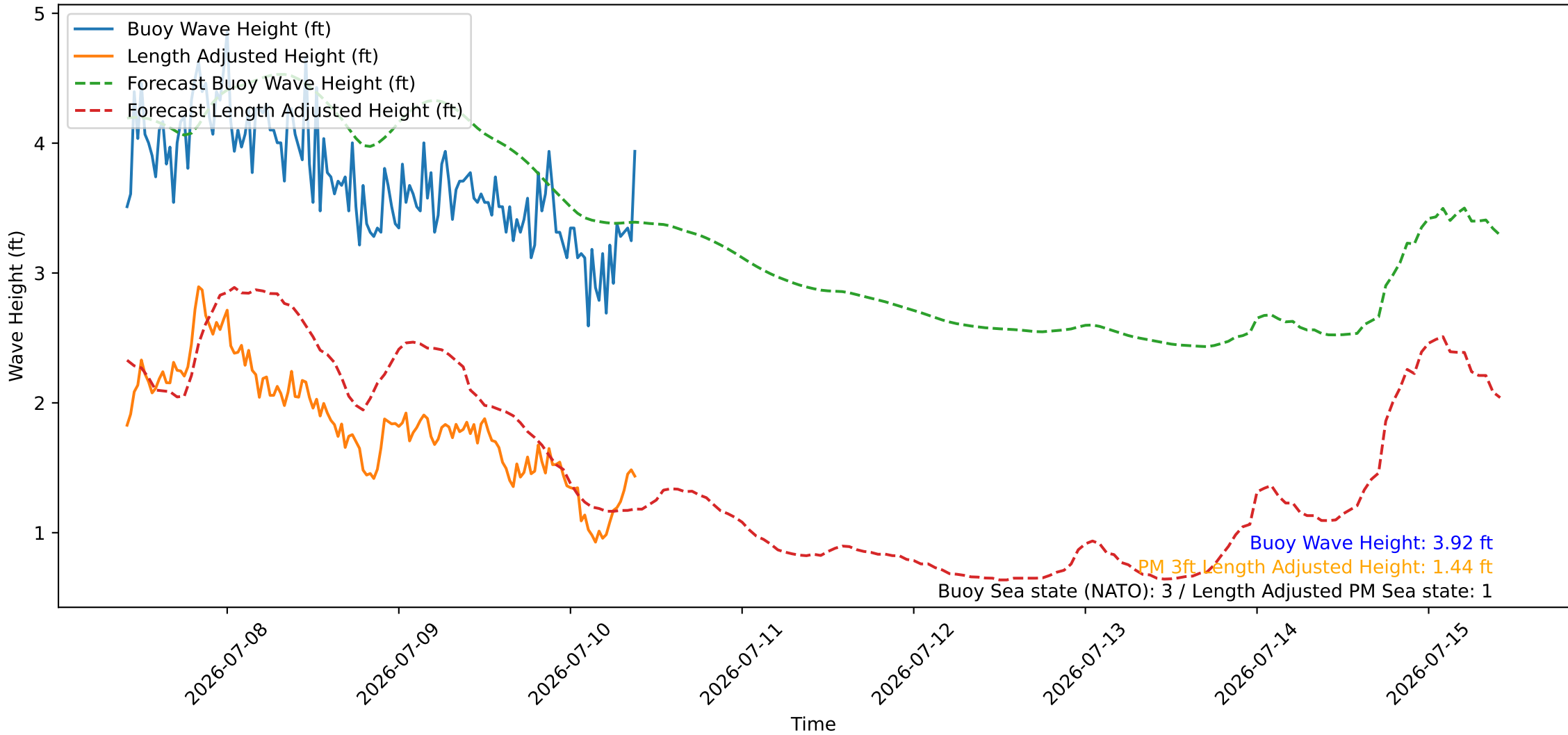
Wave Heights over Time for Red Beach at 2026-07-10 09:50:47
