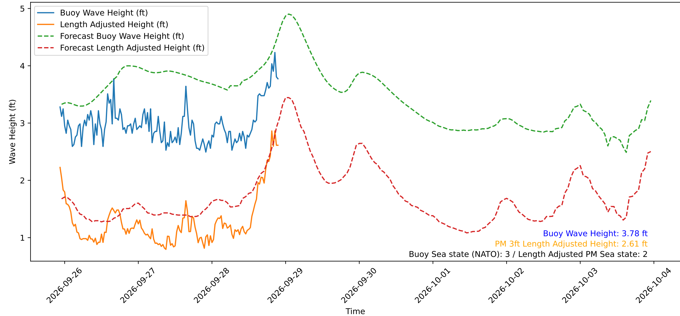
Wave Heights over Time for Oceanside Harbor at 2026-09-28 22:30:30
